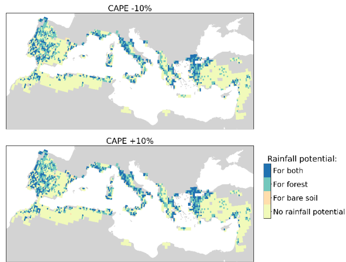
Figure A11: Sensitivity of rainfall potential to a change in the convective available potential energy (CAPE). Top: a change in CAPE of -10%, bottom: a change in CAPE of +10%. This plot indicates for each grid cell if most samples have a rainfall potential over bare soil, forest, both land cover types or no rainfall potential in any of the samples.
