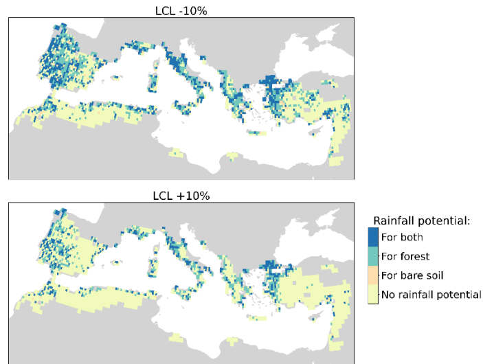
625 Figure A10: Sensitivity of rainfall potential to a change in the lifting condensation level (LCL). Top: a change in LCL of -10%, bottom: a change in LCL of +10%. This plot indicates for each grid cell if most samples have a rainfall potential over bare soil, forest, both land cover types or no rainfall potential in any of the samples.
