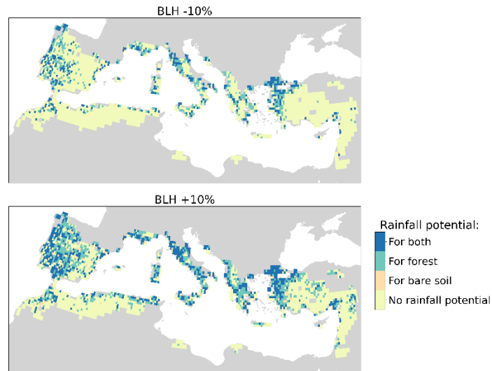
620 Figure A9: Sensitivity of rainfall potential to a change in the boundary layer height (BLH). Top: a change in BLH of -10%, bottom: a change in BLH of +10%. This plot indicates for each grid cell if most samples have a rainfall potential over bare soil, forest, both land cover types or no rainfall potential in any of the samples.
