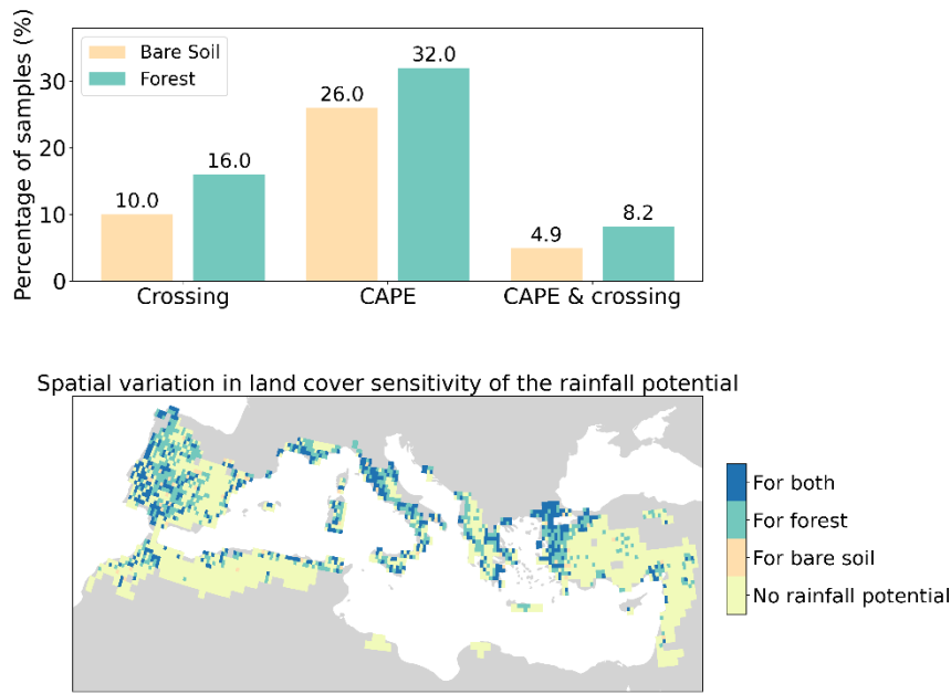
345 Figure 4: Top: The percentage of samples with a crossing, sufficient CAPE ( \geq 400 \text{ J kg}^{-1} ), or both sufficient CAPE and a crossing for the Mediterranean Basin when covered in either forest or bare soil. Bottom: The spatial variability of the land cover sensitivity of the convective rainfall potential, i.e., there is both a crossing of the ABL and LCL ( ABL \geq LCL ) and sufficient CAPE ( \geq 400 \text{ J kg}^{-1} ), if one or both of these conditions are not met there is no convective rainfall potential. This plot indicates for each grid cell if most samples have a convective rainfall potential over bare soil, forest or both land cover types or if they have no convective rainfall potential in any of the samples. These results are obtained from the model runs in which only the parameters that are related to land cover are varied. All other variables remain similar to the realistic situation and are obtained (directly or indirectly) from ERA5. 350
