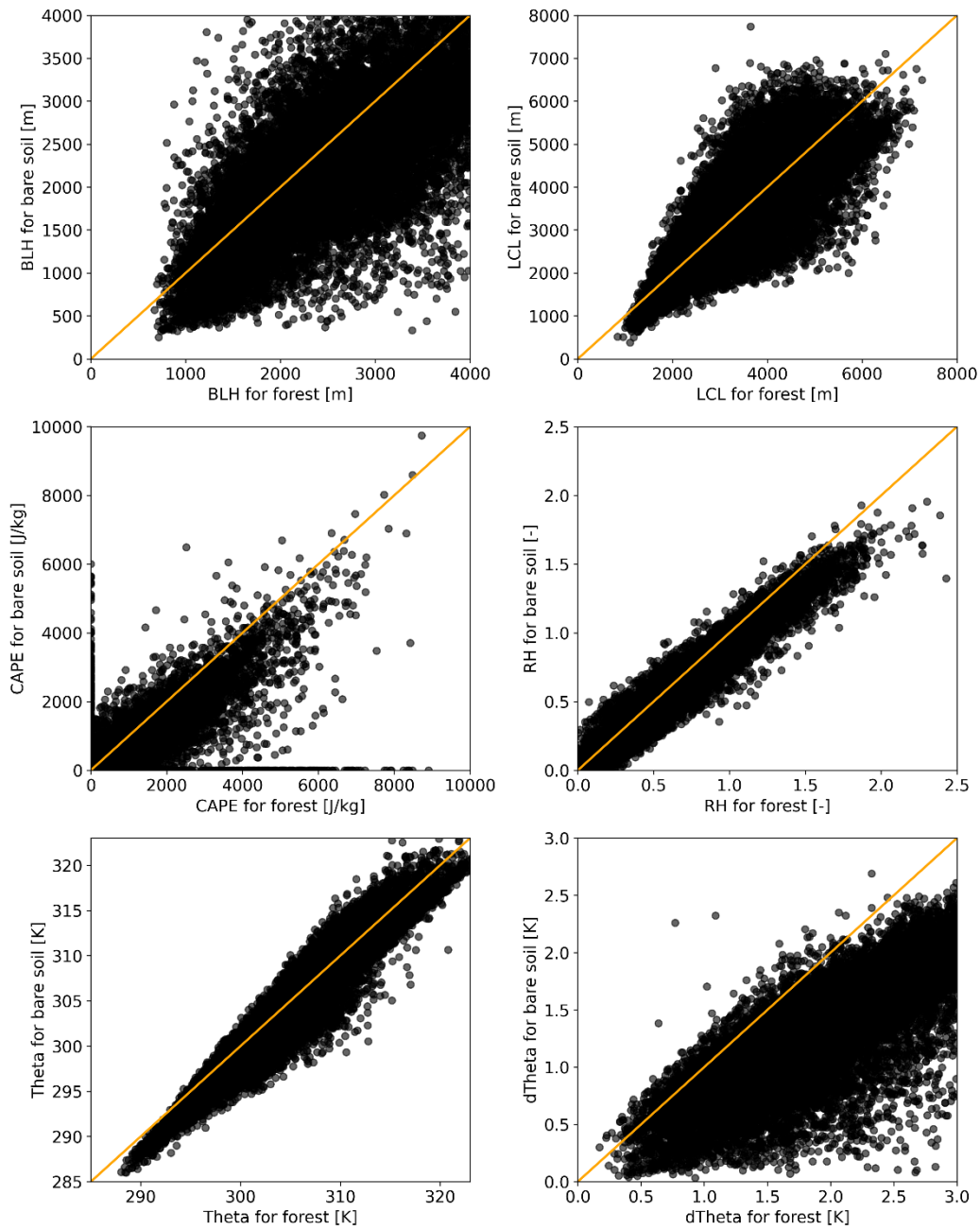
570 Figure A4: Output of the bare soil scenario and forest scenario for all samples that pass the postprocessing filter for boundary layer height (BLH), lifting condensation level (LCL), convective available potential energy (CAPE), relative humidity (RH), potential temperature (Theta), and the jump in potential temperature at the top of the boundary layer (dTheta). The orange line indicates the identity line ( x=y ).
