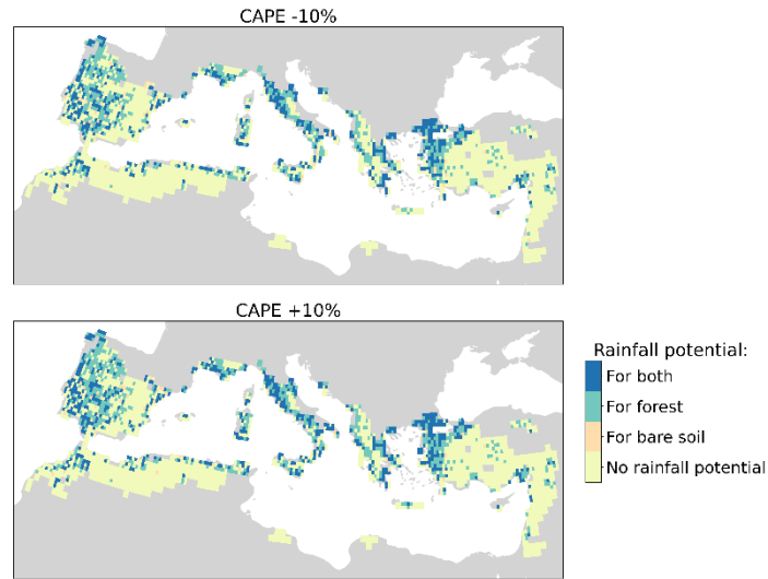
600 Figure A10: Sensitivity of rainfall potential to a change in the convective available potential energy (CAPE). Top: a change in CAPE of -10%, bottom: a change in CAPE of +10%. This plot indicates for each grid cell if most samples have a rainfall potential over bare soil, forest, both land cover types or no rainfall potential in any of the samples.
