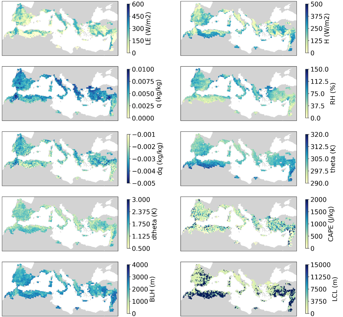
Figure A6: CLASS output for the bare soil scenario. For each variable the mean value per grid cell is shown. Note that due to filtering the amount of samples varies among the grid cells. The output that is shown is the latent heat flux (LE), sensible heat flux (H), specific humidity (q), relative humidity (RH), jump in specific humidity at the top of the boundary layer (dq), potential temperature (theta), jump in potential temperature at the top of the boundary layer (dtheta), convective available potential energy (CAPE), boundary layer height (BLH), and lifting condensation level (LCL).
