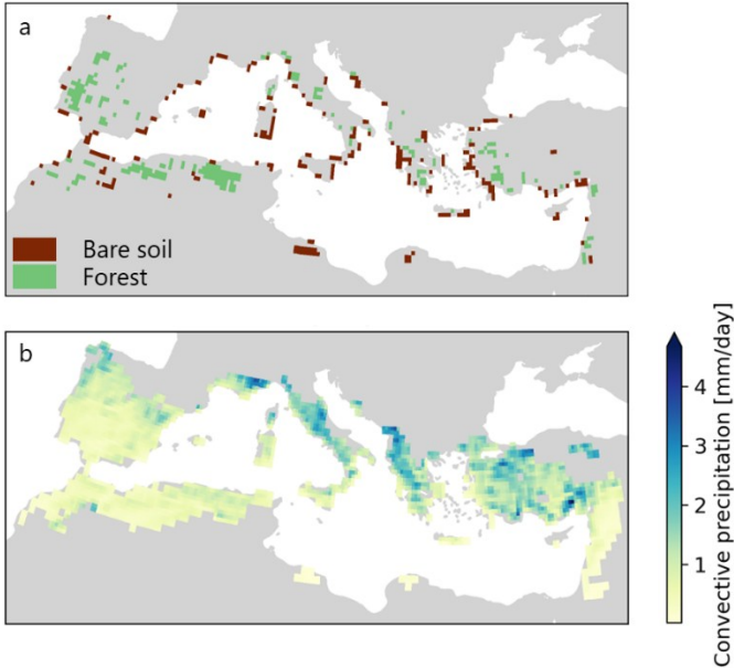
555 Figure A1: Characteristics of the Mediterranean Basin. (a) Grid cells with mostly bare soil or forest cover. For grid cells with bare soil, both tall vegetation cover and short vegetation cover are smaller than or equal to 0.1. For grid cells with forest, tall vegetation cover is larger than or equal to 0.8. (b) Mean convective precipitation (mm/day) for the months May and June between the years 2013 and 2022. The data for these plots is obtained from the ERA5 data set.
