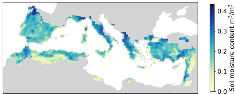
120 Figure 2: The soil moisture content in the top layer for all regions around the Mediterranean Sea that have a Mediterranean climate according to the Köppen climate classification. This plot shows the mean soil moisture content in May and June for the years 2013-2022 and the data is obtained from ERA5.
