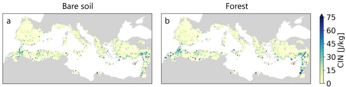
605 Figure A11: Convective inhibition (CIN) for the bare soil (a) and forest (b) scenarios. The plots indicate the mean value of all runs for each grid cell separately.
