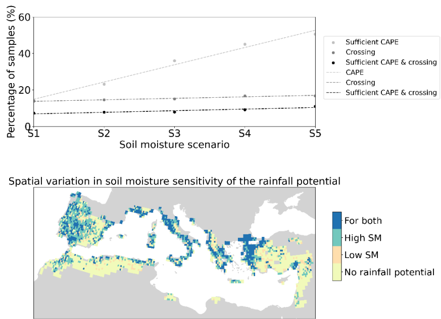
355 Figure 5: Top: The percentage of samples with a crossing, sufficient CAPE ( \geq 400 \text{ J kg}^{-1} ), or both sufficient CAPE and a crossing for varying soil moisture content. The different soil moisture scenarios increase linearly from wilting point (S1, 0.15 \text{ m}^3\text{m}^{-3} ) to field capacity (S5, 0.35 \text{ m}^3\text{m}^{-3} ). The dotted lines are the regression lines (CAPE: R^2 = 0.98 , crossing: R^2 = 0.93 , CAPE & crossing: R^2 = 0.87 ). Bottom: The spatial variability of the soil moisture sensitivity of the convective rainfall potential, i.e., there is both a crossing of the ABL and LCL ( \text{ABL} \geq \text{LCL} ) and sufficient CAPE ( \geq 400 \text{ J kg}^{-1} ), if one or both of these conditions are not met there is no convective rainfall potential. This plot indicates for each grid cell if most samples have a convective rainfall potential for soil moisture scenario 1, soil moisture scenario 5, or both soil moisture scenarios, or no convective rainfall potential in any of the samples.
