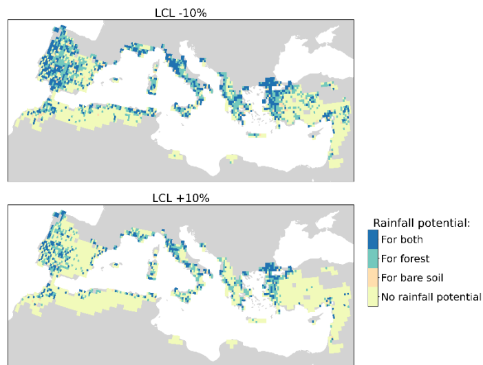
Figure A9: Sensitivity of rainfall potential to a change in the lifting condensation level (LCL). Top: a change in LCL of -10%, bottom: a change in LCL of +10%. This plot indicates for each grid cell if most samples have a rainfall potential over bare soil, forest, both land cover types or no rainfall potential in any of the samples.
