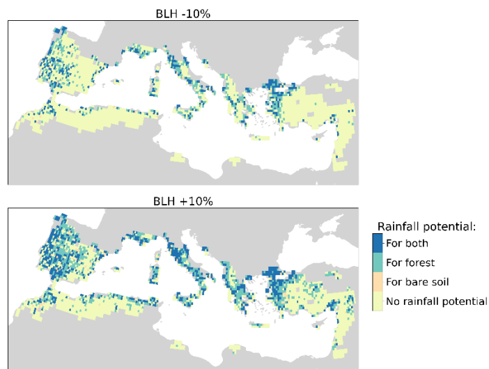
Figure A8: Sensitivity of rainfall potential to a change in the boundary layer height (BLH). Top: a change in BLH of -10%, bottom: a change in BLH of +10%. This plot indicates for each grid cell if most samples have a rainfall potential over bare soil, forest, both land cover types or no rainfall potential in any of the samples.
