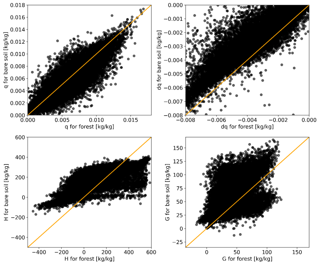
575 Figure A5: Output of the bare soil scenario and forest scenario for all samples that pass the postprocessing filter at 3 PM for specific humidity ( q ), jump in specific humidity at the top of the boundary layer ( dq ), sensible heat flux ( H ), ground heat flux ( G ). The orange line indicates the identity line ( x=y ).
