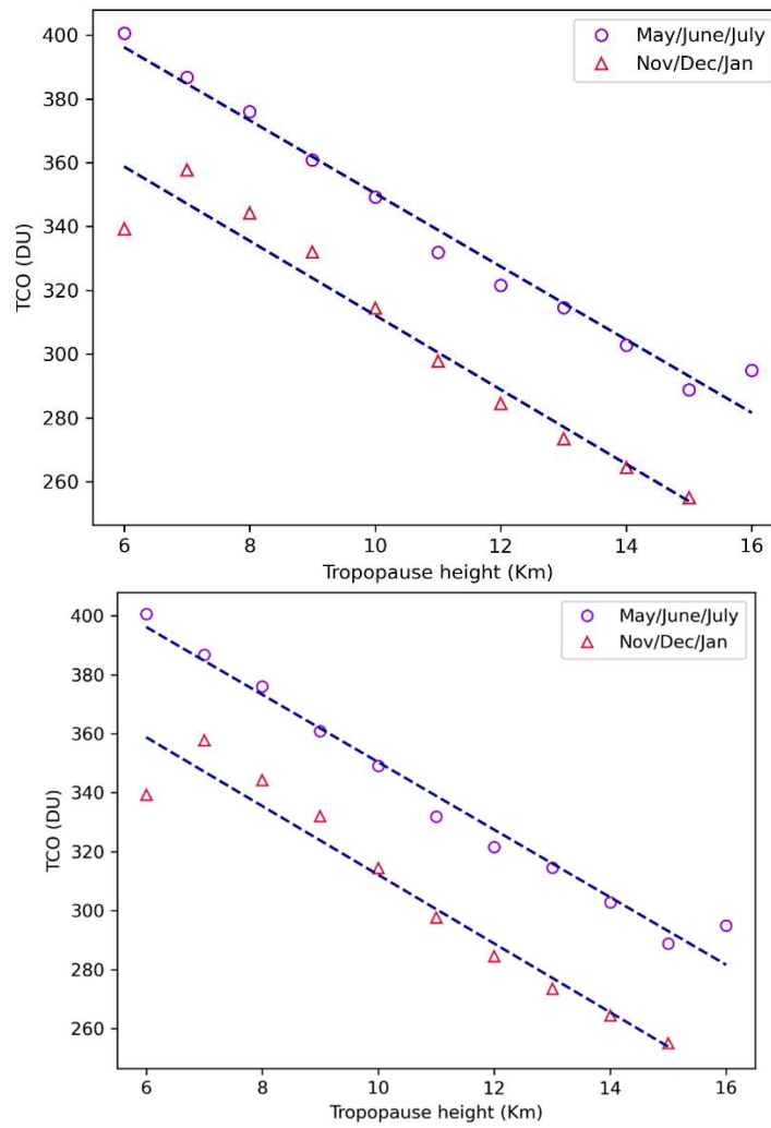
Figure 5 Linear fit of TCO means obtained for different ranges of tropopause height during the May, June, and July (purple) and November, December, and January (red) periods. The data set considered for the plot corresponds to days between 18 August 1993 and 31 May 2024, when daily means for both tropopause height and TCO are available.
