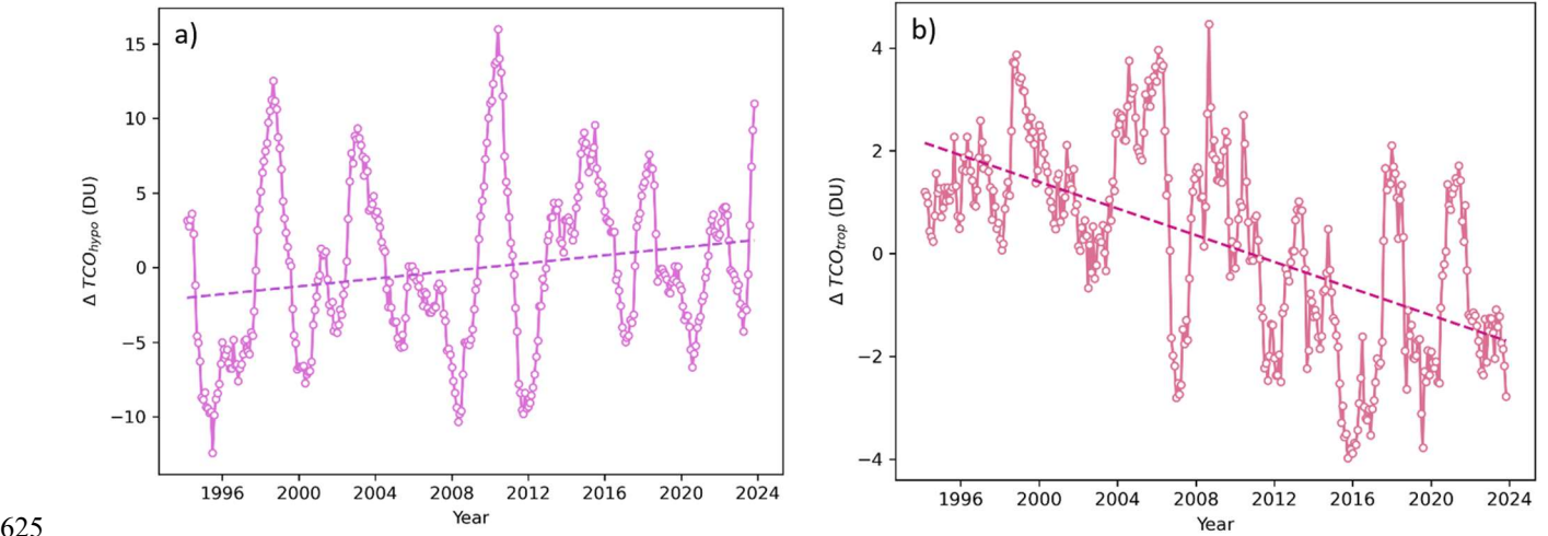
Figure 7 Time series of deseasonalised monthly running means of (a) hypothetical TCO and (b) TCO related to tropopause height from March 1994 to November 2023 (circles). Dashed lines indicate linear fits to the data.
