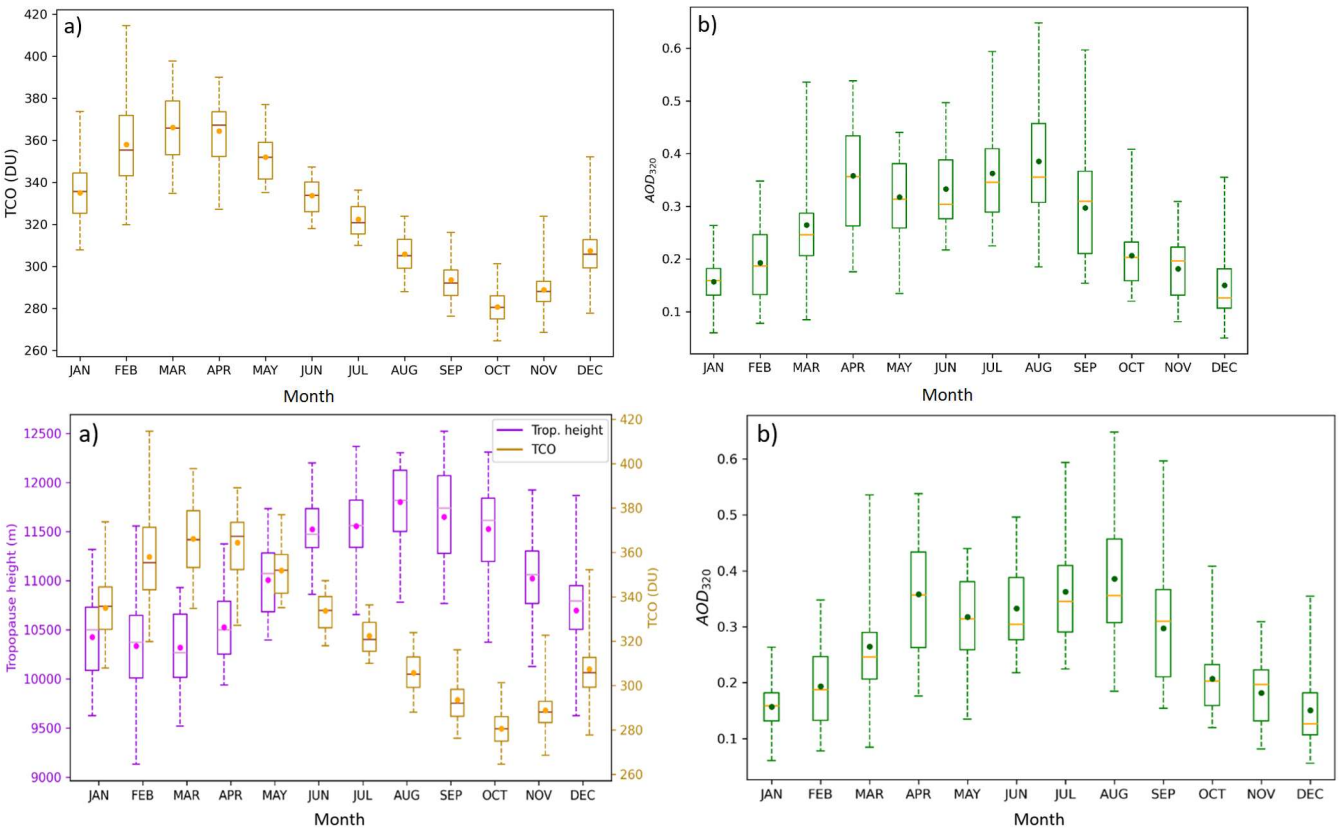
Figure 2 Boxplots showing the statistical distribution of the tropopause height (left vertical axis) together with the TCO (right vertical axis) of TCO (a) and AOD 320 (b) for each month based on data from September 1993 to May 2024. The means are
