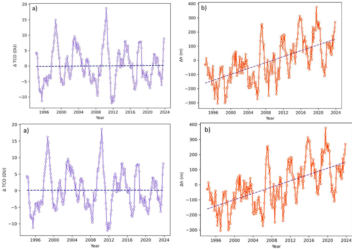
Figure 6 Representation of the time evolution of deseasonalized monthly running means of TCO (a) and tropopause height (b) from March 1994 to November 2023 (circles). Dashed lines represent linear fits to the data.
