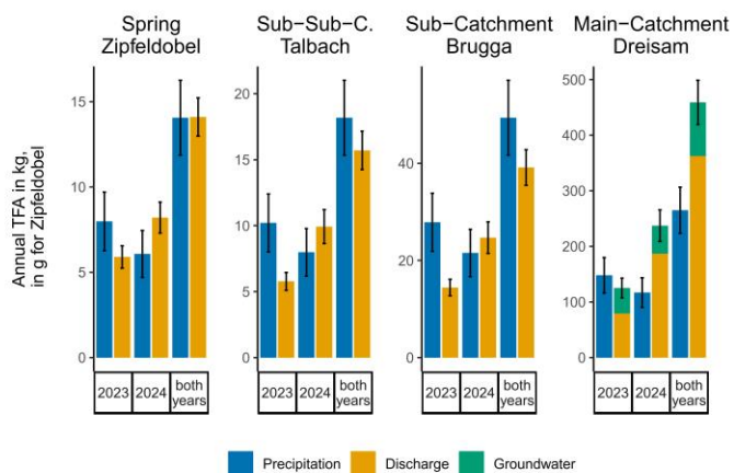
365 Figure 4: The TFA mass balance for the spring Zipfeldobel, the nested sub-catchments Talbach and Brugga, and the DRC. Whiskers indicate statistical significance as standard errors, calculated from bootstrapped standard errors for mean concentrations and volumes and consecutive Gaussian error propagation.
