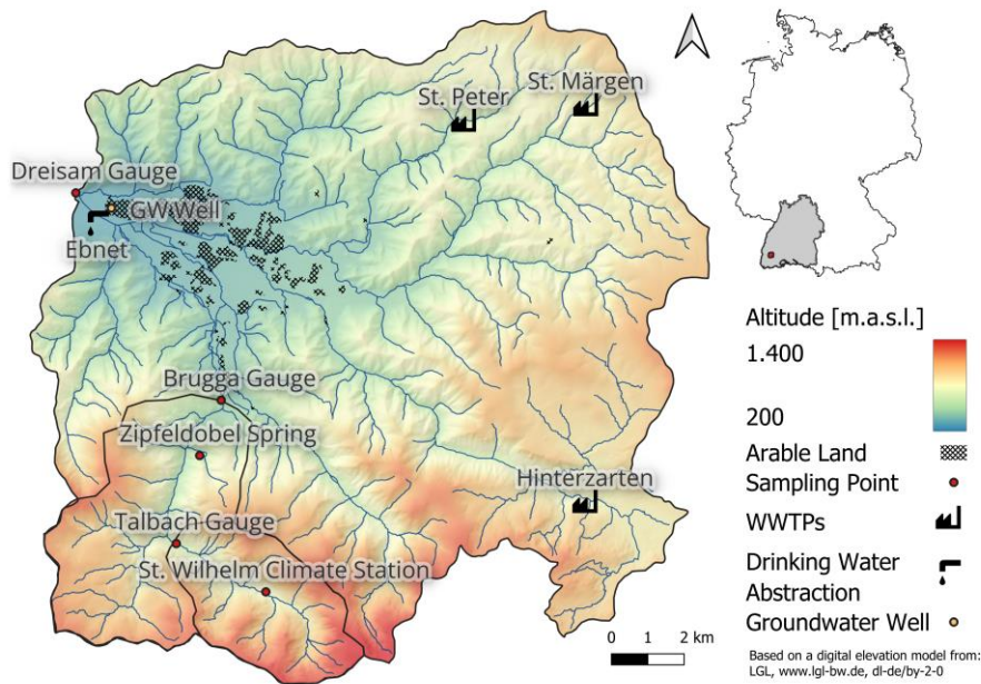
80 Figure 1: The Dreisam catchment: sampling locations and sites with potential TFA input.
