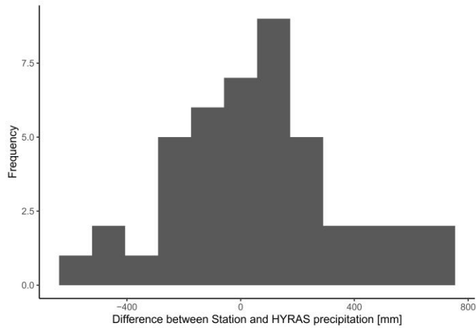
620 Figure D3: D istribution of differences between the annual station and HYRAS precipitation data.
