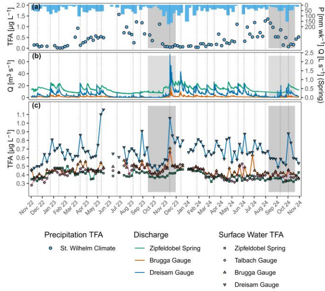
305 Figure 2: Time series of precipitation, discharge, and TFA concentrations. Grey areas, showing changes from dry to wet conditions, are highlighted in Figure 3. (a) Weekly precipitation is plotted against the corresponding weekly TFA concentration in rainwater at the St. Wilhelm station. (b) Dreisam, Brugga, and Zipfeldobel Spring discharge. (c) Weekly TFA concentration measurements in four surface waters of the DRC. Vertical dotted lines indicate discharge events.
