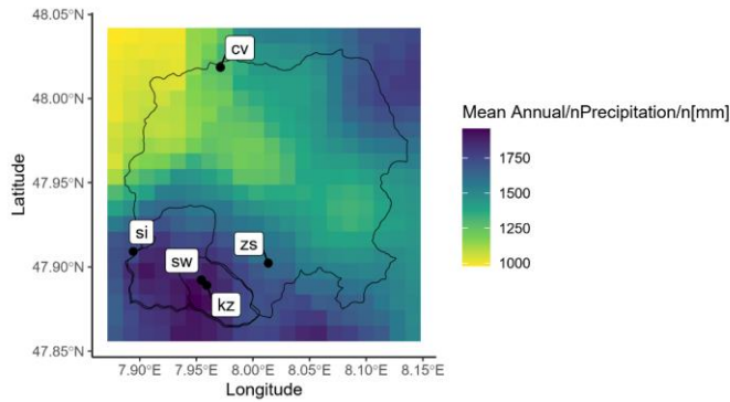
Figure D1: Annual mean precipitation of the HYRAS interpolation product. Points indicate climate stations not included in the interpolation algorithm and used for error estimation.
