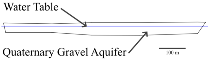
595 Figure C2: Geologic profile of the aquifer below the Dreisam gauge.
