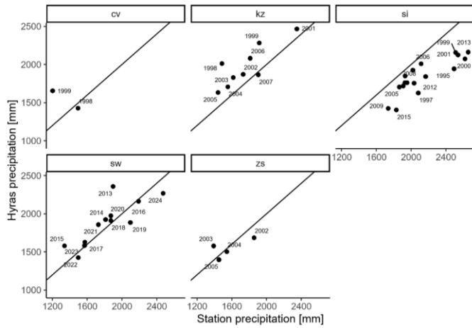
615 Figure D2: Comparison of annual HYRAS precipitation data with five climate stations' values. The black line indicates the perfect fit.
