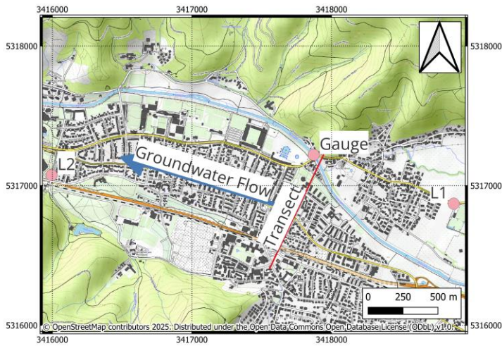
Figure C1: DRC gauge area. Groundwater wells L1 and L2, the transect on which a geologic profile was taken, and the main groundwater flow direction (blue arrow).
