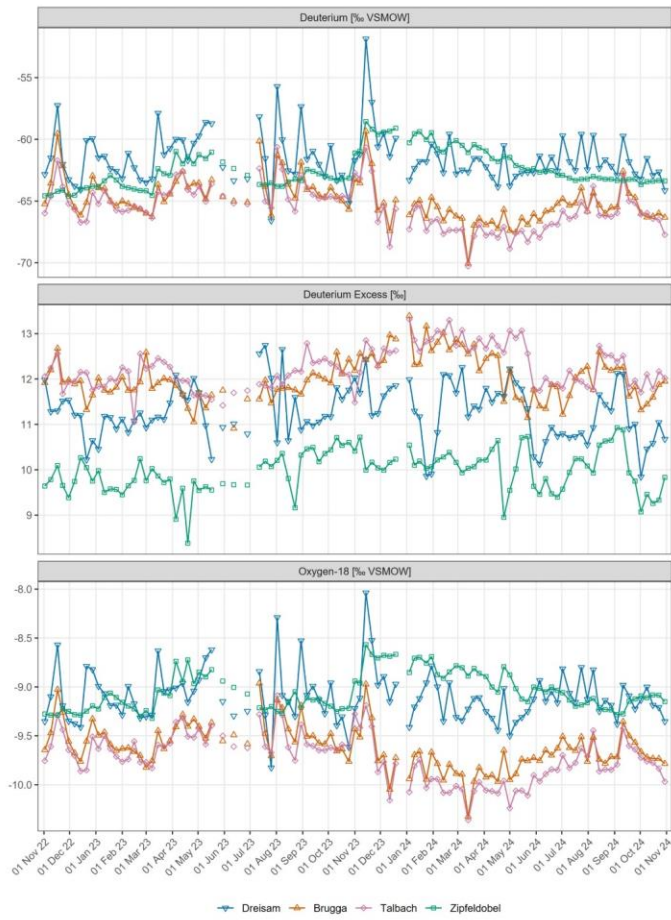
635 Figure F1: Time series of isotopic tracer data recorded in surface waters for the hydrological years 2023 and 2024.
