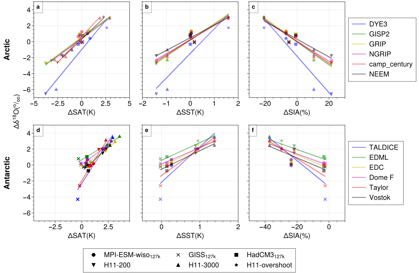
Figure A8. \Delta SAT at each ice core location (first column), \Delta SST (north/south of 40^\circ latitude for Arctic and the Antarctica) and \Delta SIA (annual sea ice area) versus \Delta\delta^{18}\text{O} from each ice core sites, for all simulations.
