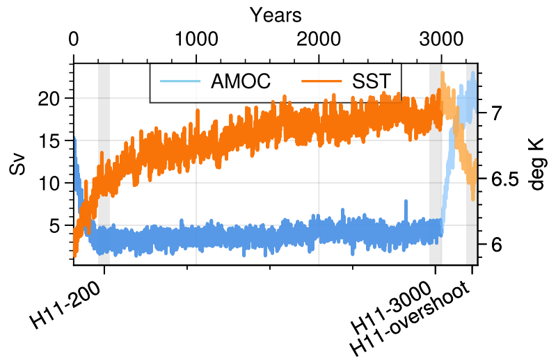
Figure A2. Time series of AMOC (in Sv) and average Southern Hemisphere SST (south of 40°S) time series from HadCM3 H11 simulations. The lighter colors represent the period where the water hosing was stopped. The three grey bands denote the three selected slices from this simulation: H11-200; H11-3000; and H11-overshoot.
