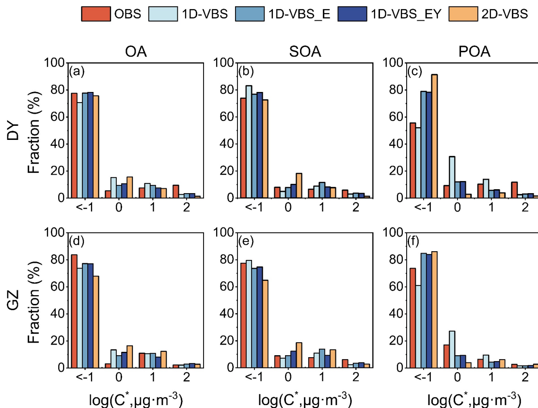
Figure 2: Simulated volatility distributions of OA, POA, and SOA across volatility bins with C^* up to 10^2 \mu\text{g m}^{-3} , compared to the observations in DY (a-c) and GZ (d - f). The compounds with C^* equal or below 10^{-1} \mu\text{g m}^{-3} were grouped into a single volatility bin, and referred to as low-volatility OA in this study.
