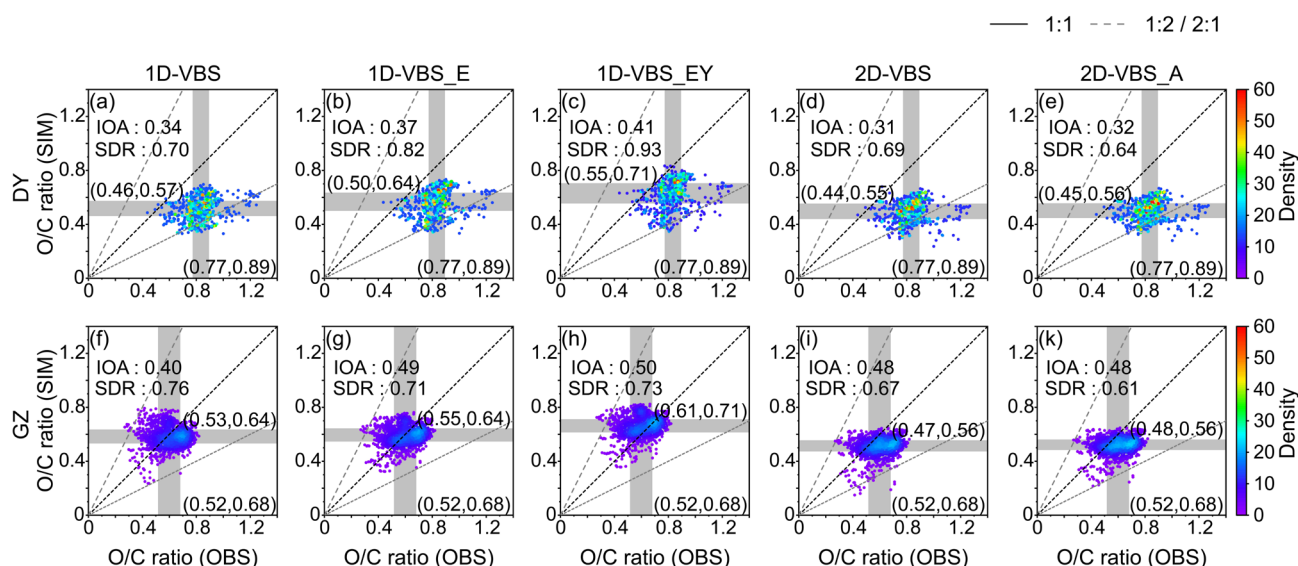
395 Figure 4: Density distribution of simulated versus observed hourly O/C ratios of OA in DY (a-e) and GZ (f-k). The edges of the grey shading represent the 25 th and 75 th percentiles in both the observations and simulations, with the shading indicating the interquartile range (IQR). The Index of Agreement (IOA, reflecting both bias and variability) and Standard Deviation Ratio ( \sigma_{sim}/\sigma_{obs} , comparing the magnitude of variability in simulations and observations) are calculated.
