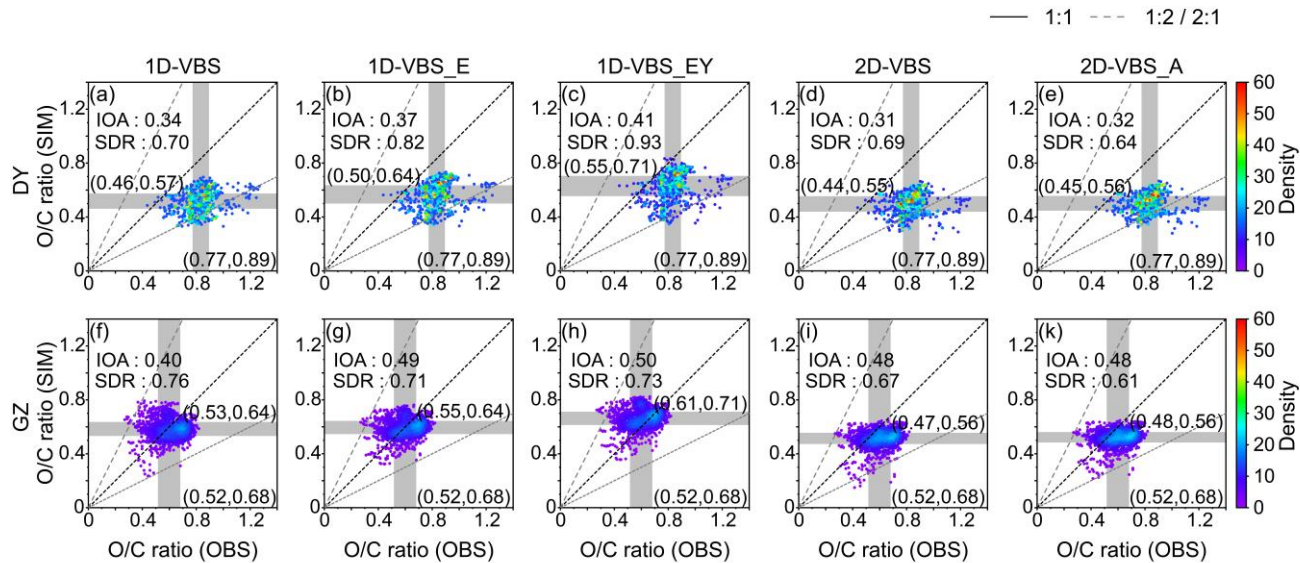
415 Figure 4: Density distribution of simulated versus observed hourly O/C ratios of OA in DY (a-e) and GZ (f-k). The edges of the grey shading represent the 25 th and 75 th percentiles in both the observations and simulations, with the shading indicating the interquartile range (IQR). The Index of Agreement (IOA, reflecting both bias and variability) and Standard Deviation Ratio ( \sigma_{sim}/\sigma_{obs} , comparing the magnitude of variability in simulations and observations) are calculated.
