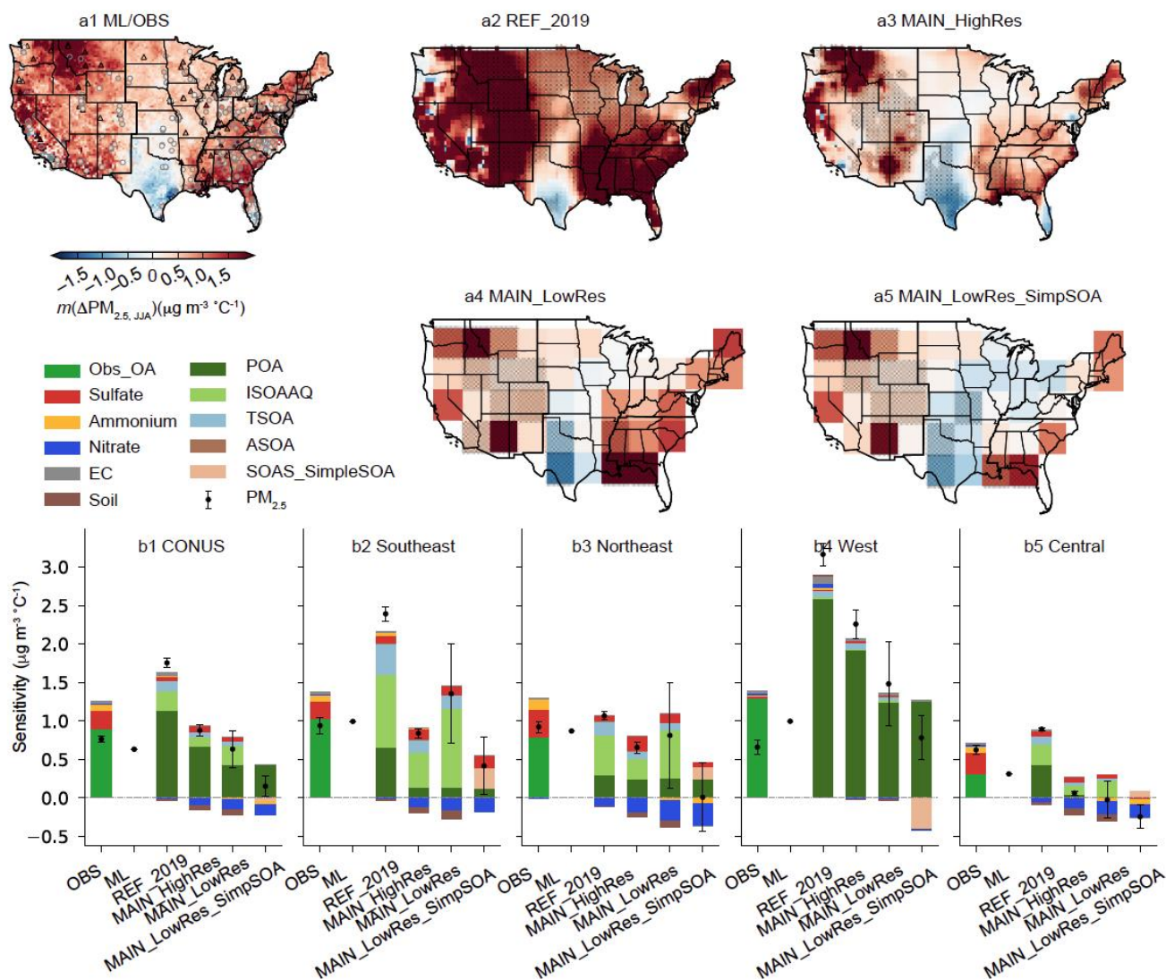
280 Figure 1: Spatial distribution and regionally aggregated temperature sensitivity of summertime PM 2.5 and its major components during 2000–2016, derived from ground-based observations, machine-learning (ML) modeled datasets, and GEOS-Chem simulations. Maps show the spatial distribution of PM 2.5 temperature sensitivity derived from ML-modeled data and observations (a1), GEOS-Chem REF_2019 case simulations (a2), MAIN_HighRes case simulations (a3), MAIN_LowRes case (a4), and MAIN_LowRes_SimpSOA case (a5). Triangle markers represent fitted sensitivities from observations with p -value <0.05 . Stippling 285 represents fitted temperature sensitivities with p -value <0.05 in GEOS-Chem. Bar charts show regionally aggregated temperature sensitivities for PM 2.5 and its major components across the contiguous United States (b1), the Southeastern US (b2), the Northeastern US (b3), the Western US (b4), and the Central US (b5).
