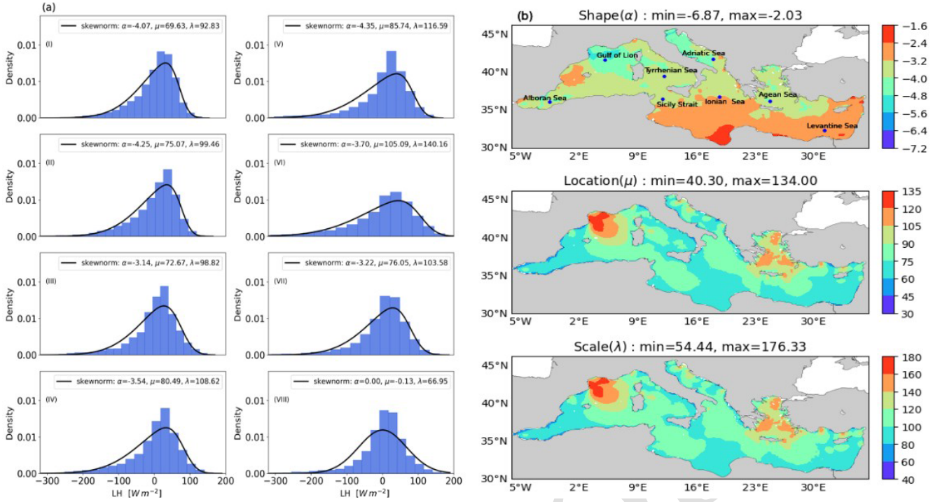
Figure 5. (a) The single grid point histograms for LH flux anomalies at the eight sampling locations for the period of 2006002020, (b) the skew-normal PDF parameter ( \alpha , \mu , \lambda ) distributions for computed LH flux anomaly for the observation period – sampling points: (I) Alboran Sea, (II) Gulf of Lion, (III) Tyrrhenian Sea, (IV) Sicily Strait, (V) Adriatic Sea, (VI) Ionian Sea, (VII) Aegean Sea, (VIII) Levantine Sea.
