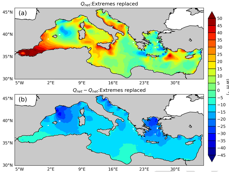
Figure 8. (a) Long term mean net heat flux after the removal of extremes ( Q_{net} : extremes replaced) using threshold of -289 \text{ W m}^{-2} ( K = 0.75 ). (b) The time mean distribution computed from the difference between Q_{net} (Fig. 3a) and “ Q_{net} : extremes replaced” time series. It shows a significant reduction of heat losses in the Gulf of Lion, Adriatic Sea and Aegean Sea regions.
