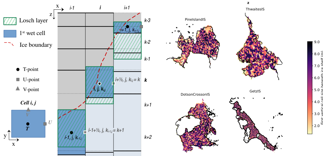
Figure 2. (a) Sketch of partial step z^* -coordinate grid showing the ice shelf in grey (deactivated cells) and the ocean in light blue in x - z coordinates. The first wet cell under the ice shelf is colored in dark blue and the Losch layer is hatched in green. In the bottom left corner, the cell (i, j) in x - y coordinates is shown with T-, U- and V-points. (b) First wet cell height below ice shelves in the ASE configuration with 121 layers: Pine Island, Thwaites, Dotson-Crosson and Getz from left to right.
