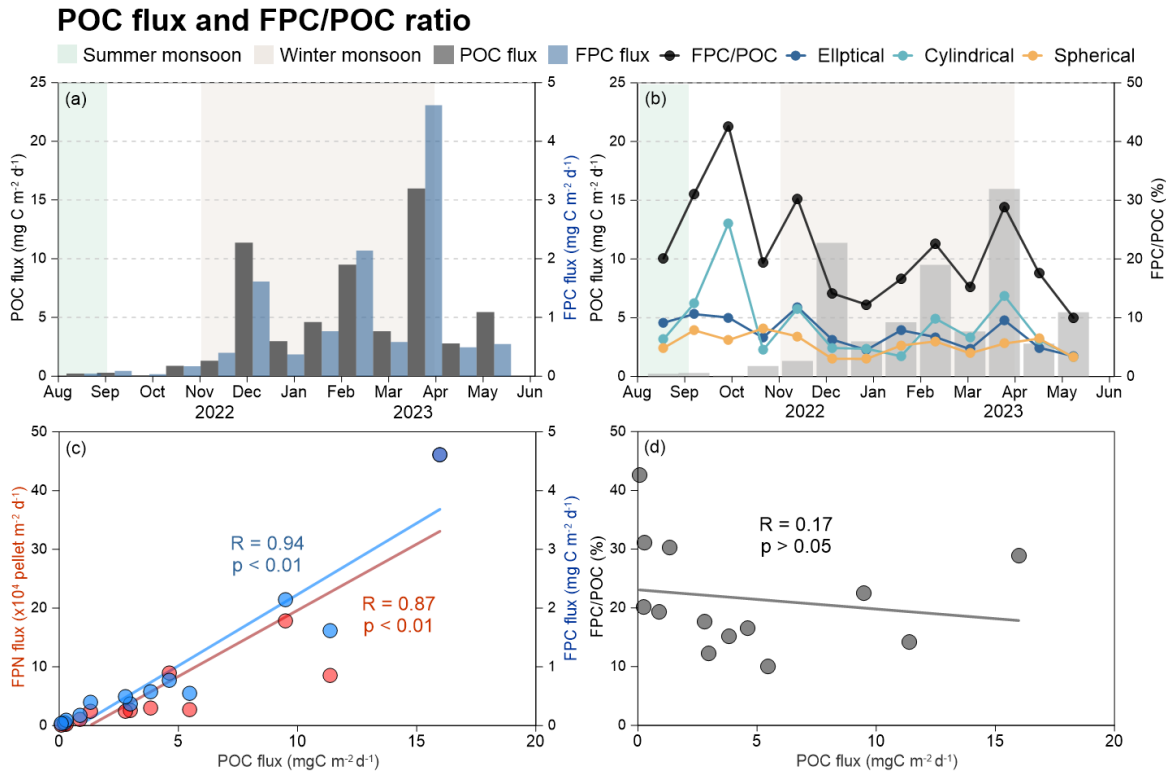
Figure 4. POC flux and FPC/POC ratio at Mooring TJ-S in the southern SCS. (a) Total POC flux and FPC flux; (b) FPC/POC ratio; (c) correlations between FPC flux, FPN flux, and POC flux; (d) correlations between FPC/POC ratio and POC flux. Solid lines indicate a linear correlation with a coefficient of R.
