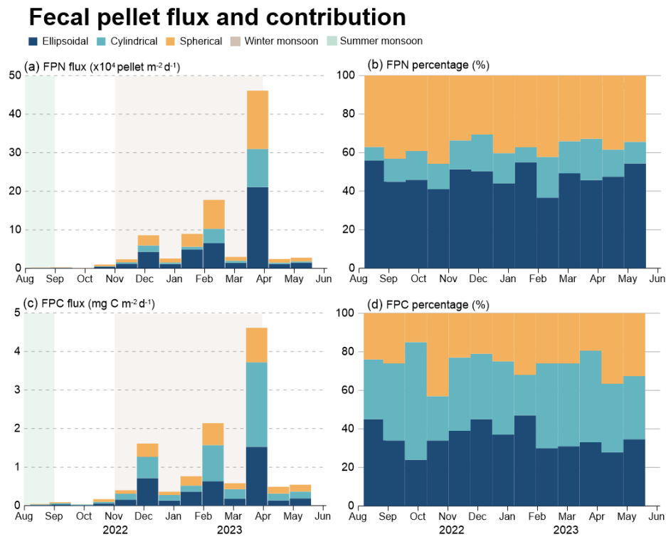
Figure 3. Time-series variation of FPN and FPC at sediment trap Mooring TJ-S (500 m) in the southern SCS. (a) FPN flux; (b) FPN percentage; (c) FPC flux; (d) FPC percentage.
