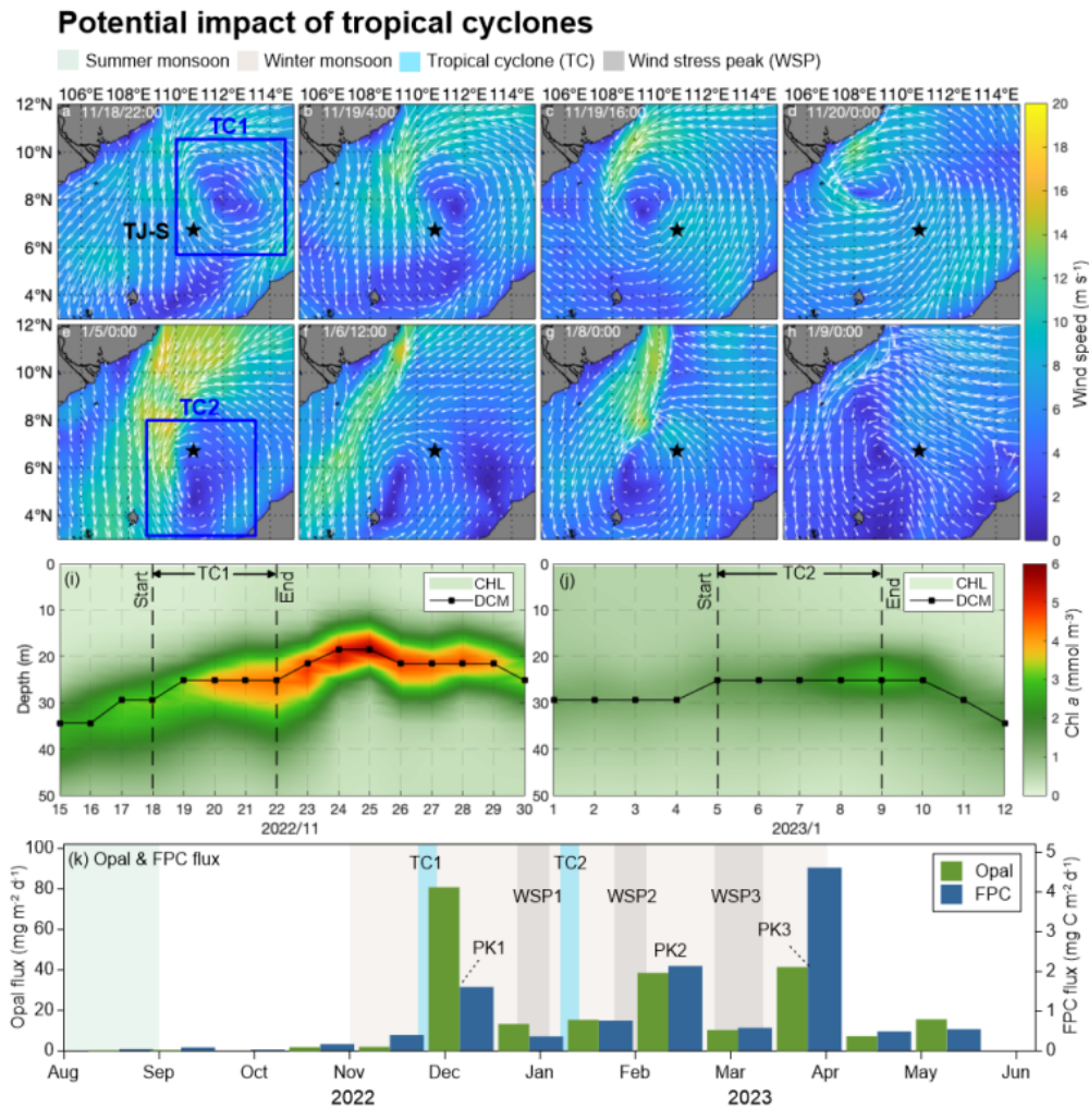
Figure 7. The possible impact of tropical cyclones at TJ-S. (a–d) Surface wind field from 18–20 November 2022, representing the passage of TC1. (e, f) Surface wind field from 05–09 January 2023, representing the possible impact of TC2. (i, j) Chl a concentration and DCM variations during the passage of TC1 and TC2. (k) Opal flux and FPC flux. 320
