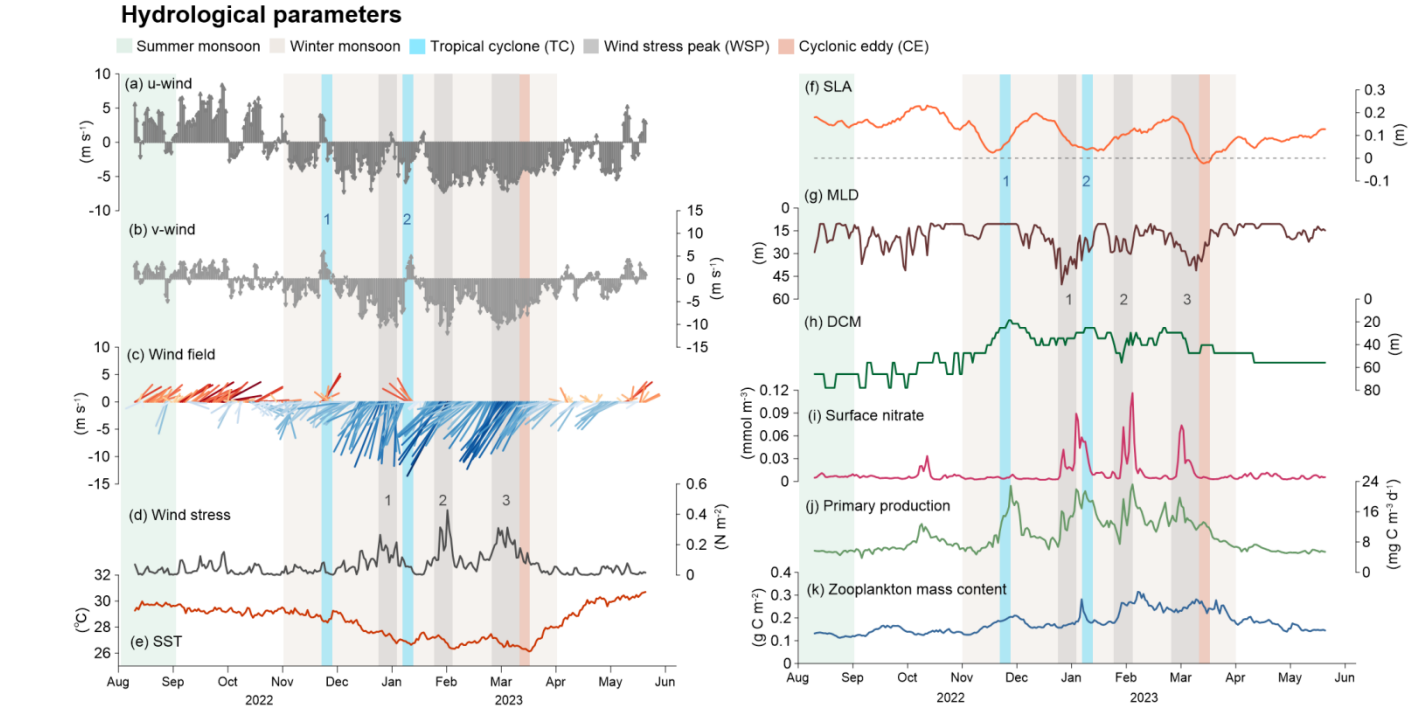
240 Figure 5. Hydrological parameters at the sediment trap Mooring TJ-S in the southern SCS. (a) eastward component for 10 m wind (u), where positive values represent eastern winds, and negative values for western wind; (b) northward component for 10 m wind (v), where positive values represent northern winds, and negative values for southern winds; (c) wind field; (d) wind stress; (e) sea surface temperature (SST); (f) sea level anomaly (SLA); (g) mixed layer depth (MLD); (h) deep chlorophyll maximum (DCM); (i) surface nitrate; (j) net primary productivity (NPP); (k) zooplankton mass content expressed in carbon.
