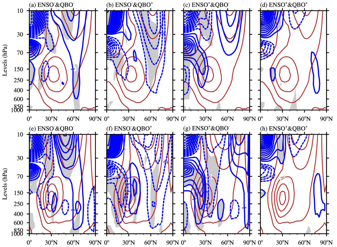
Figure 9: Climatological mean of the zonal-mean zonal winds (red contours; unit: \text{m s}^{-1} ) and composite zonal-mean zonal winds (blue contours; unit: \text{m s}^{-1} ) in 0^\circ – 360^\circ\text{E} for (a) La Niña and EQBO, (b) La Niña and WQBO, (c) El Niño and EQBO, and (d) El Niño and WQBO. (e)–(f) Same as (a)–(d), but for zonal winds averaged in 0^\circ – 140^\circ\text{E} . Grey shaded areas indicate significant values at the 90% confidence level.
