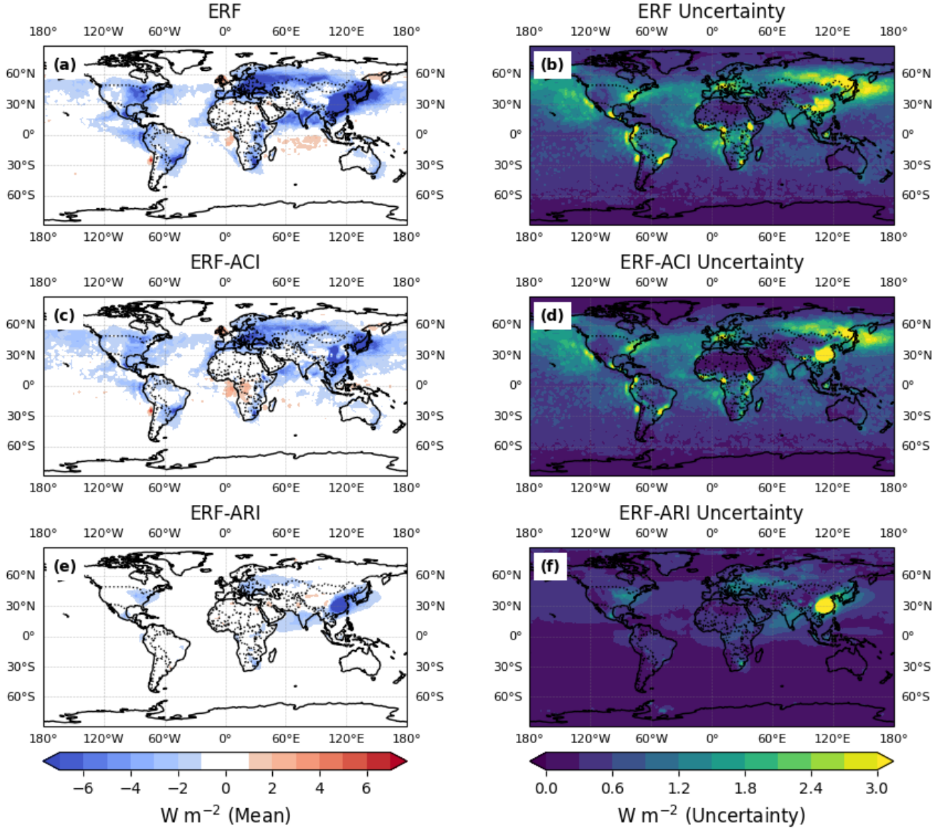
Figure 2. Annual emulated mean (a) ERF, (c) \text{ERF}_{aci} , (e) \text{ERF}_{ari} and 2 \times standard deviation ( 2\sigma ) (b) ERF, (d) \text{ERF}_{aci} , (f) \text{ERF}_{ari} . 3 million model variants are used to calculate the mean and standard deviation.
