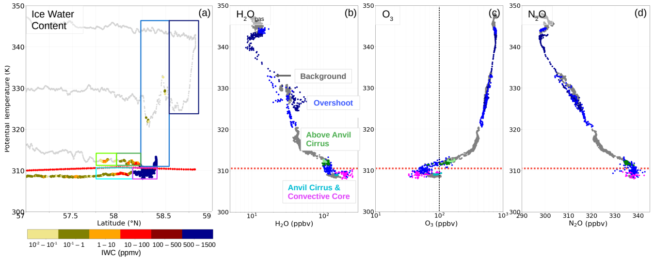
Figure 5. Observations versus potential temperature. (a) IWC, (b) H_2O_{gas} , (c) O_3 , and (d) N_2O along the flight track, as function of latitude and potential temperature. The colored boxes in (a) and corresponding labels in (b) denote different filaments of convectively influenced air encountered along the flight path. The red dotted line marks the lapse rate tropopause, and the black dotted line in (c) the 100 ppbv O_3 threshold.
