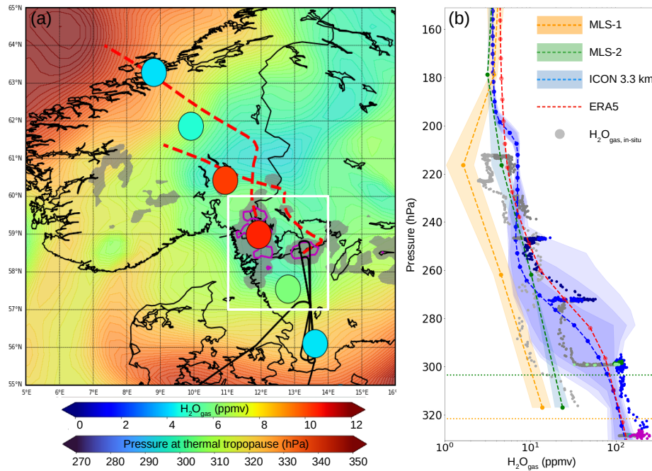
Figure 8. Comparison of in-situ measurements with MLS, ERA5 and ICON. (a) MLS observations (circles) of water vapor at the 260 hPa level, taken around 12 UTC on the day of the convection event. Overlaid are thermal tropopause pressures from ERA5 reanalysis. Red dashed lines represent 24-hour forward trajectories. Grey shaded areas indicate where cloud-top temperatures were below -40^{\circ}\text{C} during the MLS overpass. Magenta contours mark cloud tops that reached or potentially exceeded the tropopause. (b) Vertical pressure profiles of water vapor from multiple sources (gray in-situ, green and blue MLS, orange ICON and red ERA5). Two MLS averaged profiles are shown: one for the region between 59^{\circ} and 61^{\circ} N close to the convection (MLS-2), and another for four profiles located to the north and south of this zone (MLS-1); corresponding mean tropopause levels are indicated by the dotted lines. The dashed line and the shaded area indicate the median and range of MLS observation, respectively. For the ICON model, averaged over the white box region shown in (a), the median profile (dashed line) is plotted along with confidence intervals (shaded) representing the 5–95 %, 1–99 %, and 0.1–99.9 % ranges. ERA5 mean profile is shown for the same area as for ICON. In-situ measurements are also included, with different colors corresponding to specific areas defined in Figure 5.
