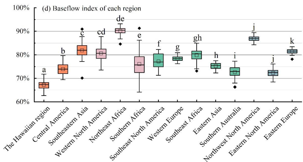
Figure 9. Distribution of BFIs in karst basins in different regions within the same climatic zone. In figure (d), orange represents tropical karst regions, magenta represents arid karst regions, green bars represent subtropical karst regions, and brownish-purple represents temperate karst regions.
