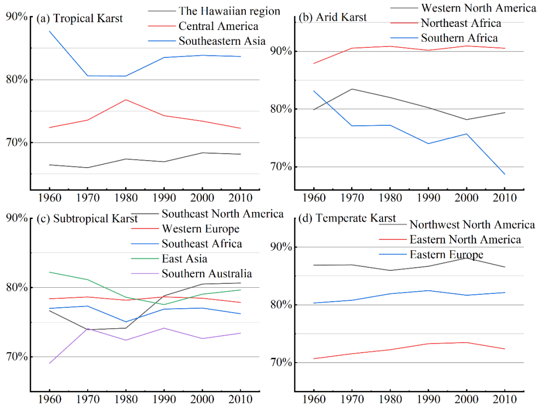
Figure 10. Characteristics of BFIs with respect to year for different regions within the same climatic zone. Where Y-axis indicates BFI and X-axis indicates year.
