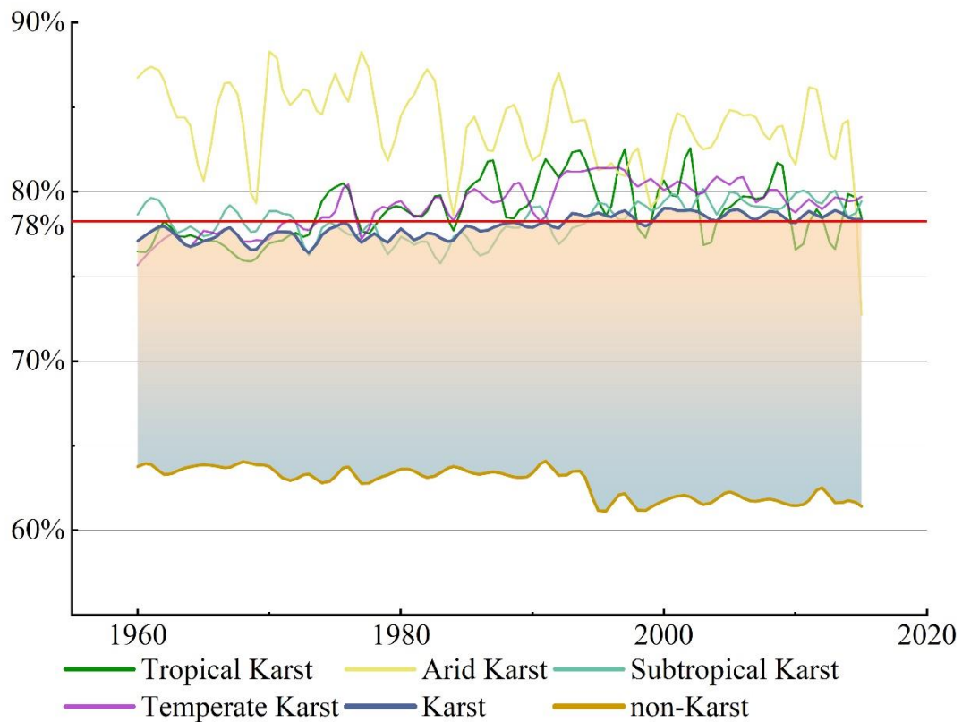
Figure 7. Temporal variations of annual BFI for different karst climatic zones compared to the global average. The x-axis indicates the year, and the y-axis indicates the BFI percentage. The thin colored lines represent the BFI fluctuations in Arid (yellow), Tropical (green), Subtropical (teal), and Temperate (purple) karst regions. The dark blue line represents the weighted average BFI for all karst regions ("Karst"), while the brown curve at the bottom represents the non-Karst average BFI ("non-Karst "). The red horizontal line marks the long-term overall mean of the karst BFI (approximately 78%).
