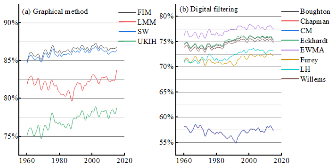
Figure 5. Global BFIs for karst regions calculated by the 12 baseflow separation
