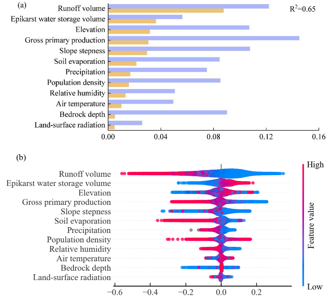
Figure 11. Contribution of different factors to baseflow and their characteristic distributions. Subfigure (a) illustrates the feature importance derived from XGBOOST and SHAP analysis, with R^2 representing the coefficient of determination of the XGBOOST model. Subfigure (b) depicts the influence characteristics of various factors on the baseflow index, where the horizontal axis indicates the magnitude of values and the vertical axis lists the different factor types.
