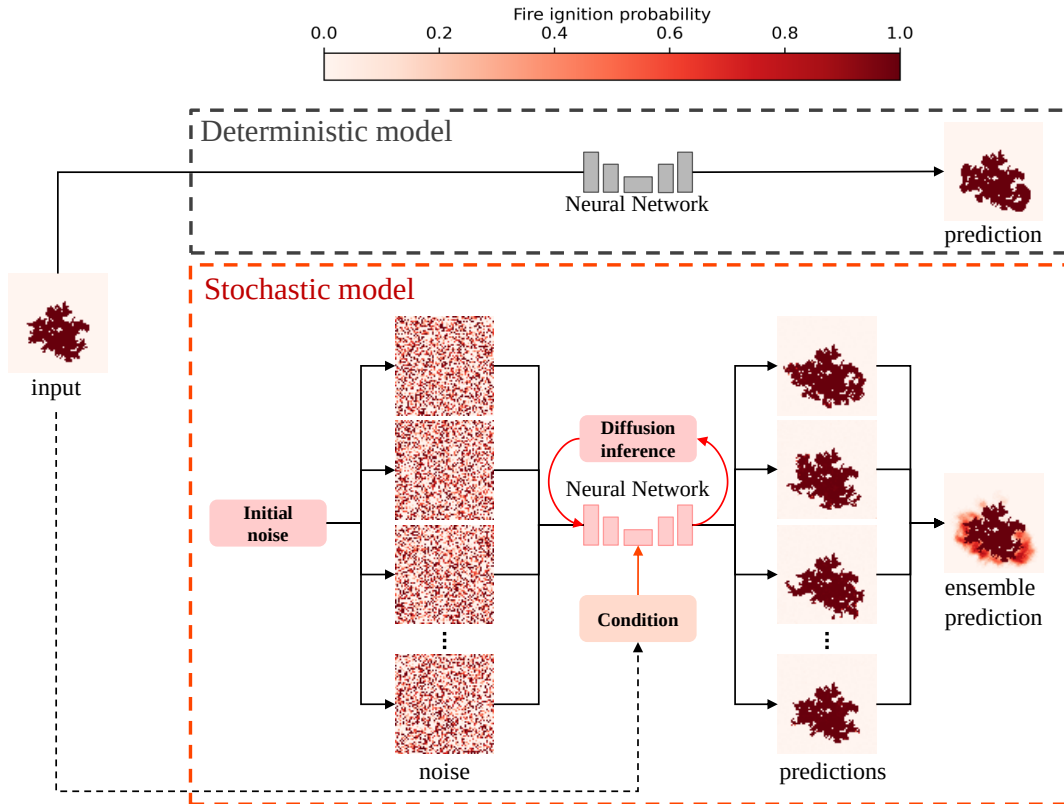
Figure 1. Deterministic and stochastic models.
