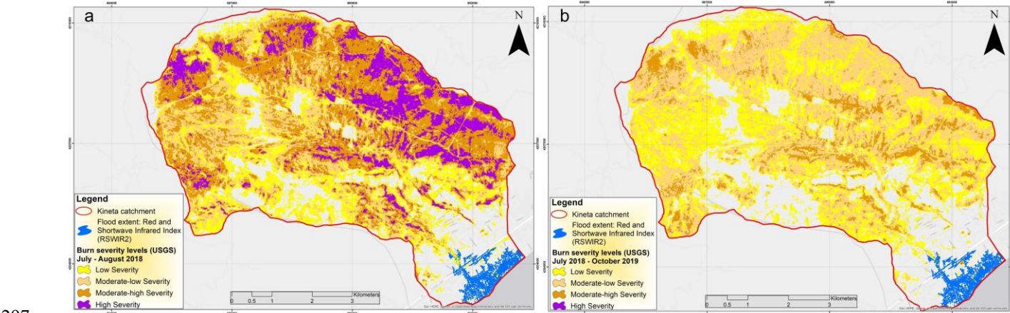
Figure 4: The RS results of the a) burn extent and severity of the wildfire period July-August 2018, b) burn extent and severity of the post-wildfire period July 2018- October 2019, both illustrating the flood extent (November 2019) according to the RSWIR2 index.
