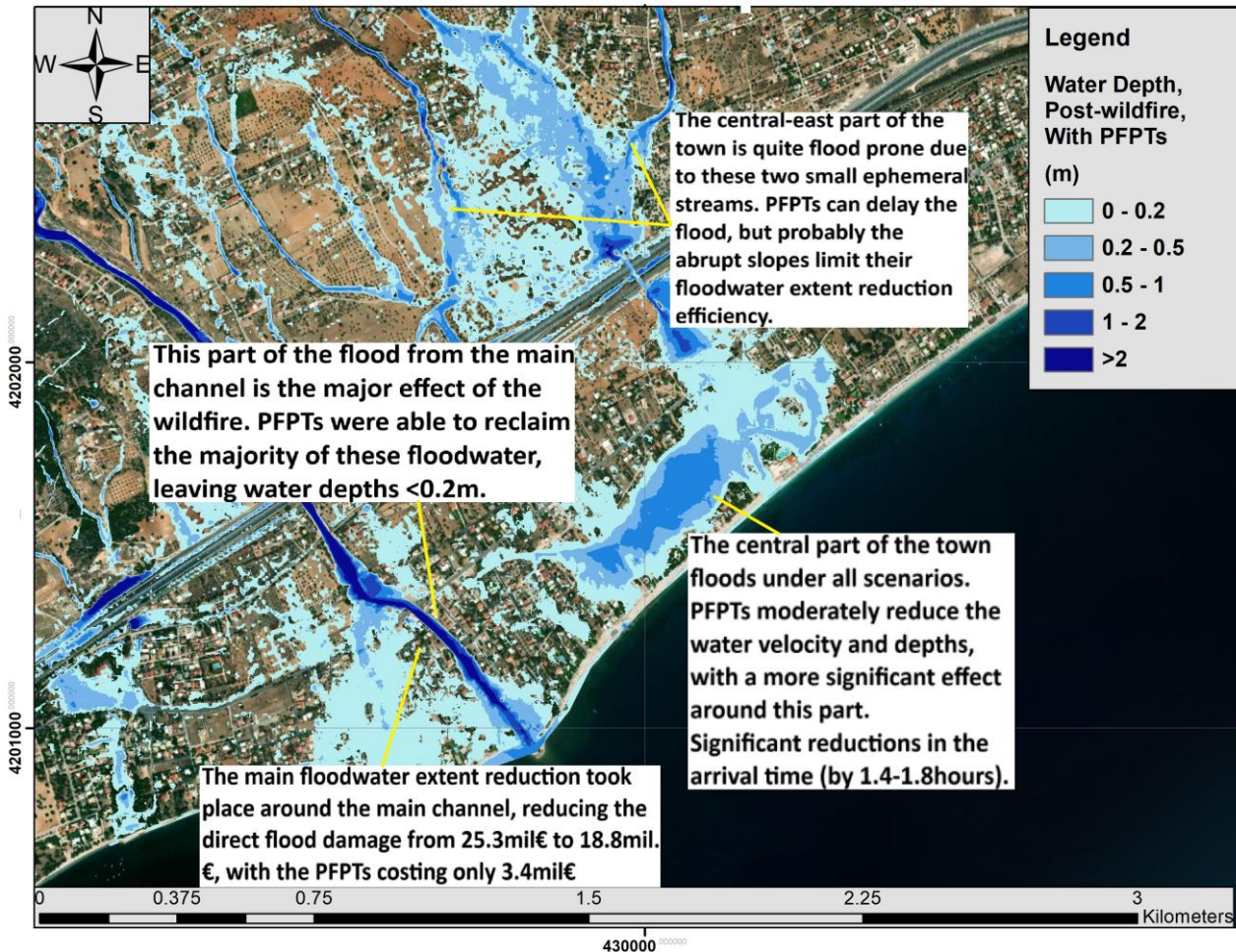
400 401 Figure 6: Summarizing the main findings on the effect of PFPTs, over the Post-wildfire With PFPTs scenario. Base-map source: © 402 Google Earth.
