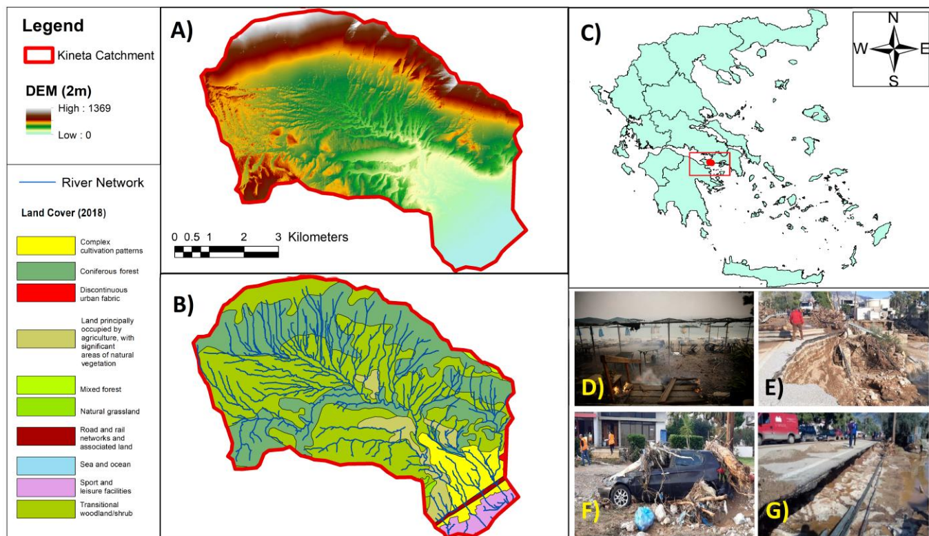
Figure 1: A) The Kineta catchment's digital elevation model (DEM). Adapted from: National Cadastre and Mapping Agency S.A. (NCMA, 2021) B) The main land cover types and the river network. C) Kineta's location in Greece (red dot). D) A picture from the wildfire of 2018, which initiated from the mountainous part of the catchment and reached the coast. F-G) Damages caused by the flood of 2019, affecting critical infrastructure and properties. Sources: (Lekkas et al., 2019; Protothema, 2019).
