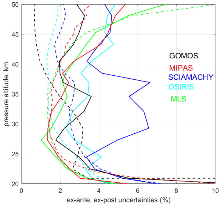
Figure 8. Ex-ante (dashed lines) and ex-post (solid lines) random uncertainty estimates for GOMOS, MIPAS, SCIAMACHY, OSIRIS and MLS in September 2007, based on the method described in Sofieva et al. (2022)
