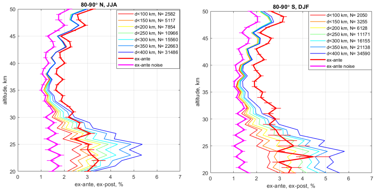
Figure 3. Colored thin curves: experimental precision estimates s_{12}/\sqrt{2} for different separation distances; thick curves with errorbars: the mean ex-ante uncertainty estimate and its standard deviation for propagated instrumental noise (magenta) and full random uncertainty (red); MIPAS self-collocations close to the North and South Poles in 2005–2011 during local summer are used.
