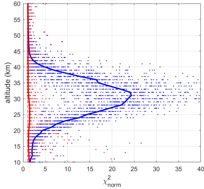
Figure 1. Adapted from (Sofieva et al., 2010): \chi_{norm}^2 in GOMOS retrievals from a set of oblique occultations of Sirius (August 2003, 66°S, obliquity angle is ~25°). Blue: random error due to residual scintillation is ignored, red: modelling errors are taken into account in the retrievals. Dots: values in individual occultations, bold lines indicate median values for the sets. The black dashed line indicates \chi_{norm}^2 = 1
