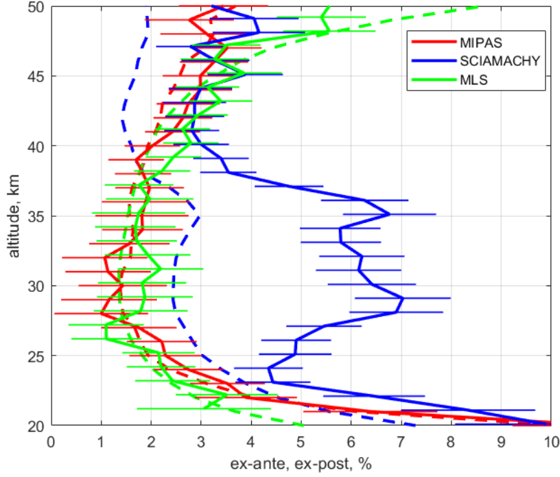
Figure 7. Dashed lines: ex-ante uncertainties; solid lines with error bars: ex-post random uncertainties estimated by the von Clarmann method. Error bars are 1-sigma uncertainties.
