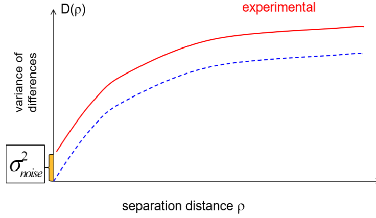
Figure 2. Reproduced from (Sofieva et al., 2021): The schematic representation of the structure function estimated from noisy measurements, \rho denotes spatio-temporal separation. Blue line: the structure function for noise-free data, red line: the structure function for experimental (noisy) data.
