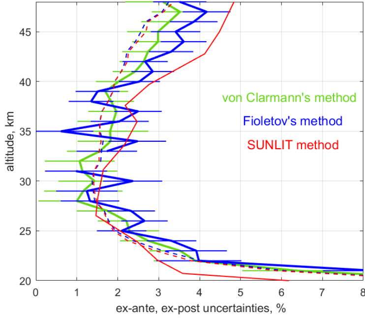
Figure 9. Uncertainty estimates for MIPAS at 20°S-20°N in 2007 by different methods. Dashed lines: ex-ante uncertainties (coinciding for Fioletov's and von Clarmann's methods), solid lines: ex-post uncertainties (%). For the SUNLIT method, data in September 2007 are used. Error bars are 1-sigma uncertainties.
