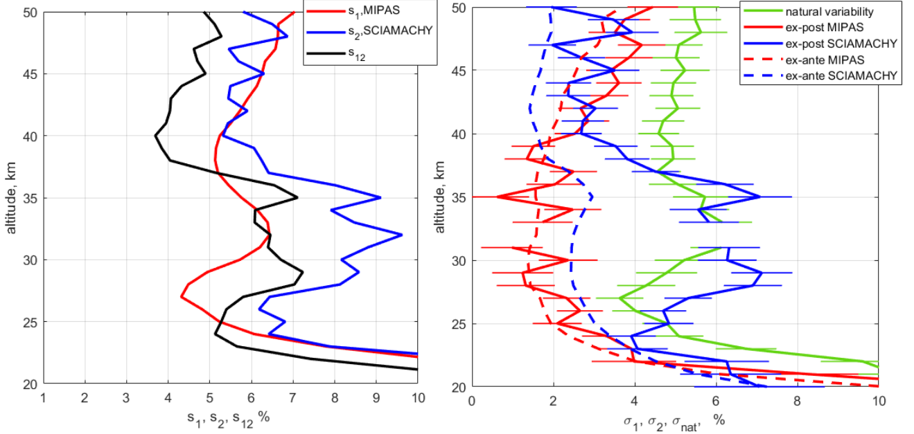
Figure 4. Application of Fioletov’s method to MIPAS and SCIAMACHY ozone datasets in 2007. Left: sample standard deviations s_1 and s_2 in collocated pairs, and the standard deviation of differences s_{12} . Right: ex-post uncertainty estimates \hat{\sigma}_1 and \hat{\sigma}_2 , and the estimate of natural variability \hat{\sigma}_{nat} with 1-sigma uncertainties (solid lines). Ex-ante uncertainty estimates are shown with dashed lines. Error bars are 1-sigma uncertainties.
