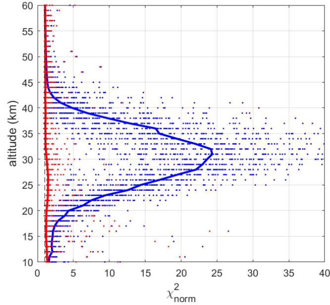
Figure 1. Adapted from (Sofieva et al., 2010): \chi_{norm}^2 in GOMOS retrievals from a set of oblique occultations of Sirius (August 2003, 66°S, obliquity angle is ~25°). Blue: random error due to residual scintillation is ignored, red: modelling errors are taken into account in the retrievals. Dots: values in individual occultations, bold lines indicate median values for the sets. The black dashed line indicates \chi_{norm}^2 = 1
