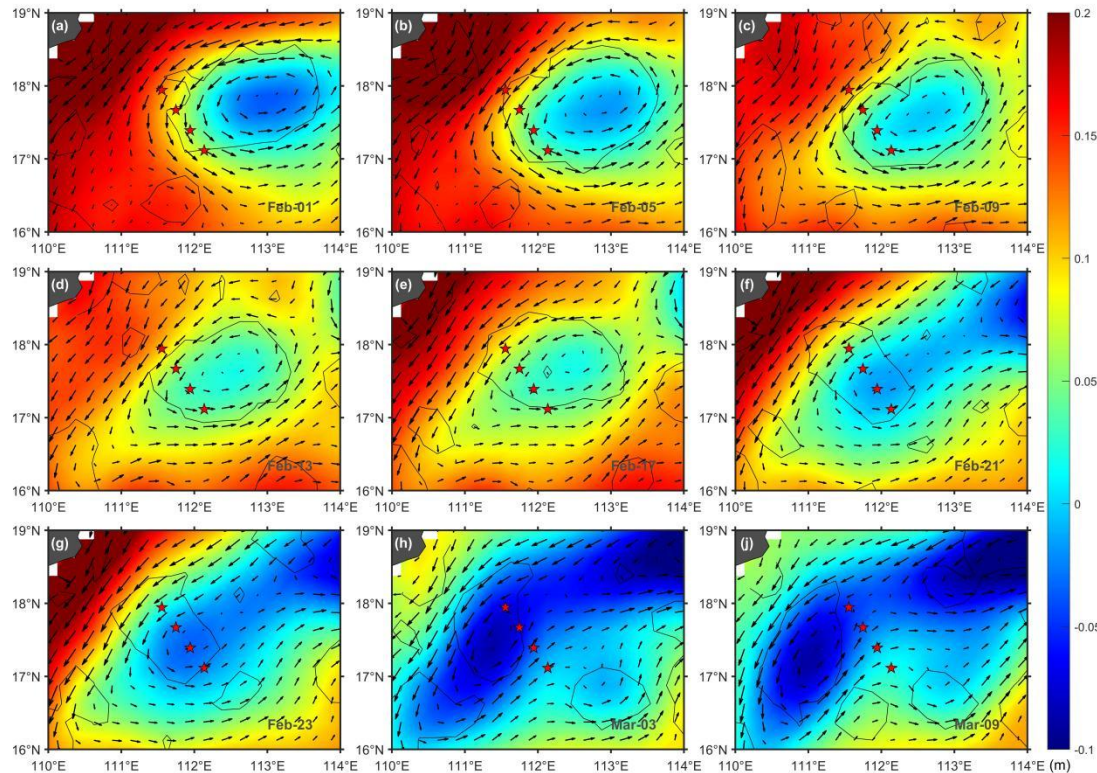
144 145 Figure 2: (a-j) The snapshot of sea level anomaly and geostrophic current vector during February 1-March 9. The 146 black line indicates the Okubo-Weiss parameters.
