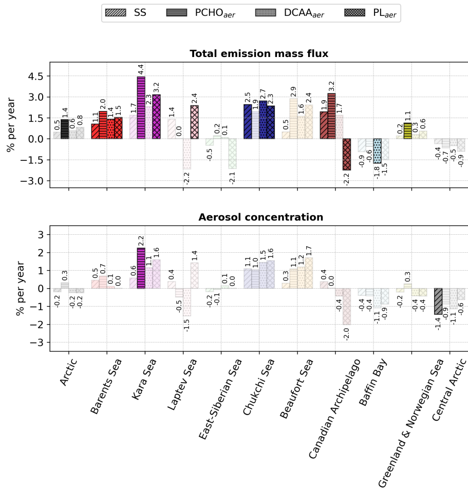
Figure G5. Bar plot of the per cent of change per year of total emission flux and near-surface mean aerosol concentration of marine species for the Arctic and subregions defined in Fig. 1 for April-May-June of the period 1990–2019. Values were calculated by normalising the slope of the trend analysis by the 30-year average value for every subregion. The values atop the bars are the corresponding percentage per year. The shaded bars represent the cases with no significant trend (Mann-Kendall test, p -value > 0.05 ).
