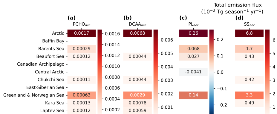
Figure H1. Heatmaps of trends over the Arctic and subregions defined in Fig. 1 for total emission mass flux of (a) \text{PCHO}_{aer} , (b) \text{DCAA}_{aer} , (c) \text{PL}_{aer} , and (d) \text{SS} simulated by ECHAM-HAM model for July-August-September of the period 1990–2019. Only regions where the trend was significant are included (Mann-Kendall test, p-value < 0.05).
