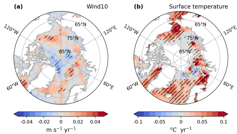
Figure G3. Arctic trends of (a) surface wind speed sea and (b) sea surface temperature (SST) for July-August-September of the simulated period 1990-2019 from ECHAM-HAM model. Only grid cells where the trends are significant (Mann-Kendall test, p\text{-value} < 0.05 ) are considered.
