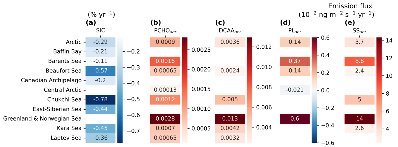
Figure 9. Heatmaps of trends over the Arctic and subregions defined in Fig. 1 for averaged (a) SIC, aerosol emission mass flux of (b) PCHO aer , (c) DCAA aer , (d) PL aer , and (e) SS simulated by ECHAM–HAM model for July–August–September of the period 1990–2019. Only regions where the trend was significant are included (Mann-Kendall test, p-value < 0.05).
