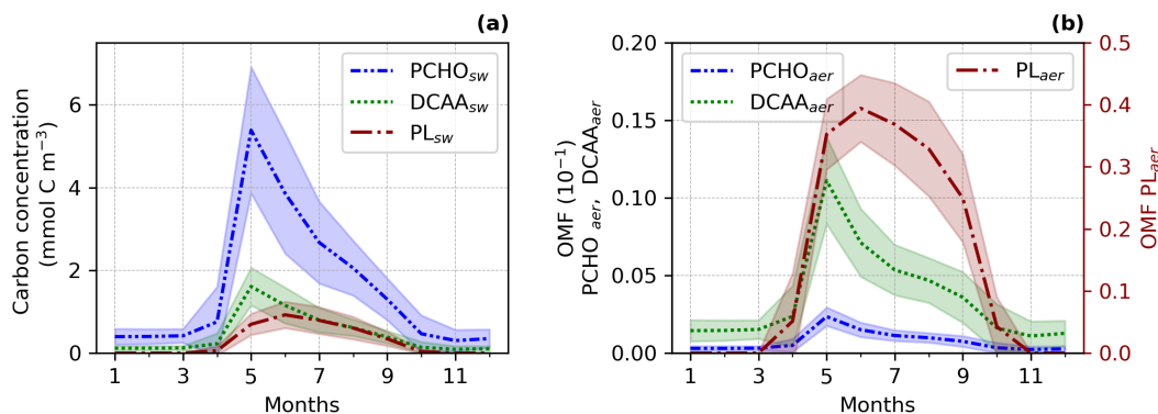
Figure 3. Seasonal climatology of (a) ocean carbon concentration for PCHO sw , DCAA sw and PL sw and, (b) offline simulated organic mass fraction (OMF) in nascent aerosol from OCEANFILMS for PCHO aer , DCAA aer and PL aer for the period 1990–2019 and sea ice free ocean conditions (SIC < 10 %; Arrigo et al., 2008) averaged over the Arctic. Values were over the Arctic circle (66 °N–90 °N) and the shaded area represents the spatial standard deviation of the long-term monthly mean.
