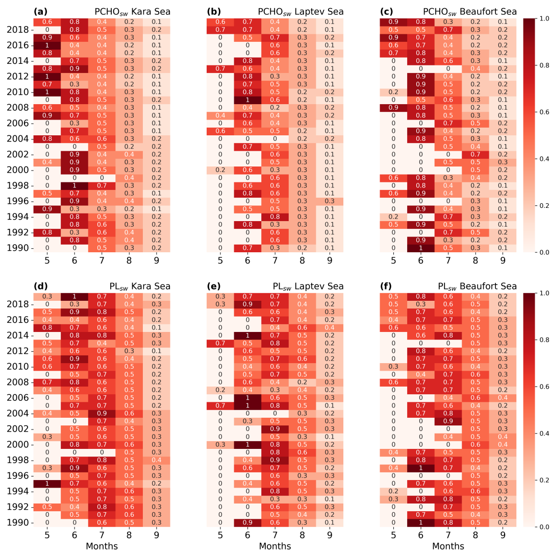
Figure C1. Annual seasonality of normalized averaged ocean biomolecule concentration for (a, b, c) PCHO sw and (d, e, f) PL sw for the (a, d) Kara, (b, e) Laptev and (c, f) Beaufort seas over the period 1990–2019 considering sea ice free ocean conditions (SIC < 10 %; Arrigo et al., 2008).
