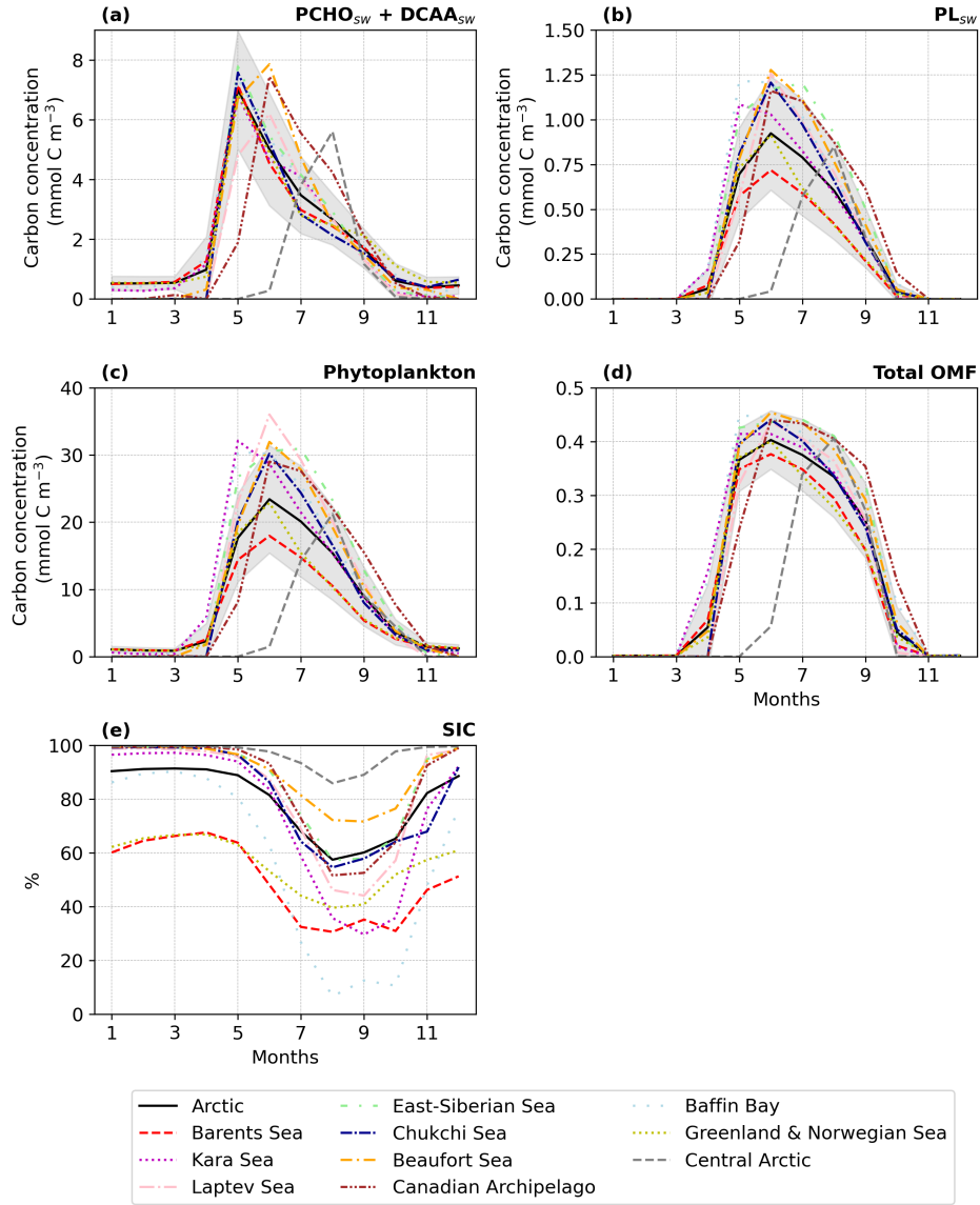
Figure B2. Seasonal climatology of (a) ocean carbon concentration of PCHO sw + DCAA sw , (b) PL sw and (c) phytoplankton, (d) total OMF with sea ice free ocean conditions (SIC < 10 %) and (e) SIC modelled by FESOM for the period 1990-2019 averaged over the Arctic Ocean (66°N – 90°N) and Arctic subregions in Fig.1.
