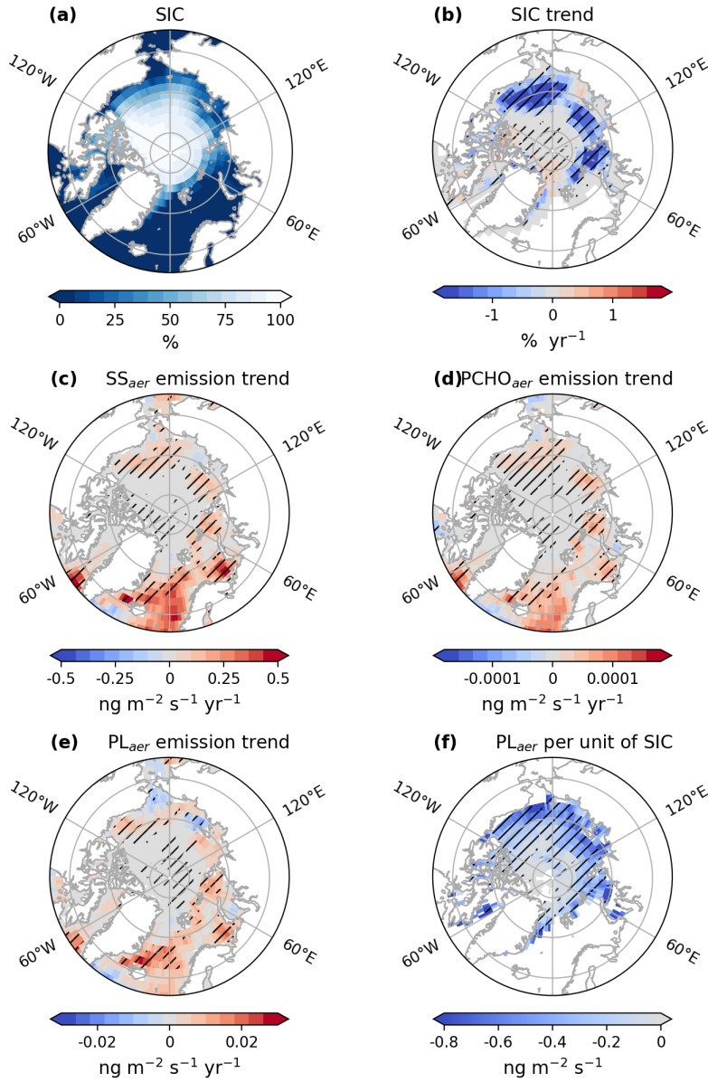
Figure 8. Maps of (a) average sea ice concentration (SIC), (b) trend of SIC, trends of emission fluxes of (c) SS, (d) PCHO aer , (e) PL aer and (f) changes of emission fluxes of PL aer per unit of SIC for SIC > 20 %, for July-August-September of the simulated period 1990-2019 by ECHAM-HAM model. The trend of PL aer per unit of sea ice was computed based on a linear regression model. The hatching indicates the areas over which trends are significant (Mann-Kendall test or t-test, p-value < 0.05).
