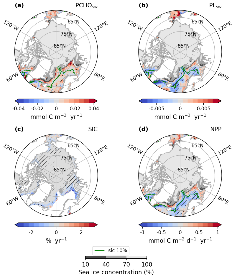
Figure G1. Arctic trends of (a) PCHO_{sw} and (b) PL_{sw} ocean concentration, (c) sea ice concentration and (d) net primary production from REcoM model for April-May-June of the simulated period 1990–2019. The hatching indicates the areas over which trends are significant (Mann-Kendall test, p\text{-value} < 0.05 ). The green contour line depicts the average season 10% sea ice concentration. The minimum seasonal SIC for the period occurred in June 2016, and it is also represented in shaded gray.
