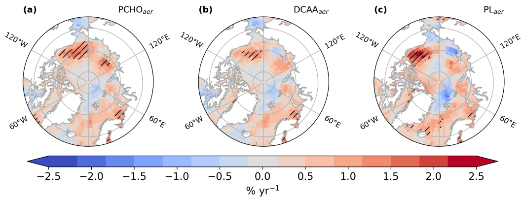
Figure 11. Maps of annual percentage variation in atmospheric burden for (a) PCHO_{aer} , (b) DCAA_{aer} and (c) PL_{aer} during July–August–September, derived from ECHAM6.3–HAM2.3 simulations covering 1990–2019. Hatched regions denote statistically significant trends (Mann–Kendall test, p\text{-value} < 0.05 ).
