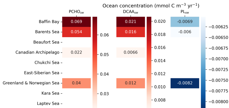
Figure G2. Absolute maximum trends for the Arctic subregions in Fig 1 of biomolecule ocean concentration for April-May-June of the period 1990–2019. Only cases where the trends are significant (Mann-Kendall test, p\text{-value} < 0.05 ) are considered. Values were obtained after applying a mask with the minimum sea ice concentration shown in Fig. G1.
