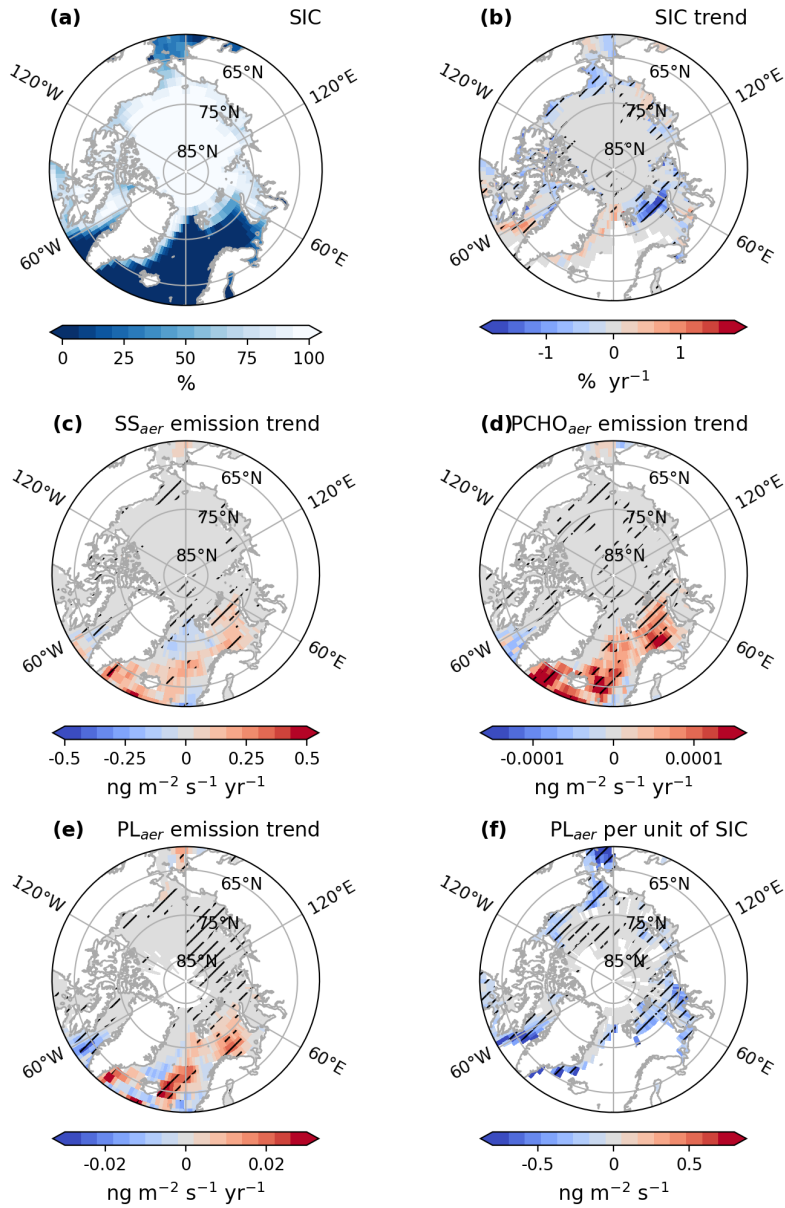
Figure G4. Maps of (a) average sea ice concentration (SIC), (b) trend of SIC, trends of emission fluxes of (c) SS, (d) PCHO aer , (e) PL aer and (f) changes of emission fluxes of PL aer per unit of SIC for SIC > 20 %, for April-May-June of the simulated period 1990-2019 by ECHAM-HAM model. The trend of PL aer per unit of sea ice was computed based on a linear regression model. The hatching indicates the areas over which trends are significant (Mann-Kendall test or t-test, p-value < 0.05).
