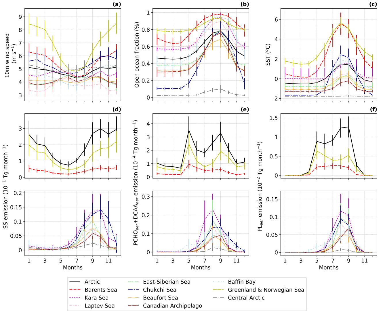
Figure 5. Seasonal climatology of (a) 10-m Wind speed, (b) Open ocean fraction, (c) SST and emission fluxes of (d) SS, (e) PCHO_{aer} + DCAA_{aer} and (f) PL_{aer} for the period 1990–2019 simulated by ECHAM-HAM model averaged over the Arctic and all seas within the Arctic Ocean (Fig. 1). Monthly emissions were obtained by summing the daily values across all grid cells in the region and then averaging over the 30-year period. The error bars indicate the multiannual standard deviation. Subregions with small emission fluxes are shown in a separate panel for better representation.
