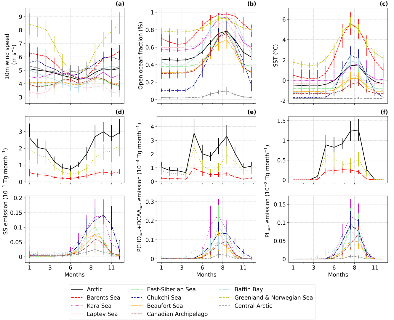
Figure 5. Seasonal climatology of (a) 10m Wind speed, (b) open ocean fraction, (c) SST and emission fluxes of (d) SS, (e) \text{PCHO}_{\text{aer}} + \text{DCAA}_{\text{aer}} and (f) \text{PL}_{\text{aer}} for the period 1990–2019 simulated by ECHAM-HAM model averaged over the Arctic and all seas within the Arctic Ocean (Fig. 1). Monthly emissions were obtained by summing the daily values across all grid cells in the region and then averaging over the 30-year period. The error bars indicate the multiannual standard deviation. Subregions with small emission fluxes are shown in a separate panel for better representation.
