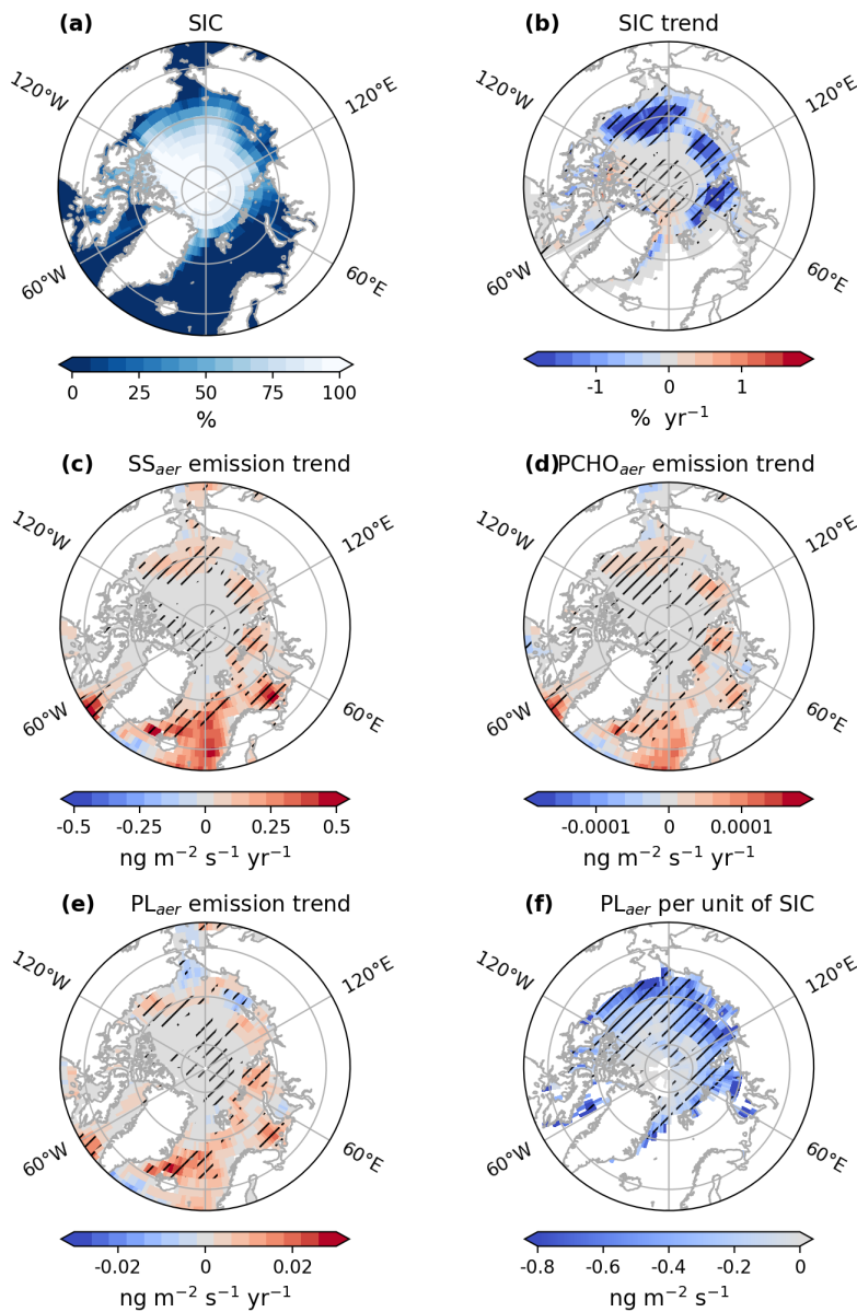
Figure 9. Maps of (a) average sea ice concentration (SIC), (b) trend of SIC, trends of emission fluxes of (c) SS, (d) \text{PCHO}_{aer} , (e) \text{PL}_{aer} and (f) changes of emission fluxes of \text{PL}_{aer} per unit of SIC for SIC > 20 %, for July-August-September of the simulated period 1990-2019 by ECHAM-HAM model. The trend of \text{PL}_{aer} per unit of sea ice was computed based on a linear regression model. The hatching indicates the areas over which trends are significant (Mann-Kendall test or t-test, p-value < 0.05).
