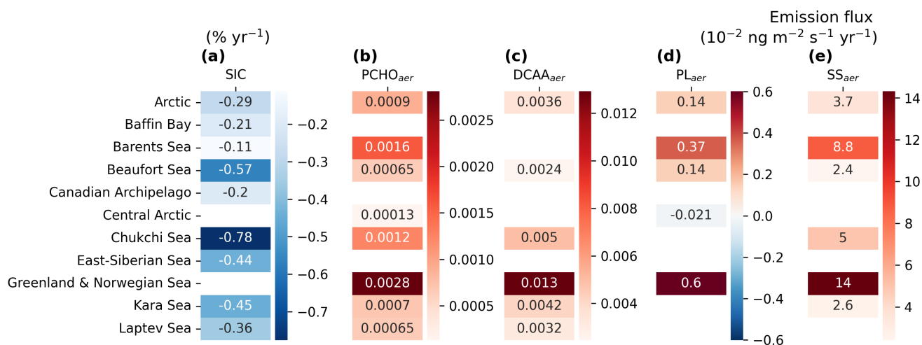
Figure 10. Heatmaps of trends averaged over the Arctic and subregions defined in Fig. 1 for average (a) SIC, aerosol emission mass flux of (b) PCHO aer , (c) DCAA aer , (d) PL aer , and (e) SS simulated by ECHAM–HAM model for July–August–September of the period 1990–2019. Only regions where the trend was significant are included (Mann-Kendall test, p-value<0.05).
