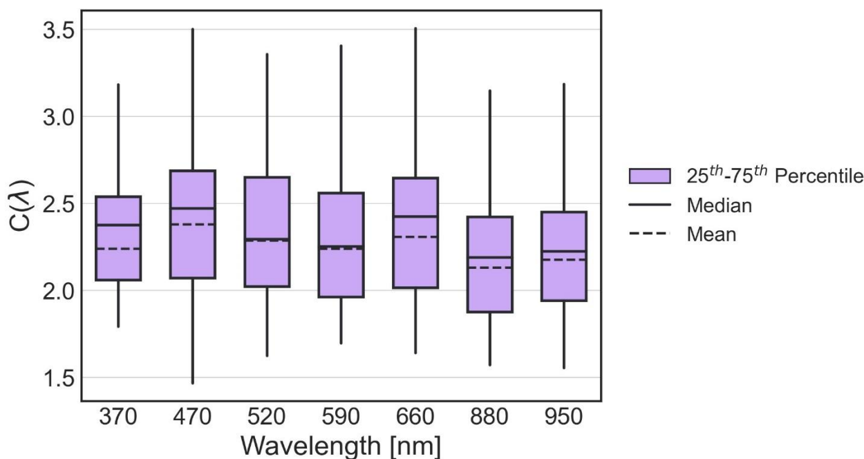
Figure 6: Boxplots describing the statistics of C values derived at each aethalometer wavelength, the 25 th – 75 th percentile range, the mean and median are reported. The MWAA was used as the reference technique for measuring the absorption coefficient.
