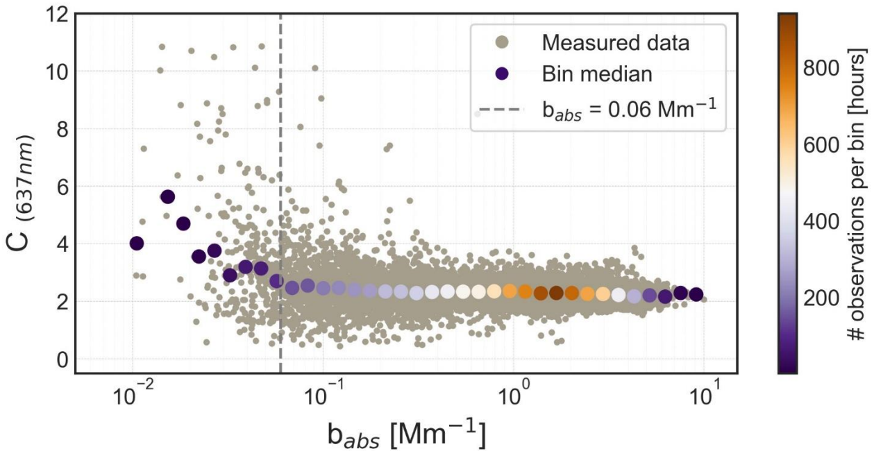
Figure 3: Scatterplot of hourly averaged C values at 637 nm as a function of the corresponding b_{abs} values measured by the MAAP at CMN. The reference technique used to measure the absorption coefficient is the MAAP. Bigger dots are used to represent the median C values in bins of b_{abs} .
