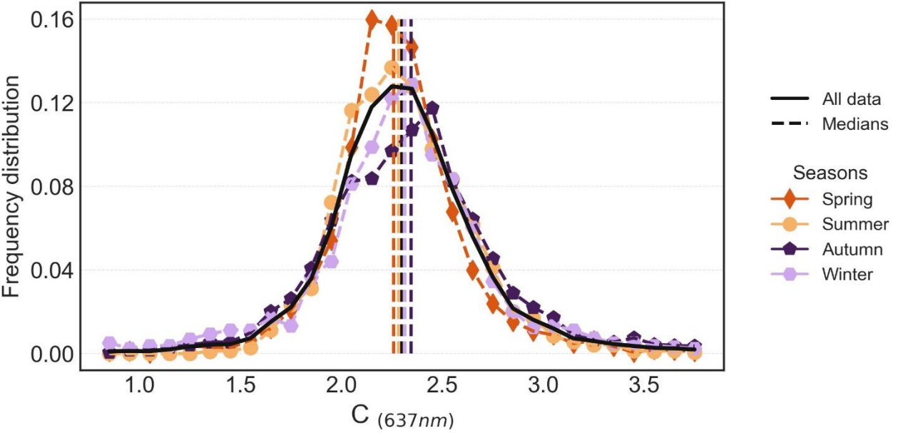
Figure 2: Histograms representing hourly averaged C values frequency distribution at 637 nm for the period July 2020 – November 2022 at CMN. The black line represents the entire period, the coloured histograms correspond to each season in the analysed period. The median values corresponding to each season are also represented as dashed vertical lines. The MAAP was used as reference technique for measuring the absorption coefficient.
