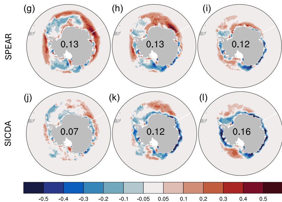
Figure 13. SIC detrended ACC, and bias on the forecast days of 1, 20, and 40 from the December-initialized reforecast experiments for SPEAR and SICDA. The skills are calculated using daily data from 1992–2017.
