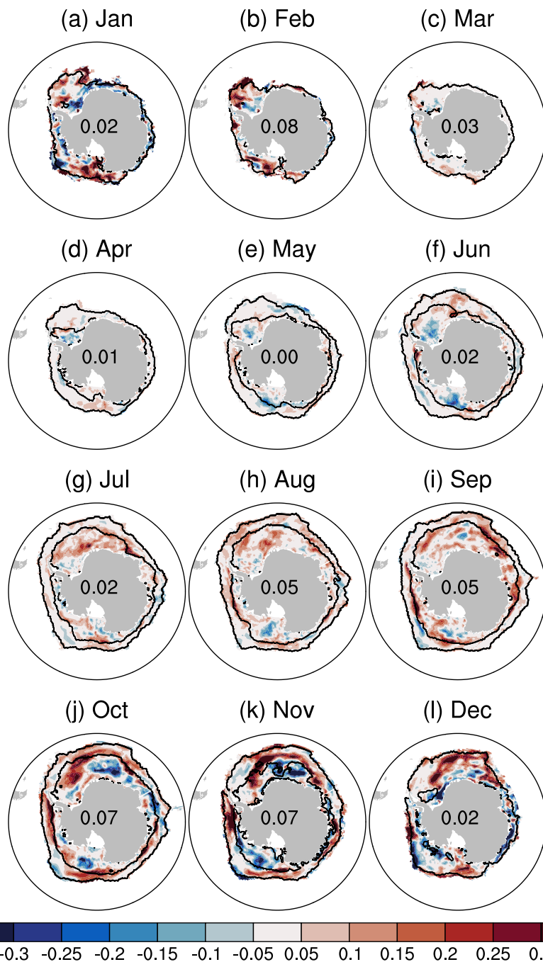
Figure 8. Difference in the 45-forecast-day 45-forecast-day mean of the detrended SIC ACC between the two reforecast experiments (SICDA - SPEAR). The black lines on each map represent the observed 10% SIC interannual variability zone. The numbers on each map are the area-weighted average of the ACC difference within the SIC variability zone.
