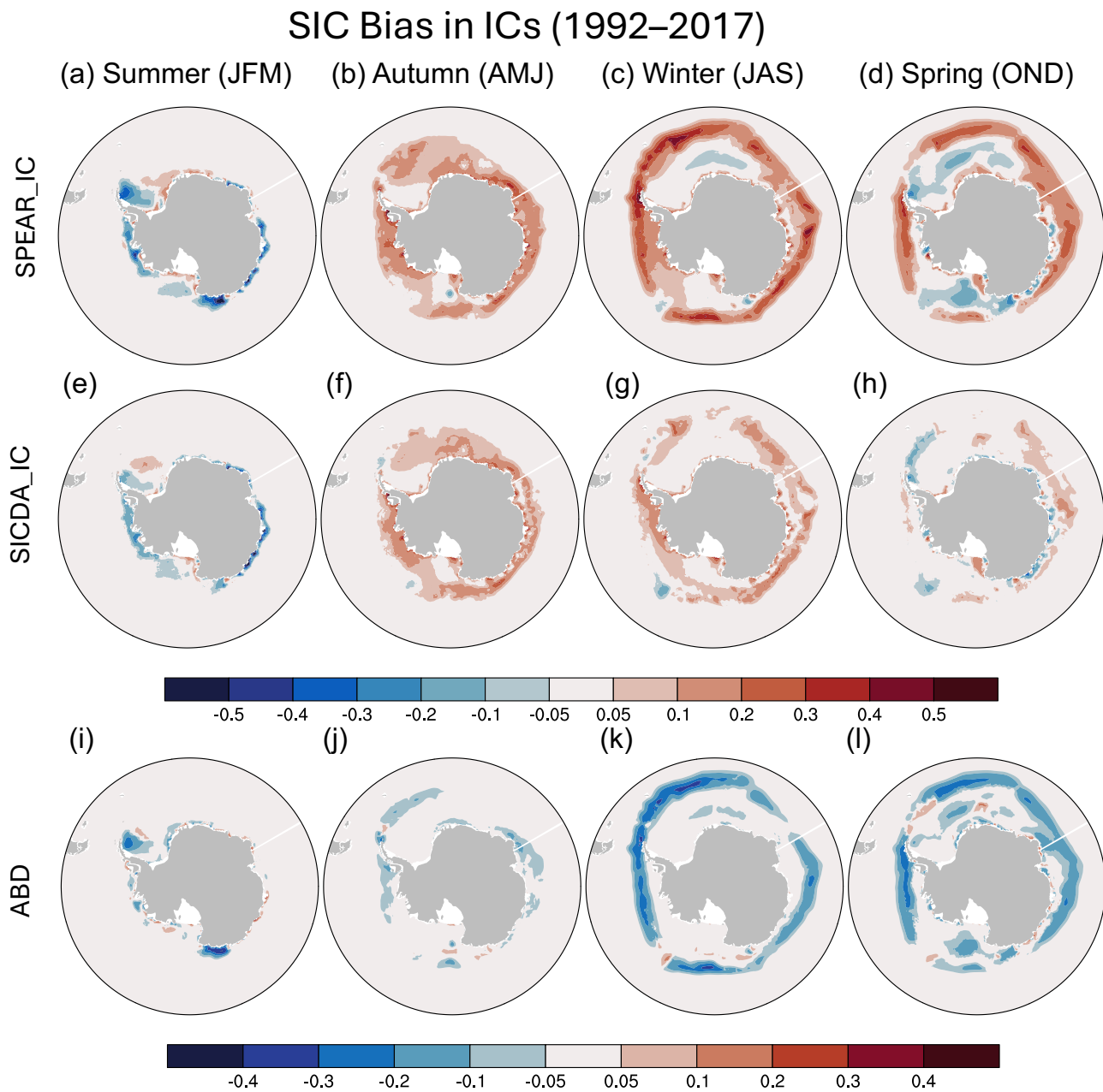
Figure 3. SIC Bias for each season for SPEAR_IC (a–d), and SICDA_IC and (e–h), and their absolute bias difference (ABD; \text{SICDA\_IC} - \text{SPEAR\_IC} ; i–l). The biases are calculated against NSIDC SIC observations from 1992–2017.
