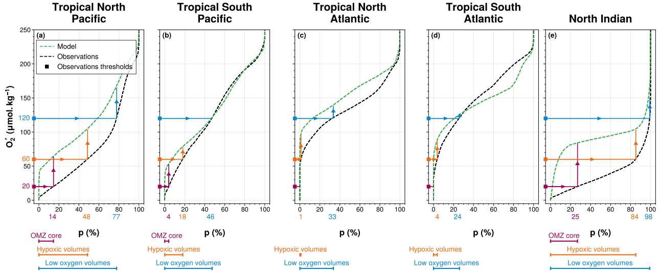
Figure 4. OMZ volume definition in IPSL-CM6A-LR simulations. For each of the five OMZ spatial boxes, the volume percentile p is computed as a function of O_2 threshold using (black dashed lines) the World Ocean Atlas database and (green dashed lines) the IPSL-CM6A-LR Large Ensemble inter-member mean. The three thresholds ((purple) 20\mu\text{mol.kg}^{-1} , (orange) 60\mu\text{mol.kg}^{-1} and (blue) 120\mu\text{mol.kg}^{-1} ) define (coloured bands) the three volume percentiles of interest for each OMZ spatial box in WOA: (purple) OMZ Core, (orange) Hypoxic volumes and (blue) Low-oxygen volumes (Table 1). These percentiles are then used to compute the corresponding OMZ volumes in the IPSL-CM6A-LR simulations (arrowed lines).
