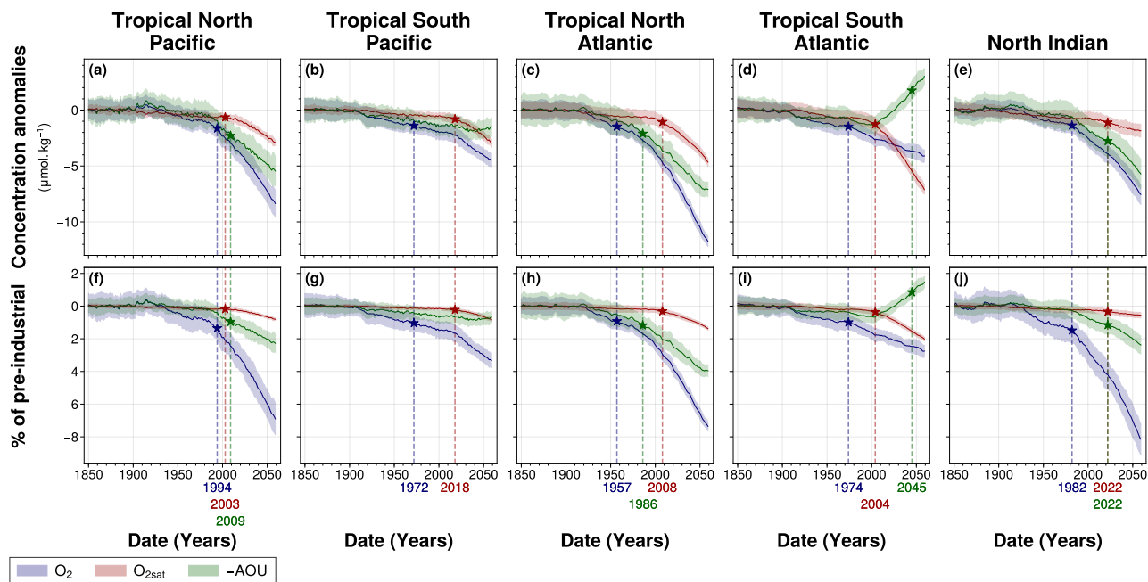
Figure 7. Time of emergence of 100 – 1000m spatial mean concentrations of (blue) O_2 , (red) O_{2sat} and (green) -AOU in the IPSL Large Ensemble for (columns) each OMZ box. The time of emergence (indicated by the star symbol) is defined as the point at which (first row) the mean concentration anomalies, and (second row) the percentage of pre-industrial concentrations, averaged across the Large Ensemble, exceed their respective (coloured areas) standard deviations within the Large Ensemble.
