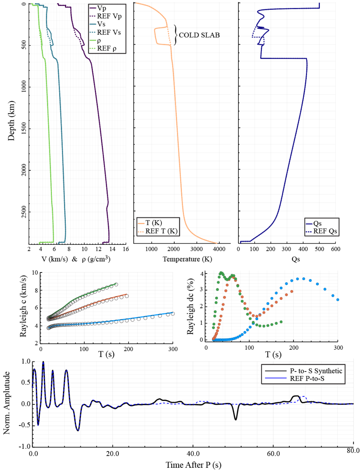
Figure 8: Example 2 showing the effect of a cold slab-like feature plunging into the transition zone. On the top: the left panel show the V_p , V_s and \rho profiles with depth (solid lines are the computed parameters and dashed ones are the PREM values), in the center we show the temperature profile with ( T ) and without (Ref T ), and on the right the attenuation profile with ( Q_s ) and without the slab ( Q_s Ref). On the center of the figure we present: on the left the dispersion curves of the model with (solid lines) and without (circles) the slab for the fundamental mode (blue) and the 1st (orange) and second (green) overtones. Anomalies between both are presented in the right panel. At the bottom P-to-S RF with (black) and without (blue) are shown. Notice that, except for the first panel, Ref is the reference model without anomalies (see text for details).
