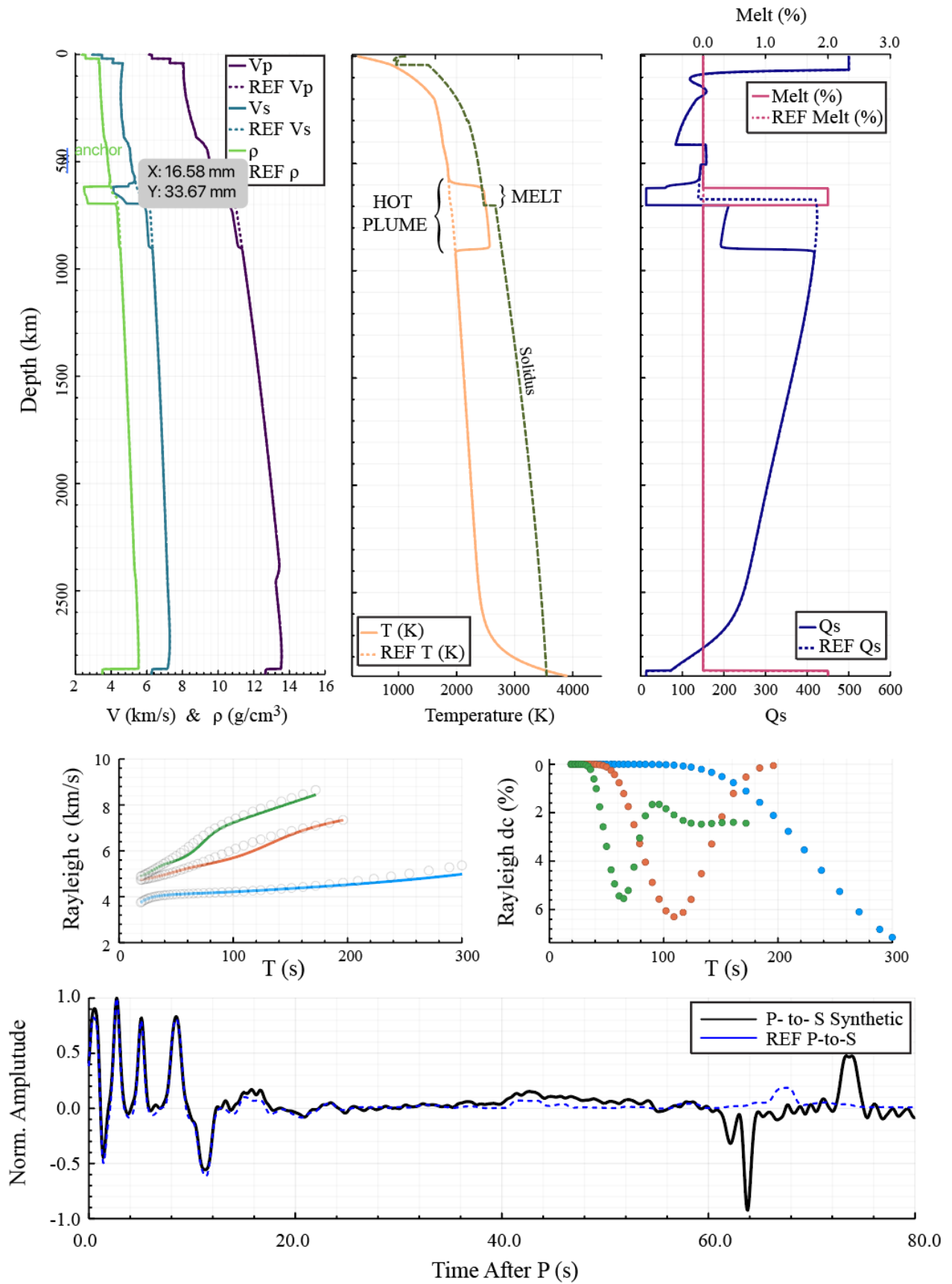
Figure 9: Example 3 showing the effect of a hot plume-like feature entering the transition zone from below. Panels are in the same configuration as in Fig. 8, but in this case we add the melt curve to the top right plot.
