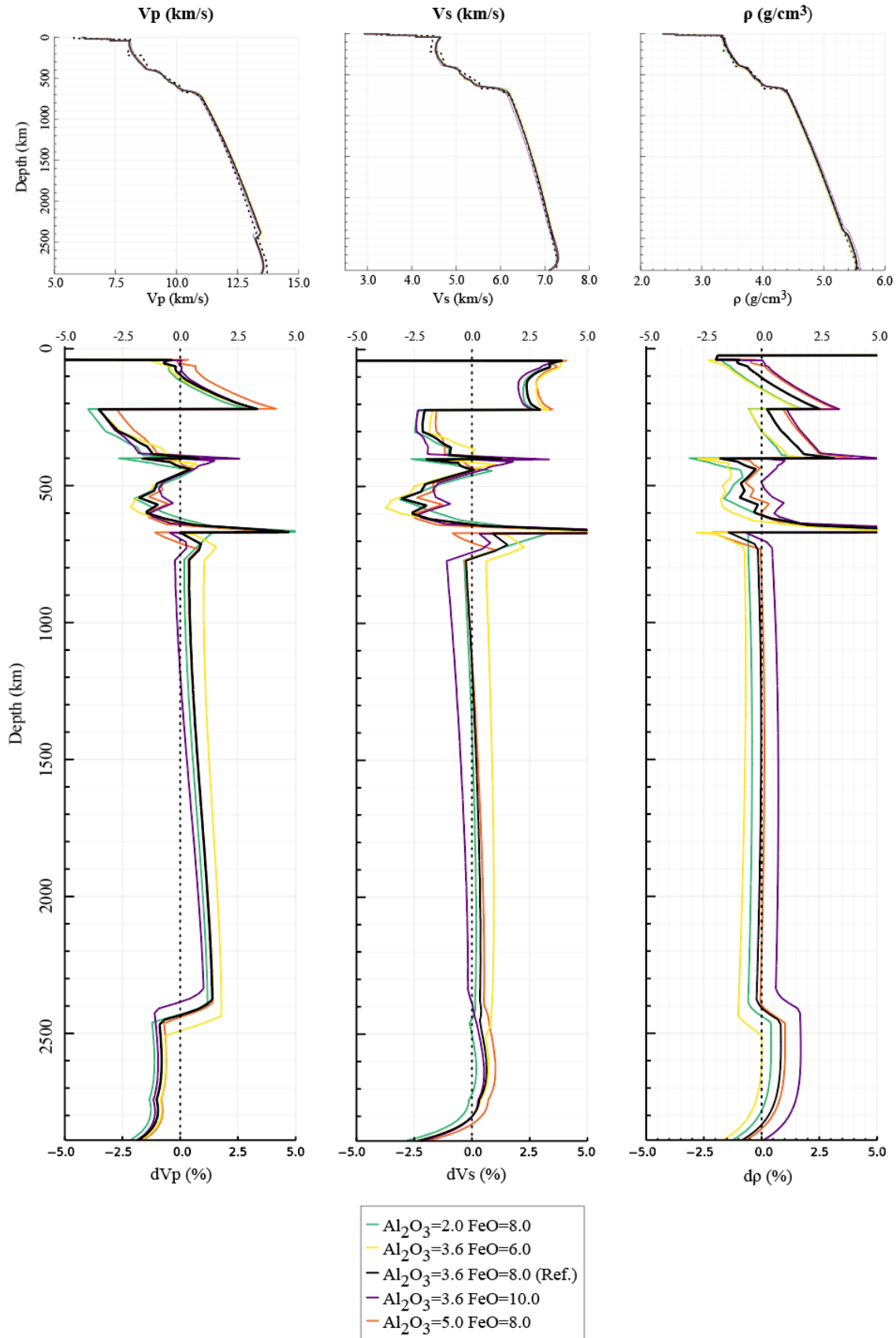
Figure 7: Example 1. Comparison between the results of a constant composition mantle in TCSEIS-1D (solid lines) and the PREM model (dashed). Here we have tested several compositions to show how large V_p , V_s and \rho anomalies can arise from extreme values of \text{Al}_2\text{O}_3 and \text{FeO} . Top panels show the comparison in absolute V_p , V_s and \rho values, while the bottom panel shows anomalies with respect to PREM. In the bottom panel, crustal anomalies have been deleted from the presentation as they are too large since PREM has a poorly estimated crust.
