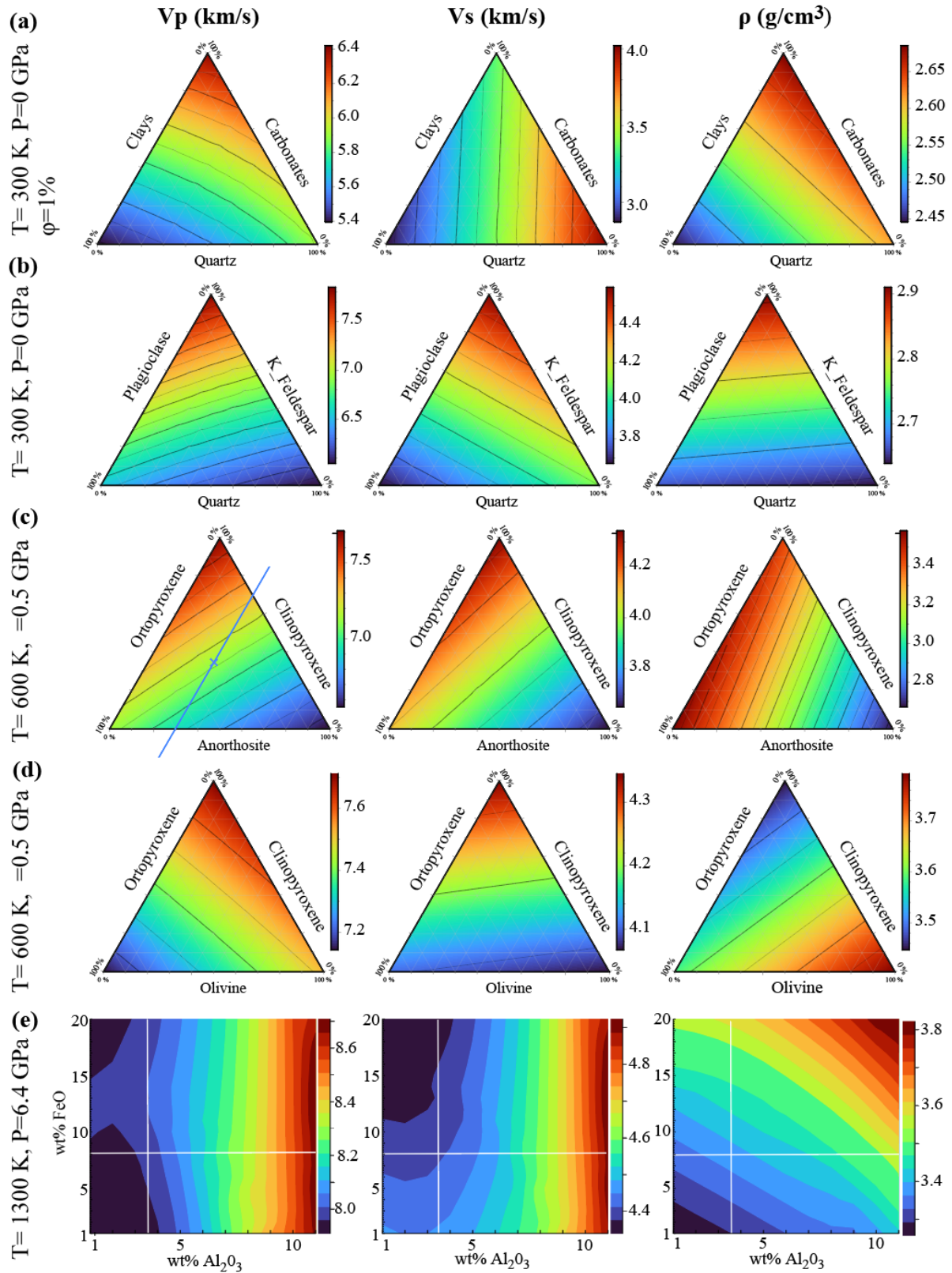
Figure 2: Examples of compressional wavespeed (Vp), shear wavespeed (Vs) and density ( \rho ) variations for: (a) sedimentary, (b) igneous felsic, (c) igneous mafic, (d) igneous ultramafic and (e) mantle rocks as a function of temperature (T), pressure (P), composition and porosity (for sedimentary rocks). All color scales are similar for ease of comparison. In sedimentary rocks (a) carbonates have the higher Vp and \rho . For felsic rocks, with higher percentage of quartz, Vp and \rho becomes higher, while Vs becomes higher with the increase of plagioclase. Also, lower values of all three properties are associated with higher percentage of K-feldspar. For mafic rocks, all properties increase with the percentage of anorthosite and decrease with the percentage of clinopyroxene. Unlike felsic or mafic rocks, in ultramafics, each mineral dominates the decrease of a different property. On (e) the cross marks the average mantle composition.
