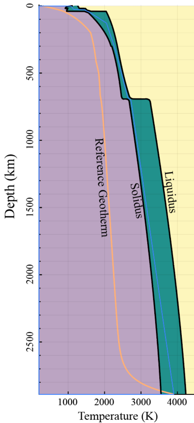
Figure 4: Solidus and liquidus curves from the entire crust and mantle. Solidus by: Gerya (2019), Katz et al. (2003), Herzberg et al (2000) and Fu et al. (2018). Liquidus by: Gerya (2019), Litasov and Ohtani (2002) and Fu et al. (2018). See text for details.
