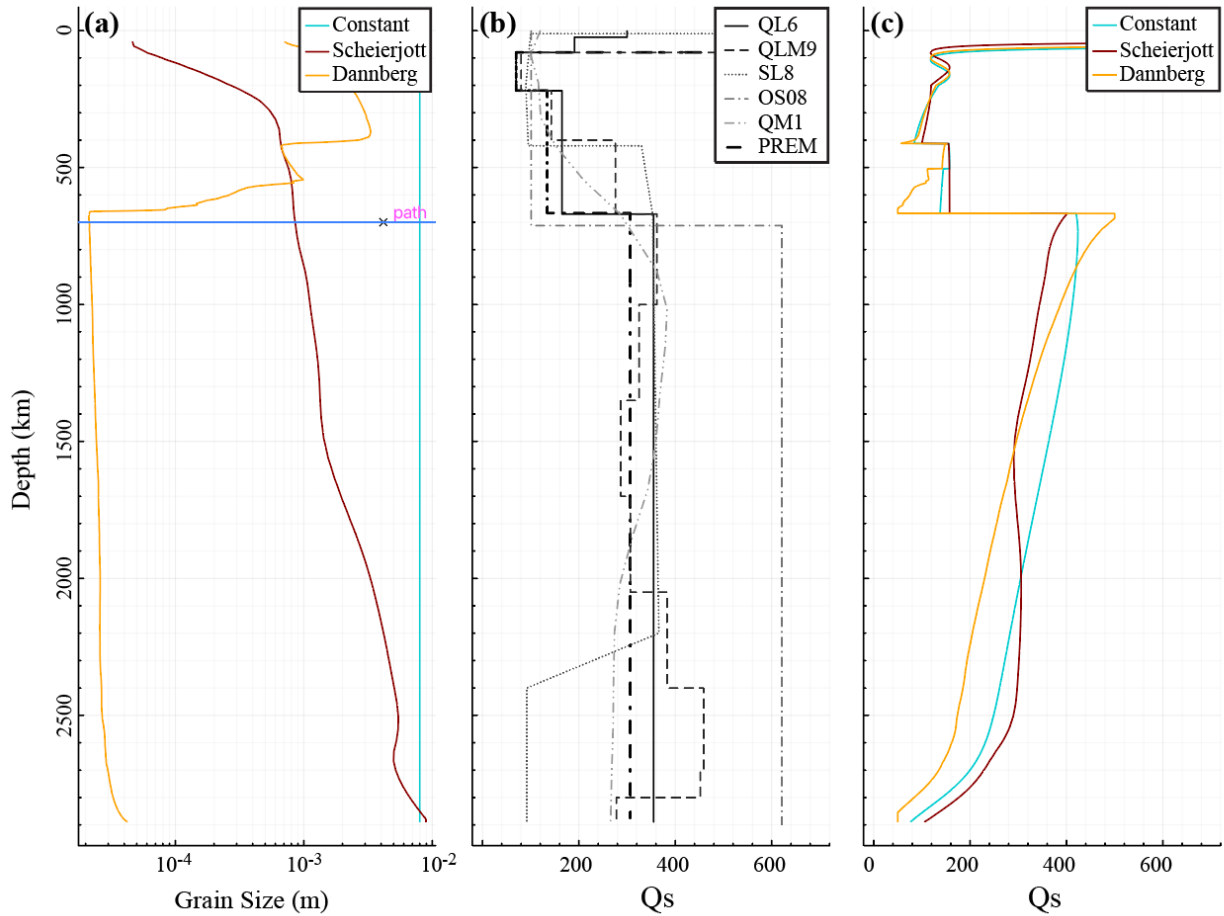
Figure 3: (a) Grain size variation with depth for the 3 models included in the code: Constant (a constant value of 10^{-2} m), Schierjott (the grain size variations estimated by Schierjott et al., 2020) and Dannberg (the grain size variations estimated by Dannberg et al., 2017). (b) Several 1D radial models of Q_s for the whole mantle: SL8 (Anderson and Hart, 1978), QM1 (Widmer et al., 1991), QL6 (Durek and Ekstrom, 1996), QLM9 (Lawrence and Wyession, 2006), QOS08 (Oki and Shearer, 2008), PREM (Dziewonski and Anderson, 1981). (c) Q_s computed from the Burgers model of linear viscoelasticity (Jackson and Faul, 2010). The Constant and Schierjott models produce the closest fit to the radial models.
