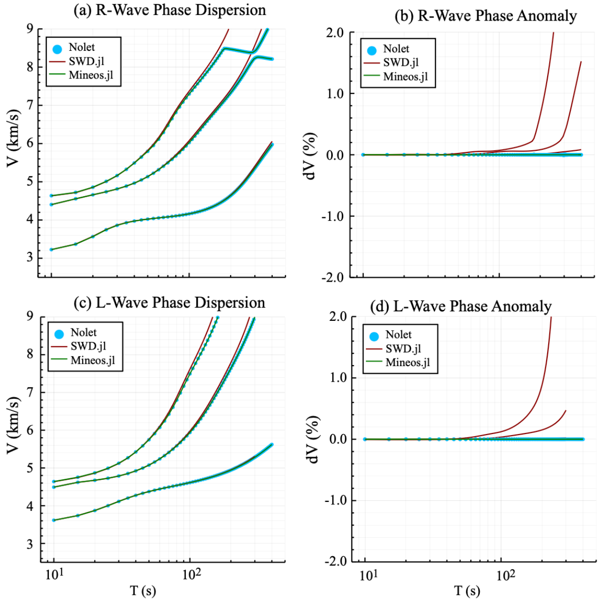
Figure 5: Comparison between surface wave dispersion curves computed by SWD.jl (red, the main TCSEIS-1D dispersion engine), Mineos (green, Masters et al., 2011) and the exact solution (blue circles marked as Nolet).
