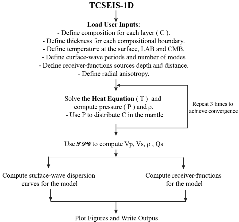
Figure 1. Schematic workflow of the TCSEIS-1D algorithm. User-defined inputs include layer composition, thickness of compositional boundaries, temperature at the surface, LAB and CMB, surface-wave periods and number of modes, receiver-function source depth and epicentral distance, and radial anisotropy. The code iteratively solves the heat equation to obtain the temperature profile, from which pressure and density are computed and used to redistribute mantle composition until convergence is achieved. Thermodynamic properties are then used to calculate seismic velocities ( V_p , V_s ), density ( \rho ), and attenuation ( Q_s ). The final 1-D model is used to compute surface-wave dispersion curves and receiver functions, followed by visualization and output of all model results.
