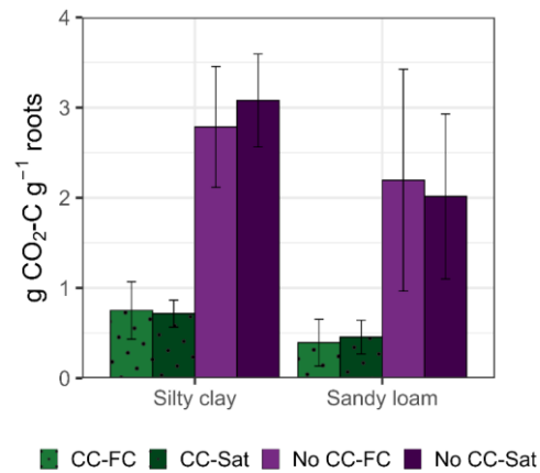
Figure S3. Off-season (beginning of the water treatment until the end of experiment) cumulative CO 2 efflux per g dry roots (mean±sd, n=4) in the top 20 cm soil layer. The g roots g -1 soil was multiplied with soil bulk density and the depth (20 cm) of the soil layer. For a description of the root washing methodology, the reader is referred to the publication by Kronberg et al. (2024).
