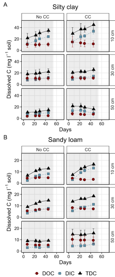
Figure S2. Timeseries of dissolved organic carbon (DOC), inorganic carbon (DIC) and total dissolved carbon (TDC) as mg C l -1 soil (mean±sd, n=1-3) during (shaded area) waterlogging in silty clay (A) and sandy loam (B) soil profiles with and without cover crops (No CC = No cover crops, CC = Cover crops) in cycle three. Days on the x-axis represent the days since the beginning of excess irrigation/waterlogging. Note the differing scales on y-axis in the two soils.
