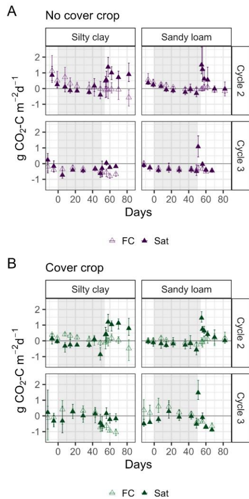
Figure S1. Residual CO 2 flux (g CO 2 -C m -2 d -1 ) from the empirical temperature and WFPS dependency model in cycle two and three in the two water treatment groups (FC=below FC, Sat=Saturation) both without (A) and with the cover crop (B). Model fitting was done separately for the two plant treatment groups (No cover crop, Cover crop) and soils (silty clay, sandy loam). The gray shaded area represents the duration of the water treatment.
