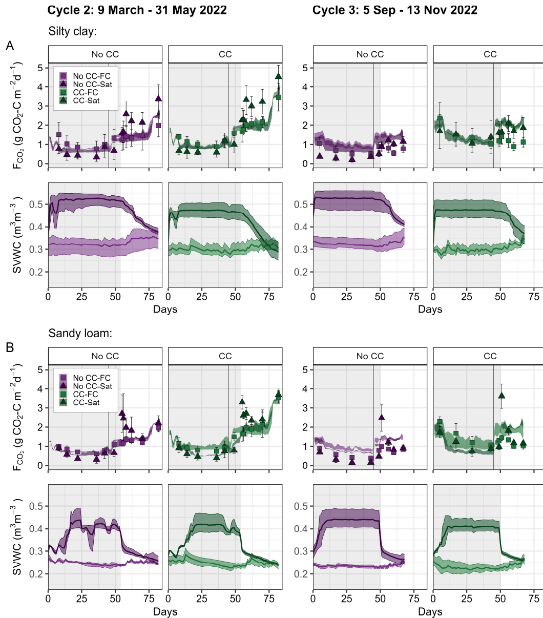
330 Figure 2. Measured (mean \pm standard deviation, n=4 ) and modelled (shaded ribbons, range, n=3 ) \text{CO}_2 efflux and soil volumetric water content at 10 cm depth (SWWC, mean \pm standard deviation, n=3 ) during and after waterlogging in A. silty clay and B. sandy loam soil during study cycles two and three CC, Cover crop; No CC, No cover crop; FC, < 70\% field capacity; Sat, Water saturation). The gray shaded area represents the duration of the waterlogging event and the vertical solid line the day when the soil temperature was increased from 5 ^\circ\text{C} to 10 ^\circ\text{C} for simulated spring. The x-axis represents the number 335 of days since the onset of the respective waterlogging event.
