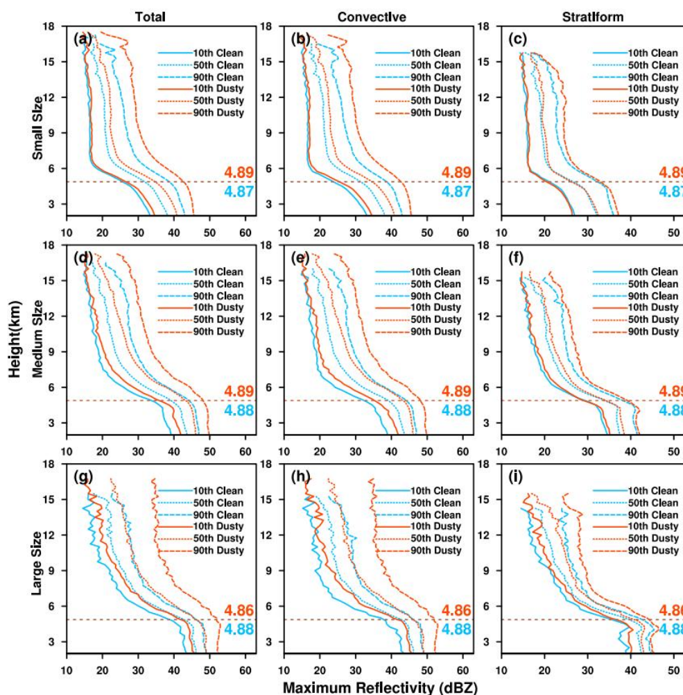
260 Figure 6. Vertical profiles of the 10th, 50th, and 90th percentiles of PS maximum radar reflectivity for total, convective and stratiform precipitation of small-sized (upper row), medium-sized (middle row), and large-sized (bottom row) PSs under clean and dusty conditions. The horizontal dashed lines show the freezing level with values labeled.
