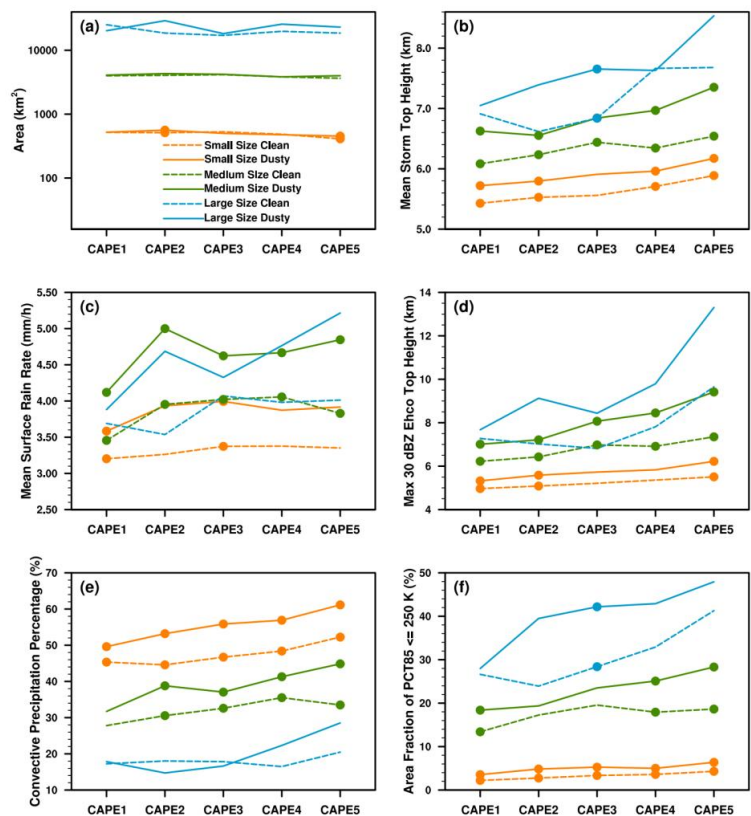
Figure 8. Variations in PS properties, including (a) area (km 2 ), (b) mean storm top height (km), (c) mean surface rain rate (mm/h), (d) maximum 30 dBZ echo top height (km), (e) convective precipitation percentage (%) and (f) area fraction of PCT85 ≤ 250 K (%), as a function of CAPE, for different sizes of PSs under clean and dusty conditions. The orange, green, and blue lines represent small-, medium- and large-sized PSs, respectively. The dashed and solid lines represent clean and dusty conditions, respectively. The circular marker indicates that the difference between clean and dusty conditions is statistically significant at the 95% confidence level using a Student's t-test.
