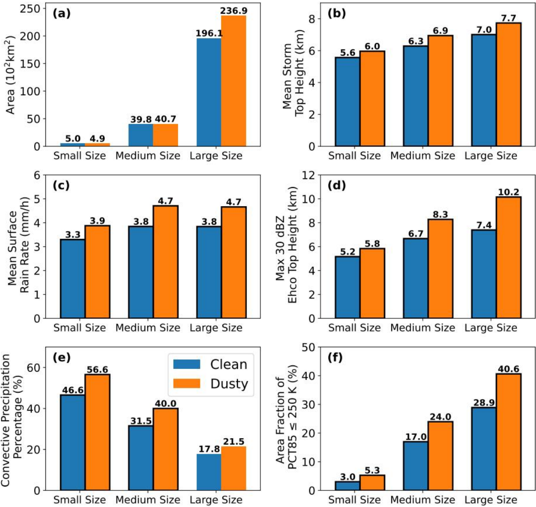
205 Figure 3. The averages of general characteristics of PSs of different sizes, including (a) area ( \text{km}^2 ), (b) mean storm top height (km), (c) mean surface rain rate (mm/h), (d) maximum 30 dBZ echo top height (km), (e) convective precipitation percentage (%) and (f) area fraction of PCT_{85} \leq 250 K (%) under clean and dusty conditions. The average values of these properties are labeled on the data bars. The black border around the data bar indicates that the difference between clean and dusty conditions is statistically significant at the 95% confidence level using a 210 Student's t-test.
