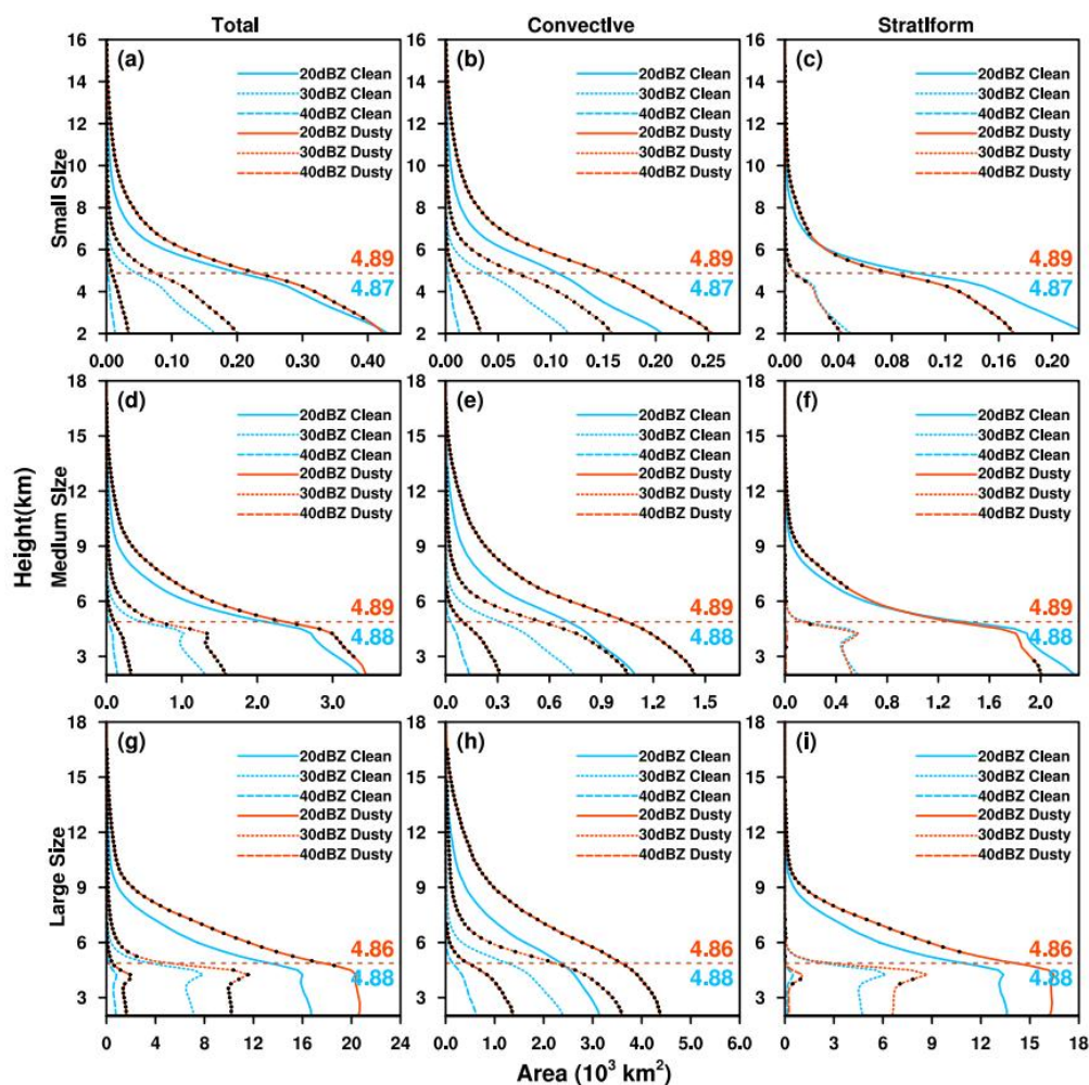
255 Figure 5. The mean vertical profiles of 20 dBZ, 30 dBZ and 40 dBZ areas for total, convective and stratiform precipitation of small-sized (upper row), medium-sized (middle row), and large-sized (bottom row) PSs under clean and dusty conditions. The black dot on the red line indicates that the difference between clean and dusty conditions is statistically significant at the 95% confidence level using a Student's t-test. The horizontal dashed lines show the freezing level with values labeled.
