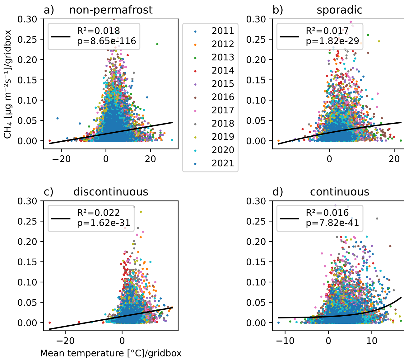
Figure A5. Grid-based melting-season-posterior melt period methane emissions and the mean temperature in the four permafrost zones; a) non-permafrost, b) sporadic, c) discontinuous, and d) continuous permafrost. Grid-cells-grid cells with negative emission rate were masked out. R^2 and p in the legends are the coefficient of determination and p -values of the slopes from linear regression fit, indicating statistical significance of the coefficient of determination.
