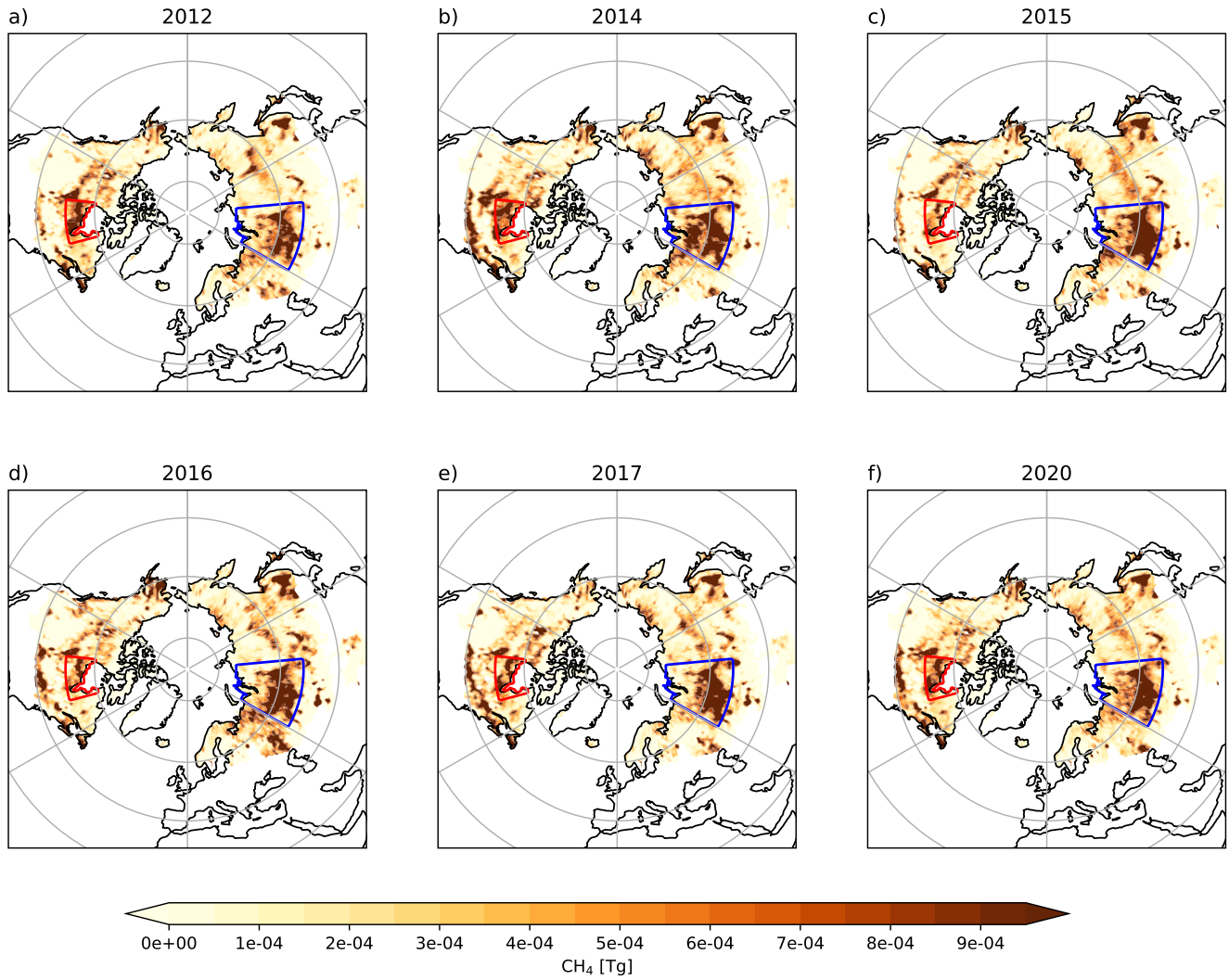
Figure A6. Region-based posterior emission maps of the melting season-melt period in the years that had some of the highest emissions in the Hudson Bay lowlands and Western Siberian lowlands. Hudson Bay lowlands have been outlined with red borders, and Western Siberian lowlands with blue borders.
