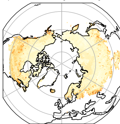
b) Start date [max-min]
