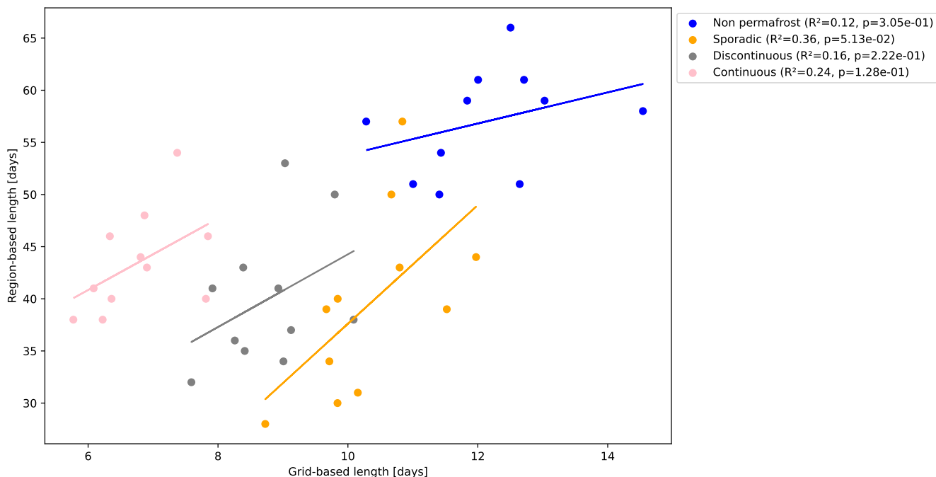
Figure A2. Relationship between grid-based and region-based melting seasons/melt periods in 2011-2021 . R^2 and p in the legends are the coefficient of determination and p -values of the slopes from linear regression fit, indicating statistical significance of the coefficient of determination.
