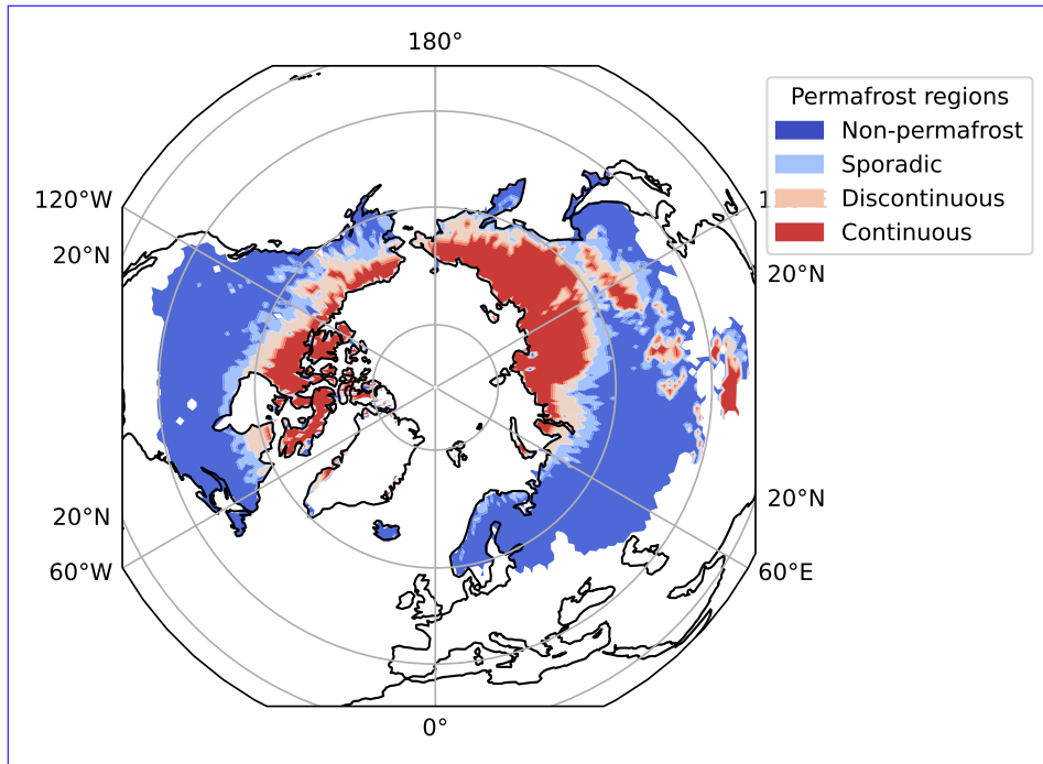
Figure 1. Extents of the four permafrost zones in 1° × 1° resolution.
