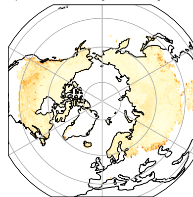
c) End date [max-min]
