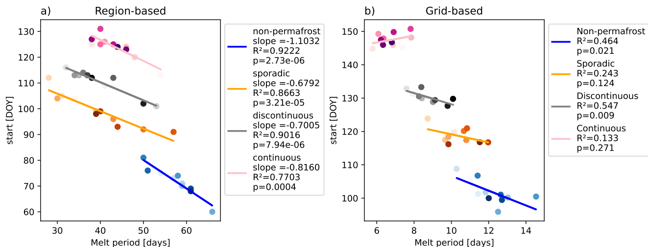
Figure A3. Relationship between region-based melt period and its' starting day (a) and grid-based melt period and its' average starting day (b) melting seasons in 2011-2021 . R^2 and p in the legends are the coefficient of determination and p -values of the slopes from linear regression fit, indicating statistical significance of the coefficient of determination.
