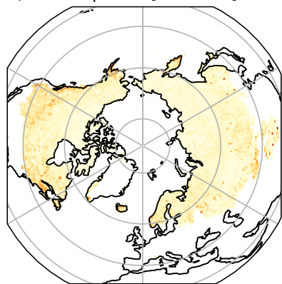
a) Melt period [max-min]
