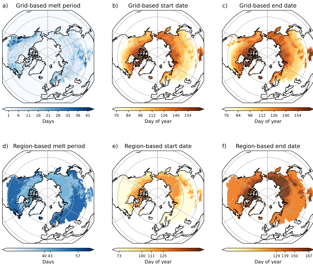
Figure 3. Grid-based (figures a,b and c) and region-based (figures d,e and f) average length, start day, and end day of the melting season-melt period in the northern high latitudes, averaged over 2011–2021. Notice the different color-range in the melting season-melt period figures on the left side (a and d). In the region-based figures, only the illustrated length, start and end days are ticked on the color-bar. The color range in the start and end day figures are the same in the grid- and region-based figures.
