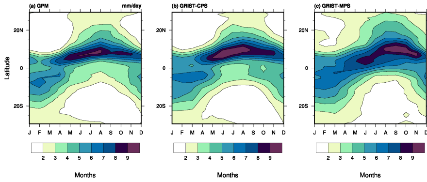
Figure 5. Seasonal evolution of tropical precipitation from 2001-2006 for observation from (a) GPM, (b) GRIST-CPS, and (c) GRIST-MPS (unit: mm/day).
