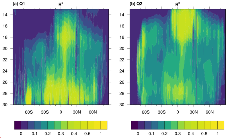
Figure 2. Offline skill of the coefficient of determination ( R^2 ) for Q_1 and Q_2 , as functions of latitude and model level. This validation is based on an independent GSRM simulation dataset out of the 80-day simulation samples.
