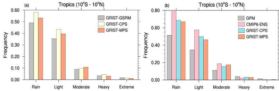
Figure 7. (a) The frequency distributions of tropical daily precipitation corresponding to the 80day-GSRM period, obtained from GSRM (gray boxes), GRIST-CPS (yellow boxes) and GRIST-MPS (orange boxes). (b) As in (a) but for precipitation frequency from 2001-2006, obtained from GPM (gray boxes), 11 CMIP6 models ensemble mean (CMIP6-ENS; pink boxes), GRIST-CPS (blue boxes) and GRIST-MPS (orange boxes).
