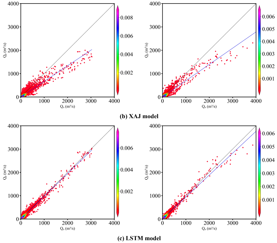
Figure 5: Scatter plots of observed ( Q_o ) and simulated ( Q_p ) flow discharges by three models in the Lushui River basin. The color bar represents the density of the scatter distribution. The denser the scatter distribution, the higher the corresponding density value in color.
