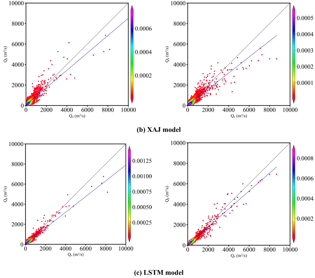
Figure 6: Scatter plots of observed ( Q_o ) and simulated ( Q_p ) flow discharge by three models in the Qingjiang River basin. The color bar represents the density of the scatter distribution. The denser the scatter distribution, the higher the corresponding density value in color.
