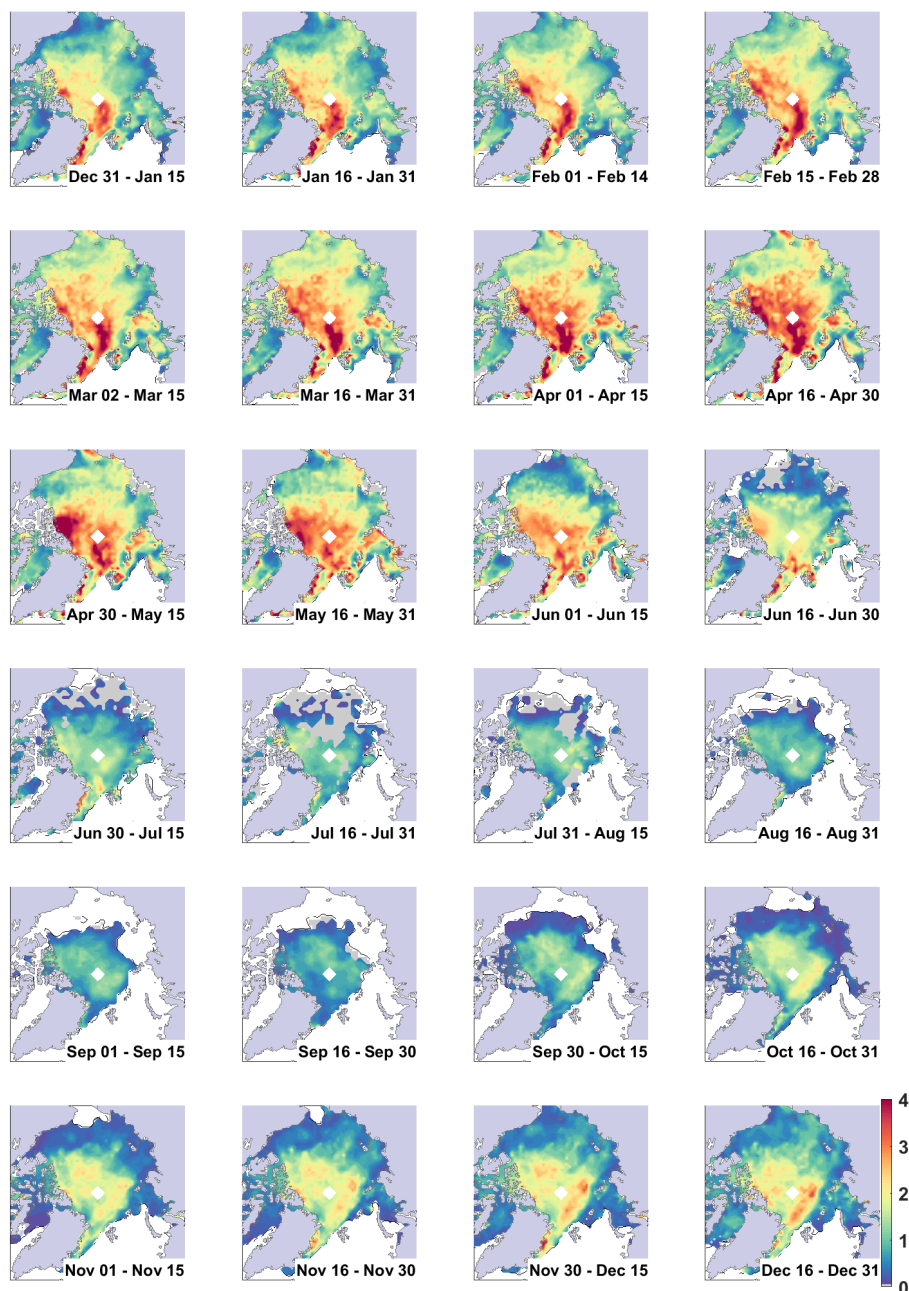
Figure B1. Sea ice thickness across the Arctic for 2015 at twice monthly intervals using the method described in Landy et al. (2022) and the original CNN architecture from Dawson et al. (2022) for the summer (May-September)
