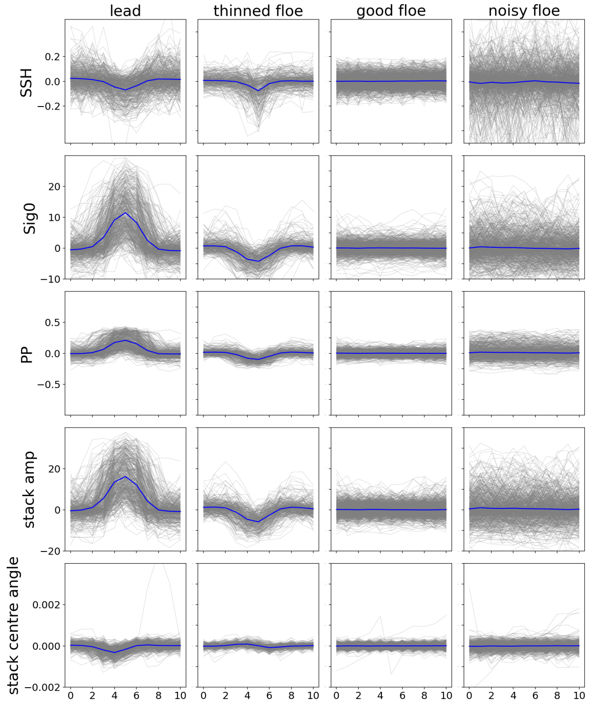
Figure 3. Sea surface height (SSH), backscatter (Sig0), pulse peakiness (PP), stack amplitude (stack amp) and stack centre angle as anomalies (rows) for 11 points along-track sampled around the manually classified point (x-axes) are used as input to the CNN. These variables exhibit unique signatures for the four different classes (columns). The grey lines are the data from the individual samples and the blue line is the average per class.
