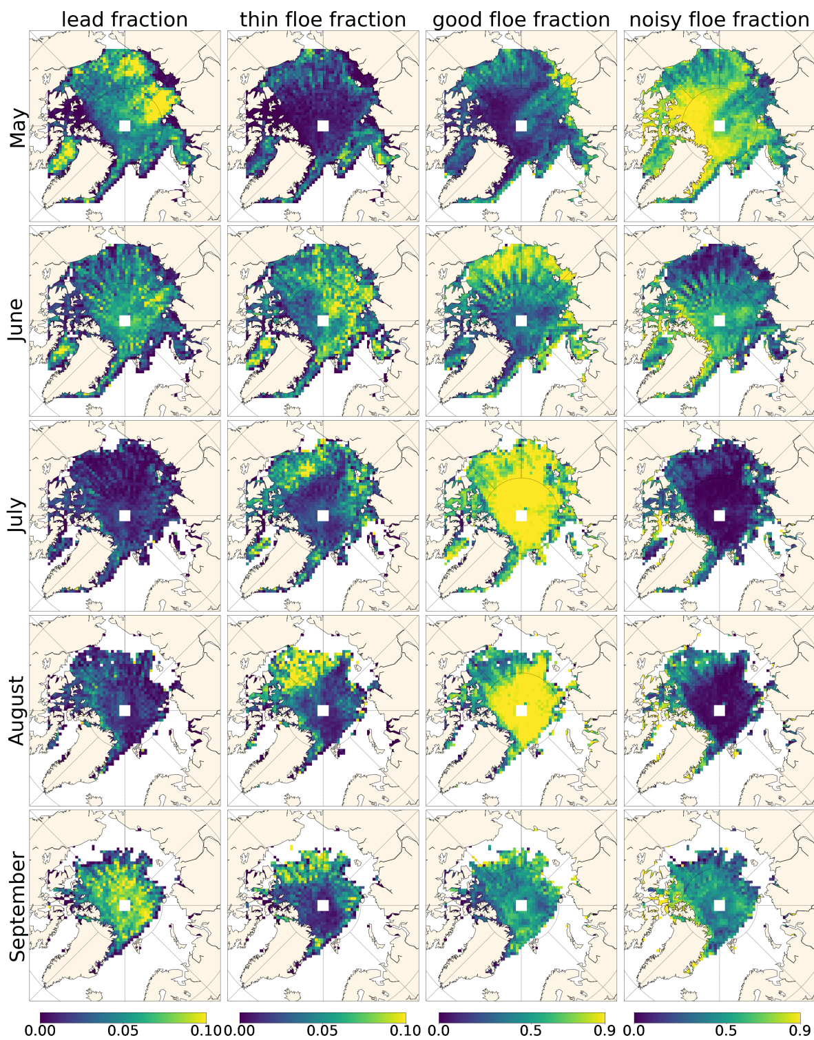
Figure 9. Geographical spread of class fractions (columns) between different months (rows) for 2015
