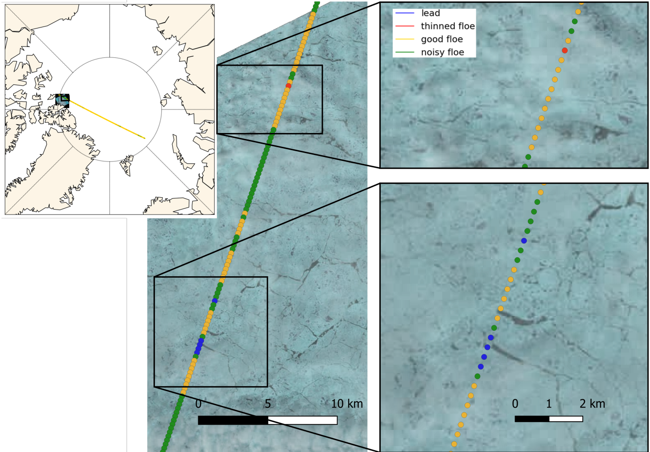
Figure 7. CryoSat-2 track (CS_LTA_SIR_SAR_1B_20180711T201201_20180711T201707_E001) overlain on a Landsat-8 image (LC08_L1GT_068001_20180711_20200831_02_T2_refl) in the Canadian Arctic.
