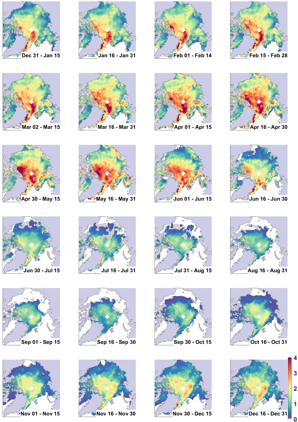
Figure B2. Sea ice thickness [m] across the Arctic for 2015 at twice monthly intervals using the method described in Landy et al. (2022) and the original CNN architecture from Dawson et al. (2022) using more training data for the summer (May-September)
