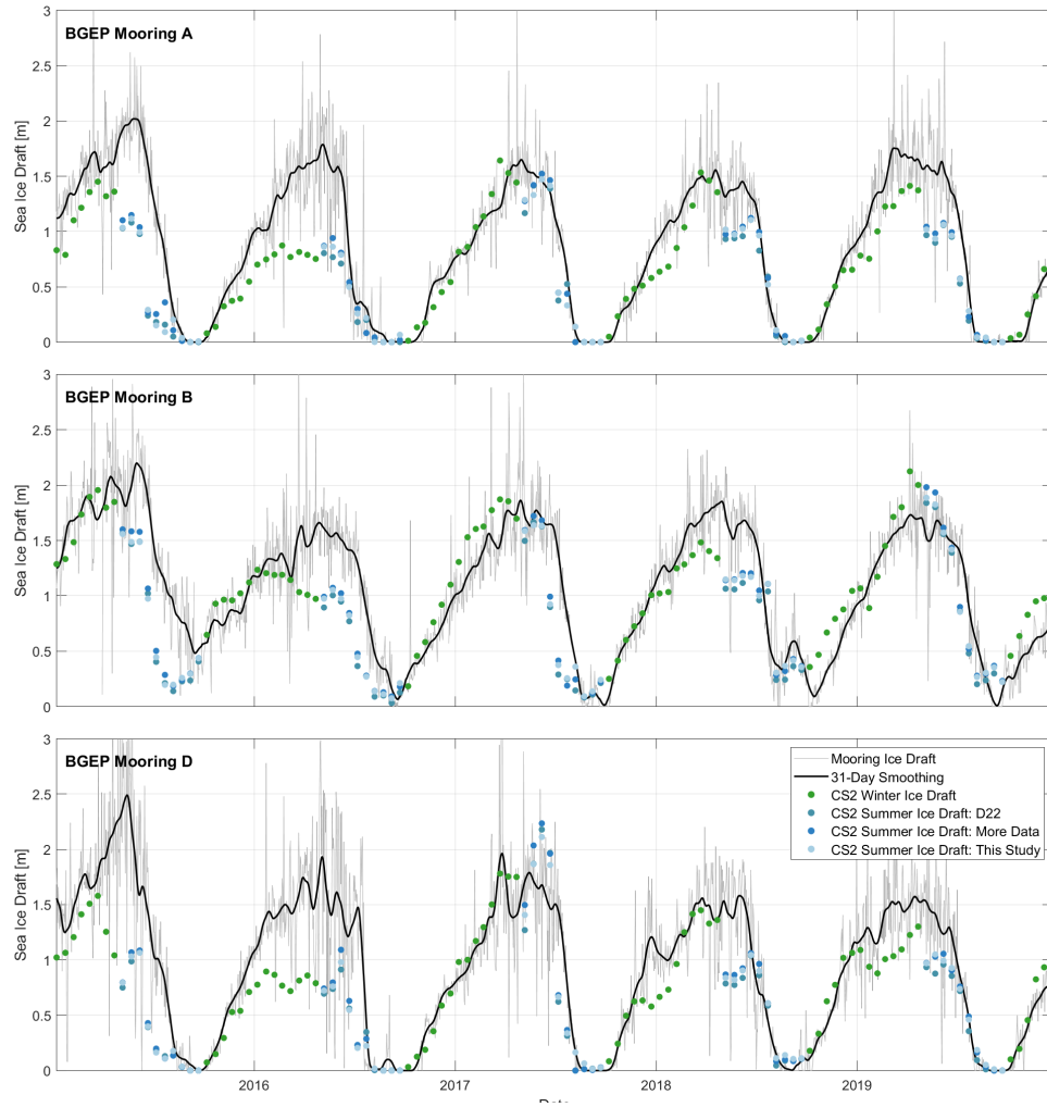
Figure 12. Time series of sea ice draft measured by the BGEF moorings and calculated from CryoSat-2 freeboard observations around the mooring positions. Winter ice draft (green dots) is calculated as described in Landy et al. (2022) and for summer ice draft we plot three versions using the different neural network configurations (blue dots).
