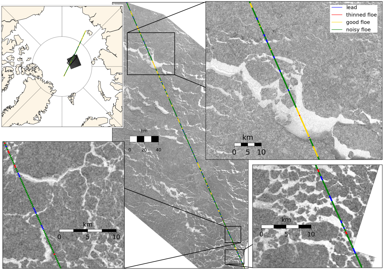
Figure 8. CryoSat-2 track (CS_LTA_SIR_SAR_2_20170924T043410_20170924T043849_E001) overlain on a Sentinel-1 image (S1B_EW_GRDM_1SDH_20170924T043238_20170924T043342_007529_00D4AC_2FDC) in the Central Arctic.
