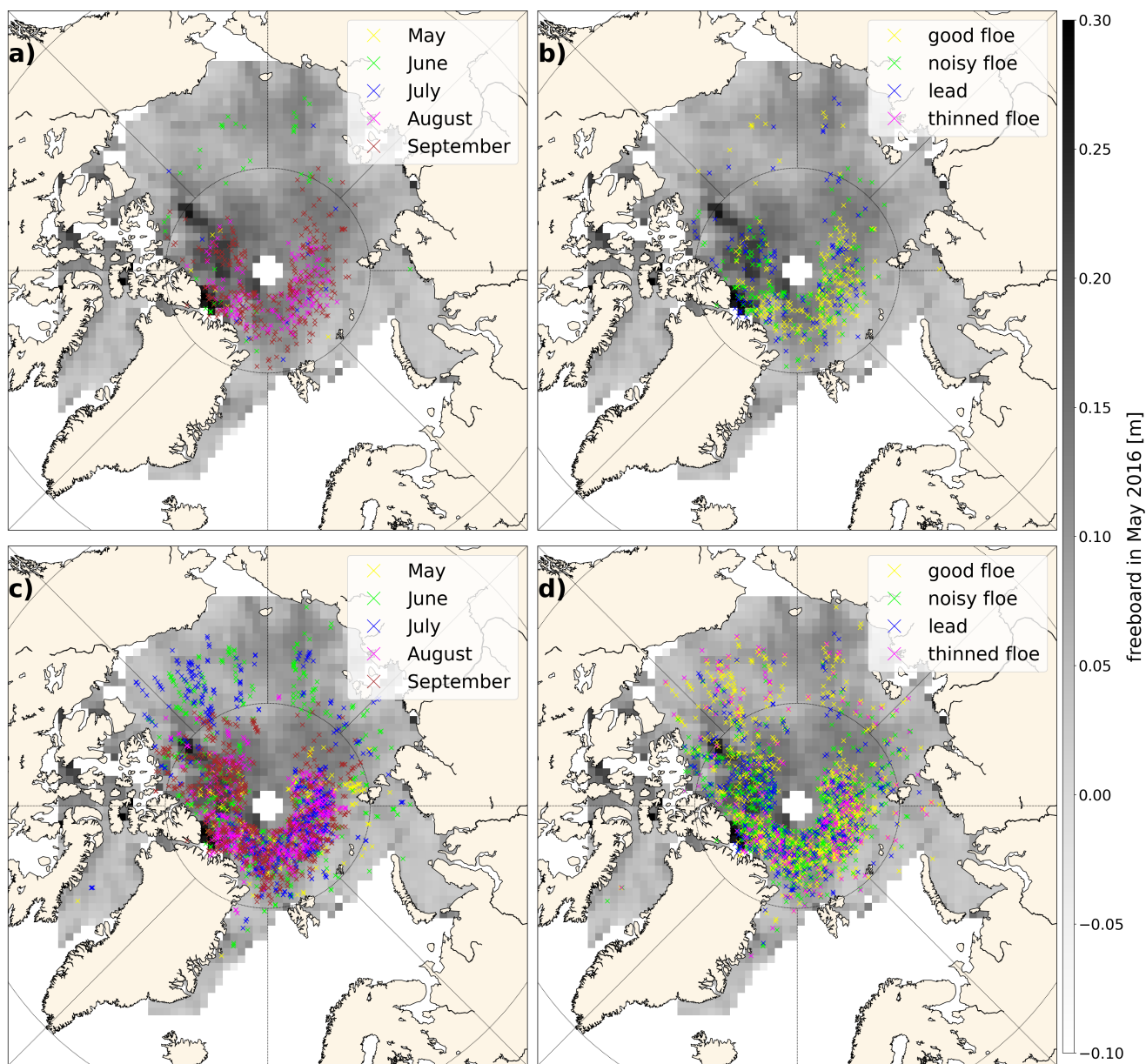
Figure 1. Spatial distribution of samples used in the training data base by Dawson et al. (2022), (subplots a, b) and the extended training database (c, d) divided by month (a, c) and class (b, d) with freeboard from May 2016 in the background
