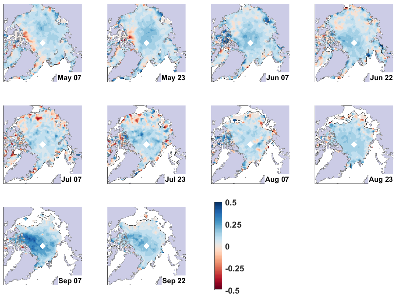
Figure D1. Difference in SIT-sea ice thickness [m] when the original (D22) setup or the novel CNN (this study) are used for classification. Each map represents the average over two weeks across 5 years (2015-2019) labeled with the middle date of each 2 week period.
