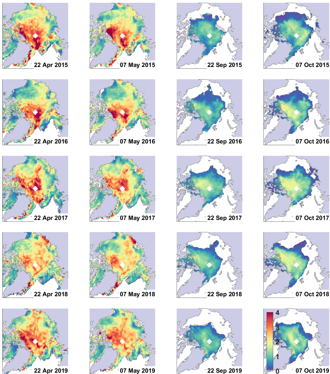
Figure C1. Sea ice thickness [m] across the Arctic at the transition between winter and summer processing during spring (April/May) and autumn (September/October) for five years (2015-2019) using the novel CNN
