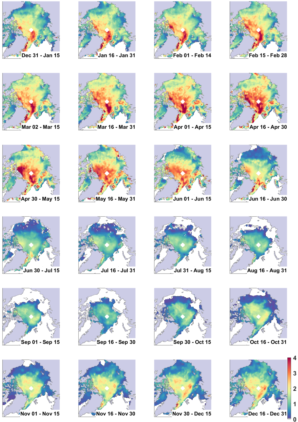
Figure 11. Sea ice thickness [m] across the Arctic for 2015 at twice monthly intervals using the method described in Landy et al. (2022) and the novel CNN architecture for the summer (May-September)
