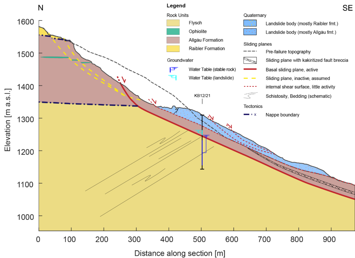
110 Figure 2: Topographic reconstruction of the Igl Rutsch landslide (modified after BTG 2022)
