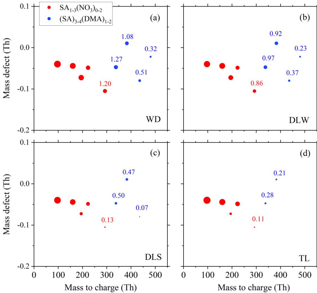
Figure 2: The mass defect of SA molecules and its clusters during four NPF events on (a) January 20 th , 2019 at WD (temperature = 275 K; [SA 1 ] = 1.4 \times 10^7 cm -3 ; CS = 0.055 s -1 ; [DMA] = 3.4 pptv); (b) January 27 th , 2023 at DLW (temperature = 277 K; [SA 1 ] = 7.3 \times 10^6 cm -3 ; CS = 0.012 s -1 ; [DMA] = 1.5 pptv); (c) May 2 nd , 2023 at DLS (temperature = 295 K; [SA 1 ] = 9.5 \times 10^6 cm -3 ; CS = 0.014 s -1 ; [DMA] = 2.9 pptv); (d) August 7 th , 2023 at TL (temperature = 304 K; [SA 1 ] = 2.6 \times 10^7 cm -3 ; CS = 0.023 s -1 ; [DMA] = 1.8 pptv). Other species detected by CI-LToF-MS were not shown, because they are not expected to participate in directly-related-to-atmospheric nucleation . The area of symbol is proportional to the logarithm of normalized signal. (multiplied by a factor of 1 \times 10^6 before taking the logarithm). The logarithm of values is annotated for some larger clusters.
