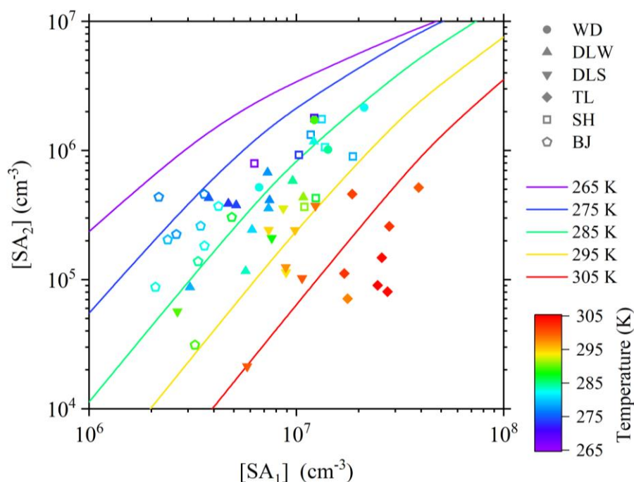
Figure 5: [\text{SA}_2]_{\text{scaled}} as a function of [\text{SA}_1] under a temperature gradient. Each symbol indicates one NPF event with a time resolution of 30 min, which was selected when J_{1.7,\text{meas}} reaches maximum. [\text{DMA}] and CS for the simulated lines calculated by the discrete-sectional model are their median values in all NPF events, i.e., 0.017 \text{ s}^{-1} and 2.3 pptv, respectively. To visualize the effect of temperature, the color of the simulated lines corresponds to the color bar.
