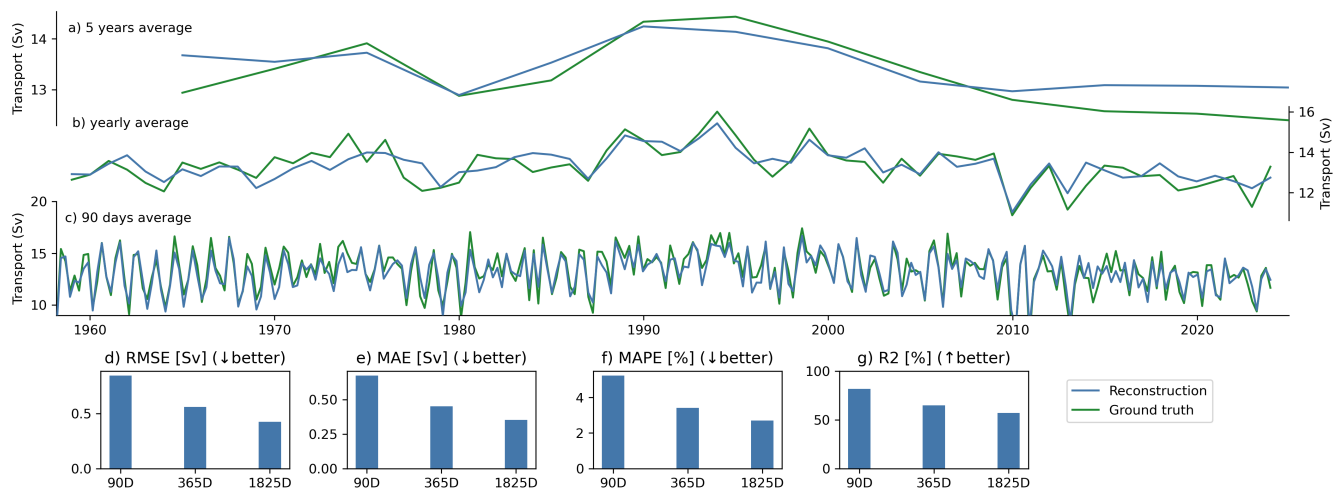
Figure 6. Reconstruction (blue) on five-yearly a), yearly b), and seasonal c) time scales with the AMOC of the third OMIP (orangegreen) cycle as test period, validation period of 20 years were attached previous and after the test period, the rest of the six cycles was used for the training of the reconstruction.
