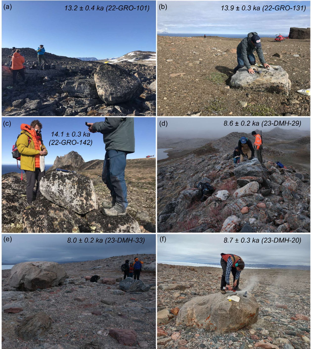
Figure 2. Representative boulder sample sites from outer Scoresby Sund (a, b, c), and the unnamed island near the terminus of Storstrømmen Glacier (d, e, f). (a) Sample 22-GRO-101, Uunarteq at the northern mouth of Scoresby Sund. (b) Sample 22GRO-131, Kap Brewster (Kangikajjip Appalia) at the southern mouth of Scoresby Sund. (c) Sample 22GRO-142, Rathbone Island, ~3 km to the east of the main coastline of Liverpool Land. (d) Sample 23DMH-29, from the prominent M1 moraine on the island at the terminus
