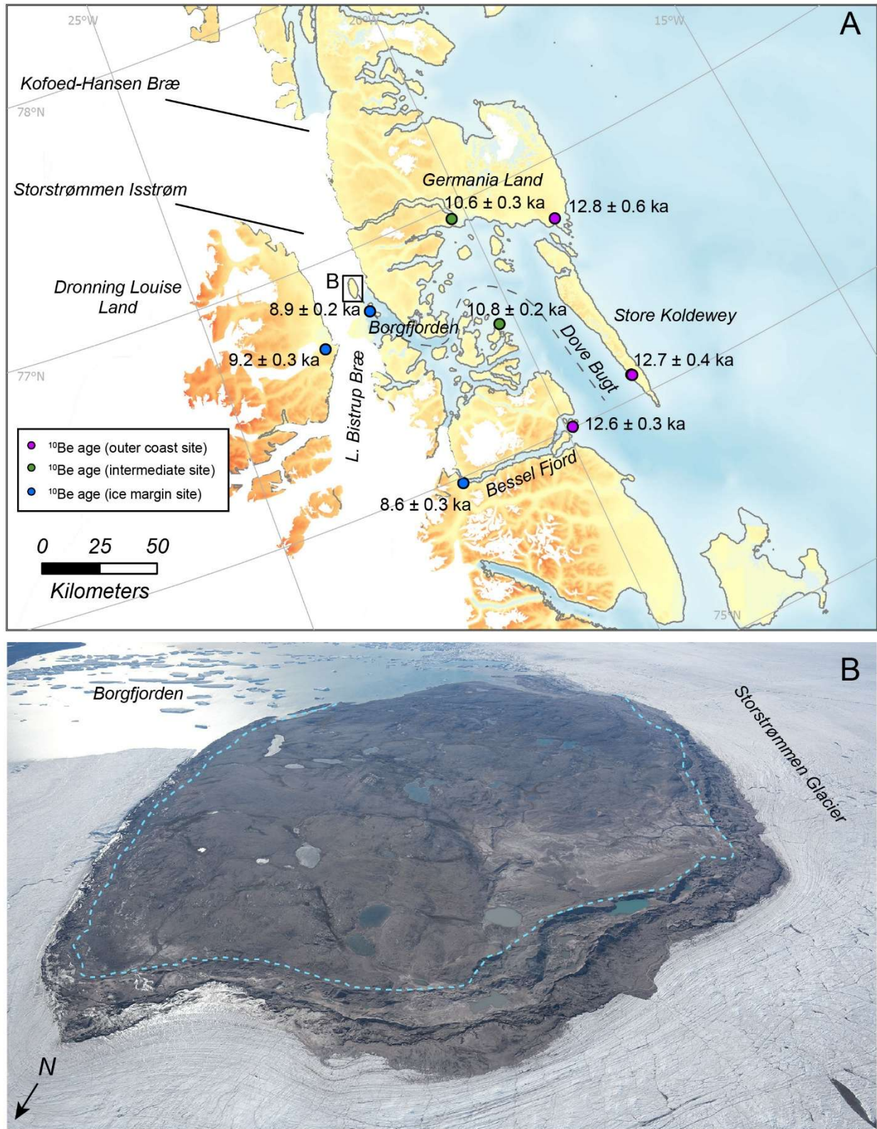
Figure 4. (A) Dove Bugt region showing outer coast (purple), intermediate (green) and ice margin (blue) exposure ages from Larsen et al. (2022). The outer coast mean ages are 12.8 ka (n = 1), 12.7 ka (n = 3),
