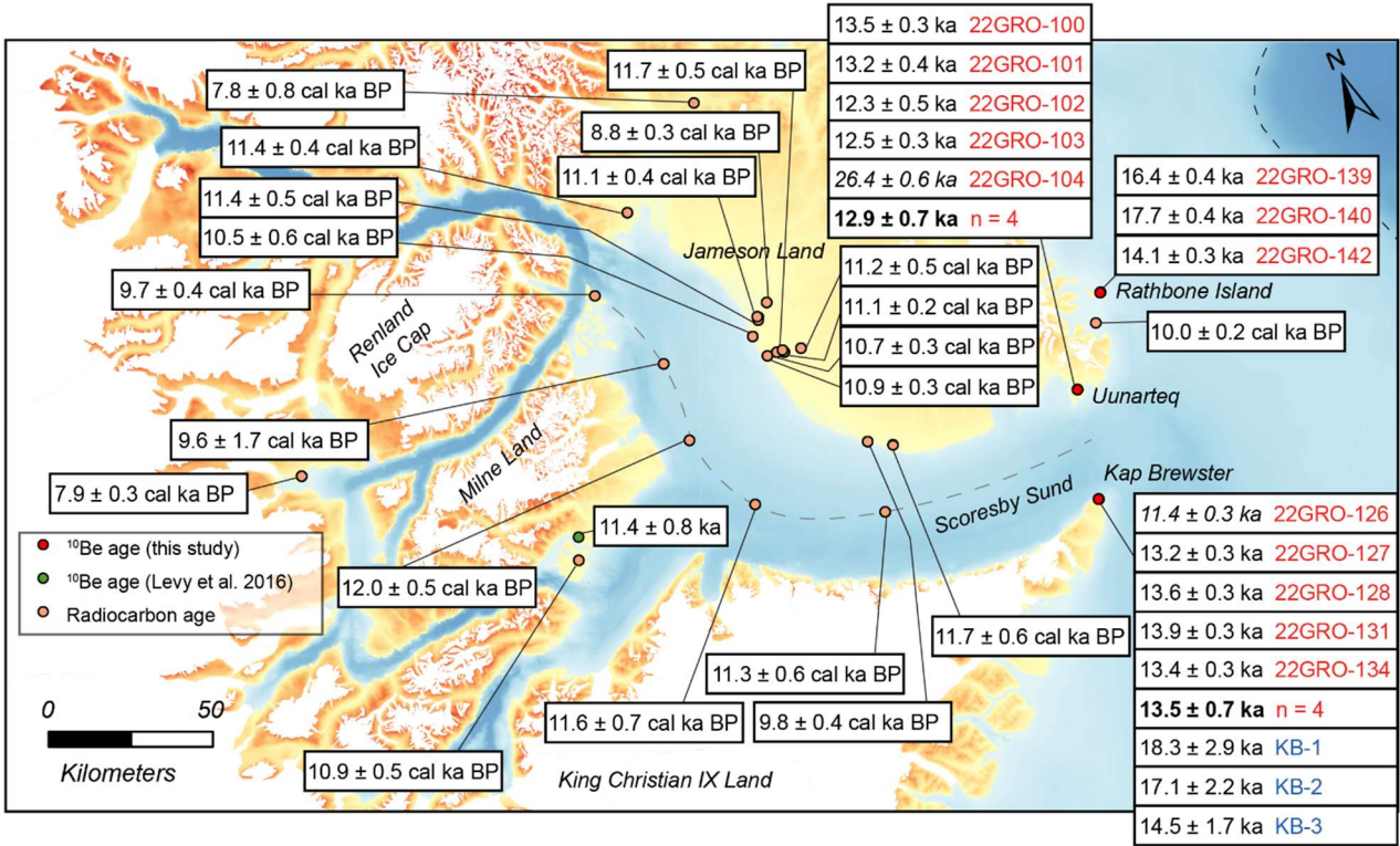
Figure 3. (A) Scoresby Sund with new measured ^{10}\text{Be} ages of boulders (red circles) with red sample names, and recalculated ^{10}\text{Be} ages of Håkansson et al. (2007a) with blue sample names at Kap Brewster. All ^{10}\text{Be} ages shown in kiloyears with 1\sigma internal uncertainties. Mean ^{10}\text{Be} ages from Uunarteq and Kap Brewster are shown in bold. Mean ^{10}\text{Be} age ( n = 8 ; green circle) from Milne Land (Levy et al., 2016). Radiocarbon ages (orange circles) are listed in Table 1. ^{10}\text{Be} age outliers shown in italics. The grey dashed line denotes the flowline and ^{10}\text{Be} and radiocarbon ages used to calculate average retreat rates. The maximum LGM extent is marked by the black dashed line, derived from Leger et al. (2024 and references therein). (B) East Scoresby Sund region showing the timing of ice margin retreat at the mouth of Scoresby Sund. The extent of the Kap Brewster submarine moraine is from Funder and Hansen (1996).
