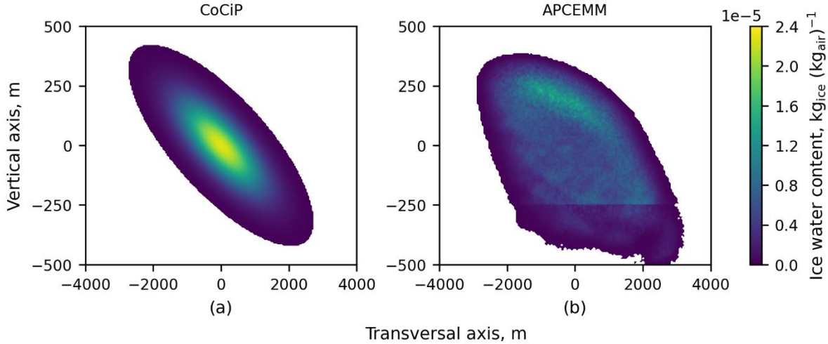
Figure 2: Cross-sectional distribution of the ice water content (IWC) for the CoCiP plume (a), and APCEMM plume (b) \sim 1 h 30m after formation. Both simulations use the same synthetic meteorological conditions. The origin of each panel represents the approximate visual center of the contrail, at a pressure altitude of 9927 m in CoCiP and 9750 m in APCEMM. The cruise altitude is 10000 m.
