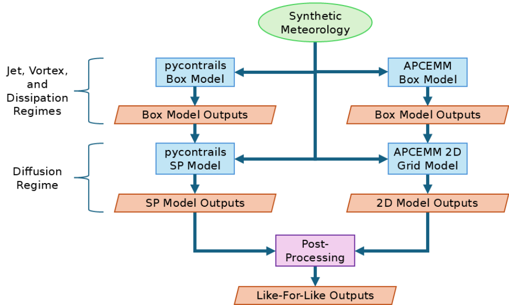
135 Figure 3: Flow chart showing the experimental simulation process for both CoCiP and APCEMM. Green ellipses indicate inputs, blue rectangles indicate plume models, orange rhombi indicate outputs, and purple rectangles indicate data processing units.
