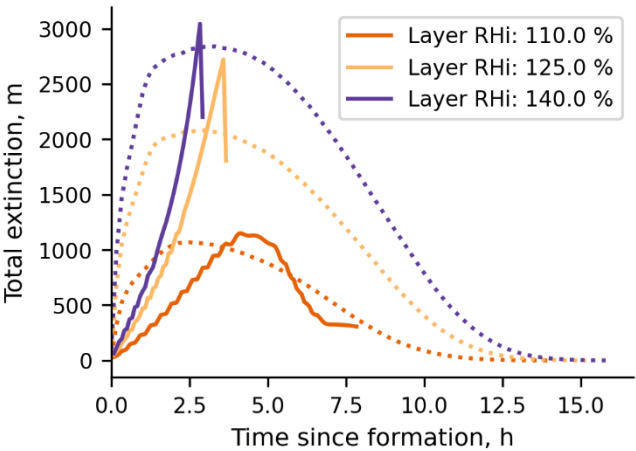
Figure 8: Total extinction ( E ) against time for the contrails produced at varying layer RHIs. The CoCiP and APCEMM simulations are represented by solid and dotted lines respectively.
