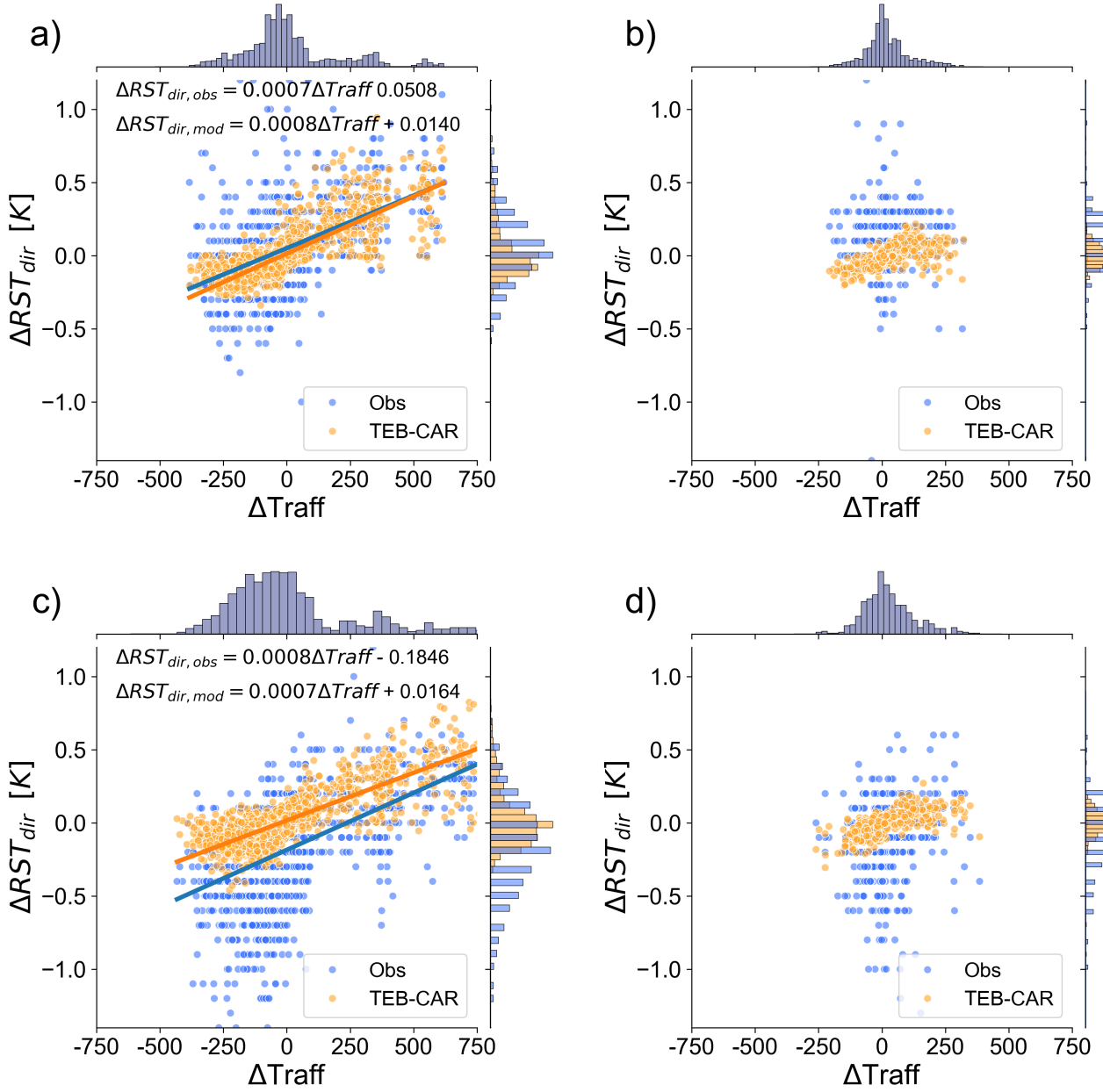
Figure 6. Simulated and observed Road surface temperature differences \Delta RST_{dir} of road surface temperatures \Delta T_s both measured and simulated values between the Helsinki direction and Turku Direction directions (H-T Helsinki minus Turku), with robust Robust linear regression lines (RLM) are drawn between \Delta Traffic and \Delta T_s \Delta RST_{dir} for both observations and simulations. Panels (a) and (b) show the differences at the Palojärvi site on weekdays (a) and week-ends weekends (b), respectively. Panels (c) and (d) show the same information at the Nupuri site.
