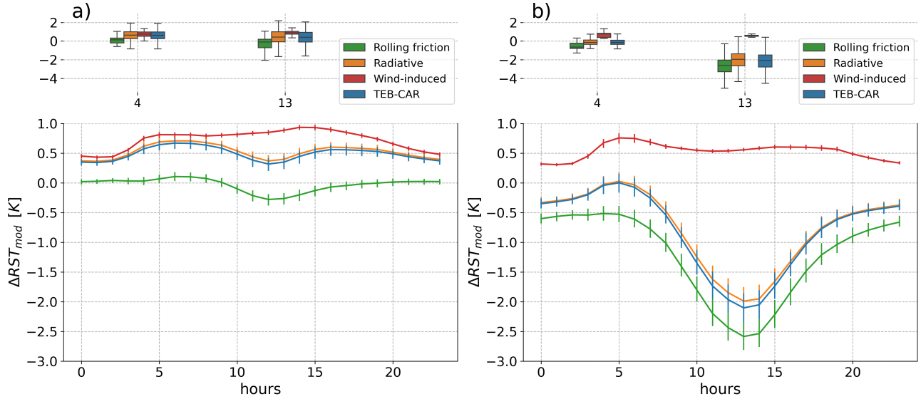
Figure 8. Ablation study of On the processes implemented in the TEB-CAR with one process removed at each simulation and the reference. Road Helsinki road direction, road surface temperature differences \Delta RST_{mod} between TEB-CAR, the ablation experiment simulations with TEB ( \Delta T_s TEB-CAR minus TEB) with the boxplots at. Boxplots are drawn in peak traffic intensity (4:00 h UTC and 13:00 h UTC) between on the simulations upper panels and lines of the observations average hourly values on the bottom panels. \Delta RST_{mod} are calculated for the winter period in (a) and spring in (b) with the confidence interval of the estimator of the expected value.
