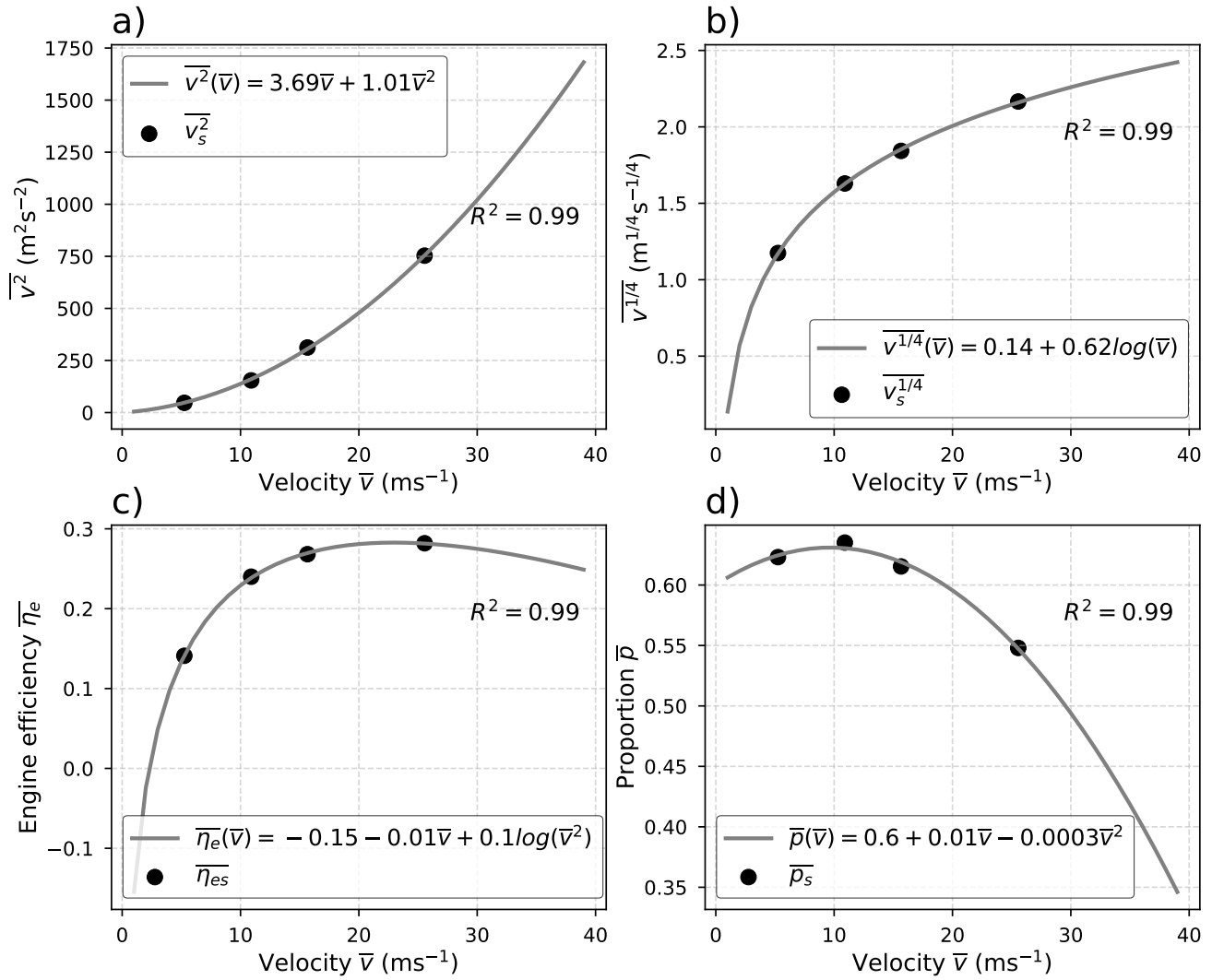
Figure B1. Regression equations from the multiple linear regressions (MLRs) of the parameters against the local estimate for each WLTC cycle with the average: (a) squared speed v_s^2 , (b) speed to the power 1/4, (c) engine efficiency, (d) acceleration proportion
