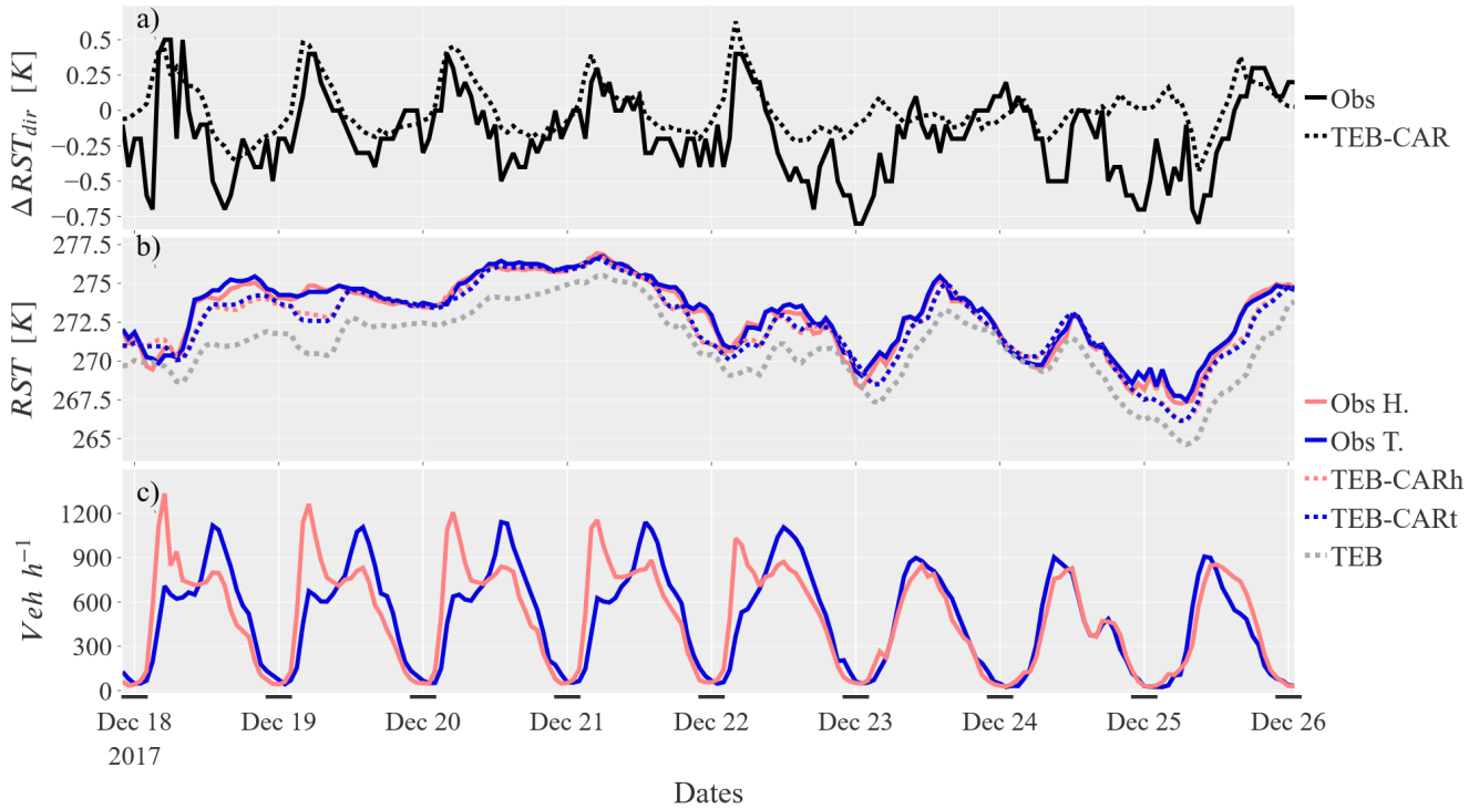
Figure 5. Comparison between TEB and TEB-CAR model version simulations (TEB-CARh for the simulation toward Helsinki-observed and TEB-CARt for the simulation toward Turku)-simulated RST on a 8-days-eight days subset period from beginning a monday to tuesday one-week-later-with-the-observations-measured at Nupuri location. The subscripts "h" and "t" are for values on Helsinki and Turku directions respectively. From top to bottom panel : (a) observed and modelled road surface temperature difference between the two road directions ( \Delta RST_{dir} ) (Helsinki minus Turku), (b) road surface temperature, (c) number of vehicles per hour
