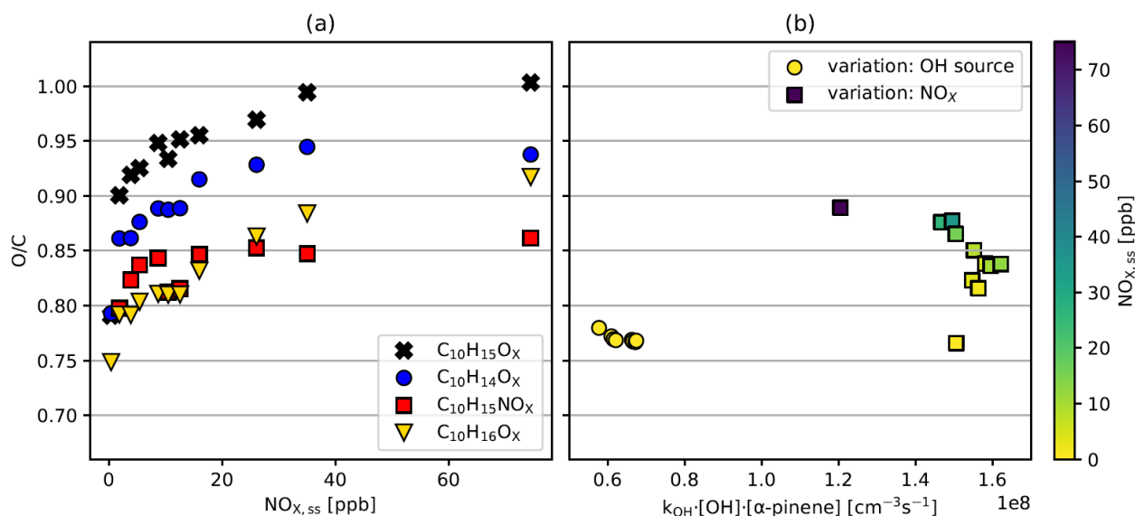
Figure 7: (a) Averaged O:C ratio of the HOM families as a function of [NO x ] ss in the NO x experiments. (b) Overall O/C as a function of turnover for C 10 monomer compounds in the reference experiments (circles) and the NO x experiments series (squares). The color scale represents the level of steady-state concentration [NO x ] ss in the chamber.
