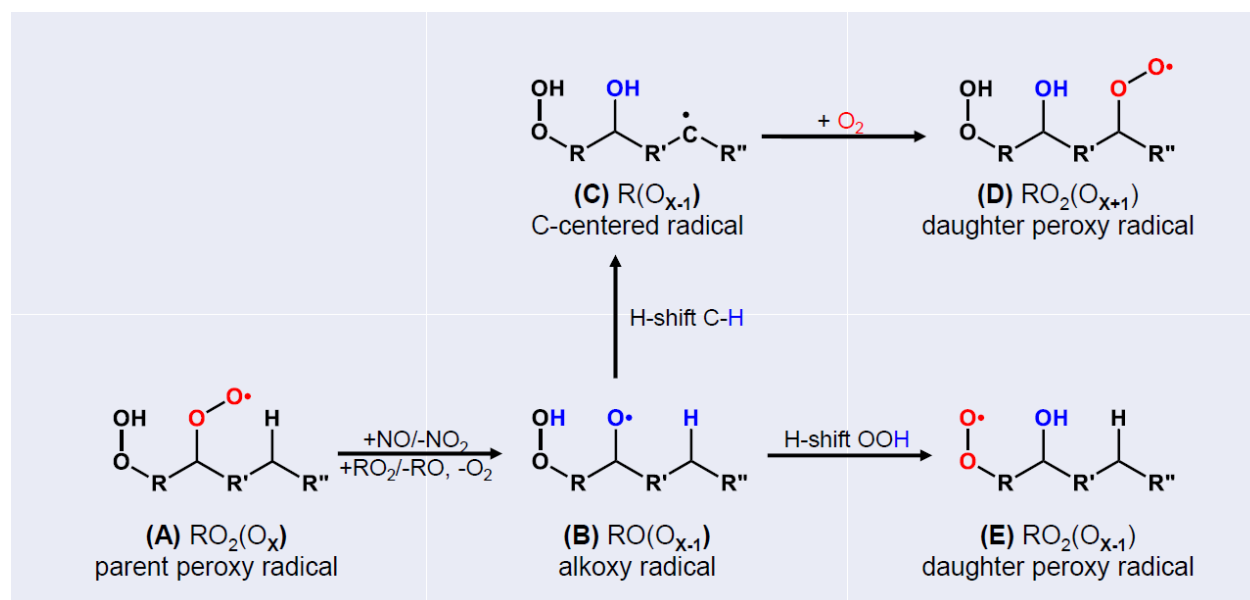
Figure 1: Schematic sketch of the alkoxy-peroxy pathways ABCD and ABE, considering fast isomerization of the alkoxy radical (B) by H-shift from a C-H bond, or by H-shift from a HO_2 group. The resulting peroxy radicals D, E have one more or one less oxygen atom compared to the parent peroxy radical (A); thus, the parity of the oxygen number is changed.
