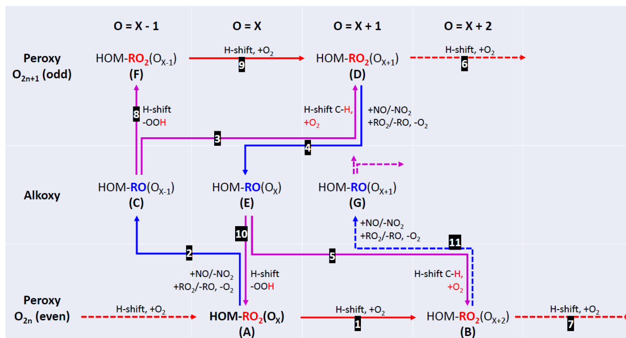
Figure 8: Scheme of alkoxy-peroxy pathways. Red arrows indicate autoxidation of peroxy radicals, blue arrows indicate formation of alkoxy radicals in reactions of the peroxy radicals with other RO 2 or with NO, and lilac arrows indicate isomerization of alkoxy radicals with subsequent O 2 addition, where it applies.
