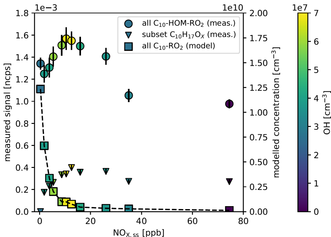
Figure 6: Comparison of the dependence on [NO x ] ss for observed C 10 -HOM-RO 2 • signal (spheres, left axis) and for modelled concentration of conventional C 10 -RO 2 • (squares, right axis), which is a fraction of the peroxy radical sum termed “RO 2 ” in MCMv3.1.2. The color code indicates the actual [OH • ] ss with a maximum of 6.9·10 7 cm -3 at about 15 ppb [NO x ] ss . While the concentration of conventional, less oxygenated C 10 -RO 2 • drops quickly with [NO x ] ss because of the strong sink provided by reaction with NO, the [C 10 -HOM-RO 2 • ] remains at a significant level even at the highest [NO x ] ss . The triangles show the signal of the subset of C 10 H 17 O x HOM-peroxy radicals (left axis) which remain also high at high [NO x ] ss . Errors for the experimental data are calculated by error propagation based on the standard deviations for averaging over the steady state intervals.
