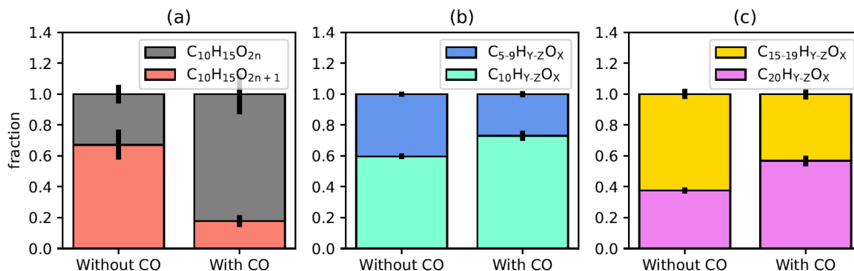
Figure 4: Impact of enhanced [HO_2]_{ss} on oxygen parity of C_{10}H_{15}O_x radicals and on fragmented products. (a) The fraction of C_{10}H_{15}O_{2n} (black) and C_{10}H_{15}O_{2n+1} (red) for the cases without and with CO addition. (b) Fraction of fragmented monomers ( C_{5-9} , blue) and C_{10} monomers (mint). (c) Fraction of fragmented accretion products (yellow) and C_{20} accretion products (magenta). Error bars are calculated by error propagation based on the standard deviations for averaging over the steady state intervals.
