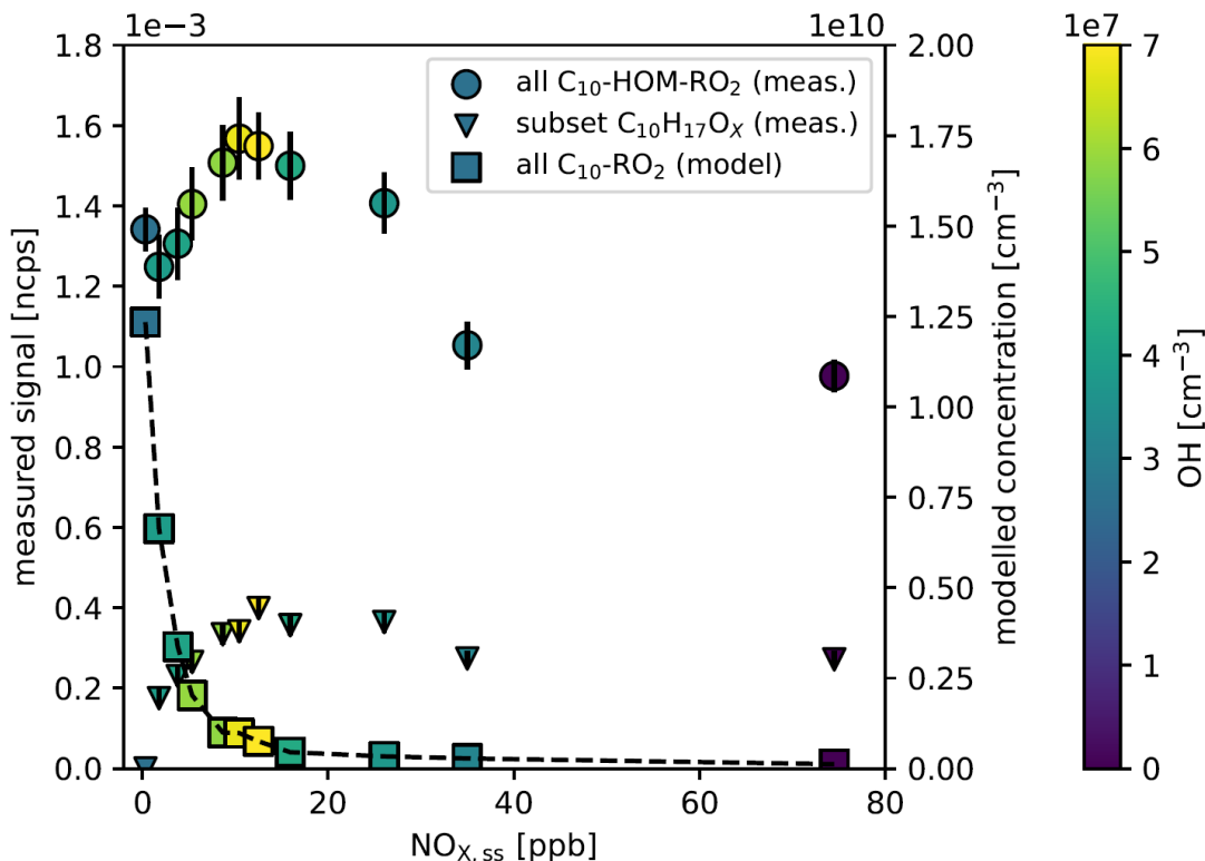
600 Figure 6: Comparison of the dependence on [\text{NO}_\text{x}]_{\text{ss}} for observed \text{C}_{10}\text{-HOM-RO}_2^\cdot signal (spheres, left axis) and for modelled concentration of conventional \text{C}_{10}\text{-RO}_2^\cdot (squares, right axis), which is a fraction of the peroxy radical sum termed “ \text{RO}_2 ” in MCMv3.1.2. The color code indicates the actual [\text{OH}^\cdot]_{\text{ss}} with a maximum of 6.9 \cdot 10^7 \text{ cm}^{-3} at about 15 ppb [\text{NO}_\text{x}]_{\text{ss}} . While the concentration of conventional, less oxygenated \text{C}_{10}\text{-RO}_2^\cdot drops quickly with [\text{NO}_\text{x}]_{\text{ss}} because of the strong sink provided by reaction with \text{NO} , the [\text{C}_{10}\text{-HOM-RO}_2^\cdot] remains at a significant level even at the highest [\text{NO}_\text{x}]_{\text{ss}} . The triangles show the signal of the subset of \text{C}_{10}\text{H}_{17}\text{O}_\text{x} HOM-peroxy radicals (left axis) which remain also high at high [\text{NO}_\text{x}]_{\text{ss}} . Errors for the experimental data are calculated by error propagation based on the standard deviations for averaging over the steady state intervals.
