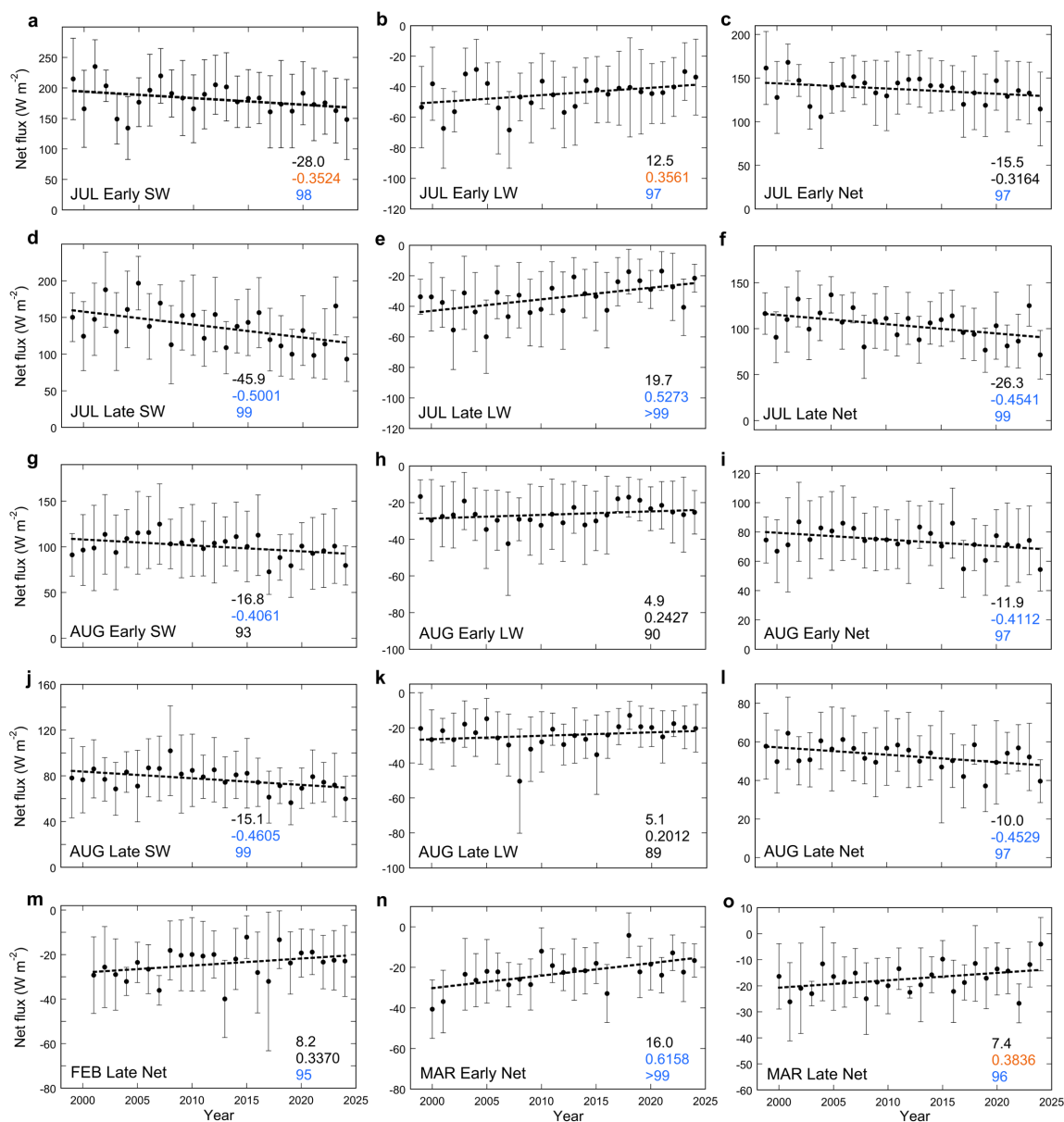
170 Figure 2. Time series of the semi-monthly interval-average net radiative flux components (shortwave SW and longwave LW) and their sum (Net); for the four intervals in July and August (panels a-l), and for net radiative flux in three other intervals that show some degree of statistical significance in the trend from 1999-2024 (panels m-o). The mean value in each interval is shown as a dot and the error bars are plus and minus one standard deviation about the mean. The linear least-squares trend is shown as a dotted line. The three numbers in each panel are the linear change in the radiative flux between 1999-2024 (top), the Pearson correlation 175 coefficient from ordinary least squares (middle) and the percent confidence level in trend detection from a Mann-Kendall test (bottom). For the latter two numbers, values having statistical significance of 95% or greater are shown in blue, values with one- tailed confidence (90-95%) are shown in orange, and values with less statistical confidence are left in black.
