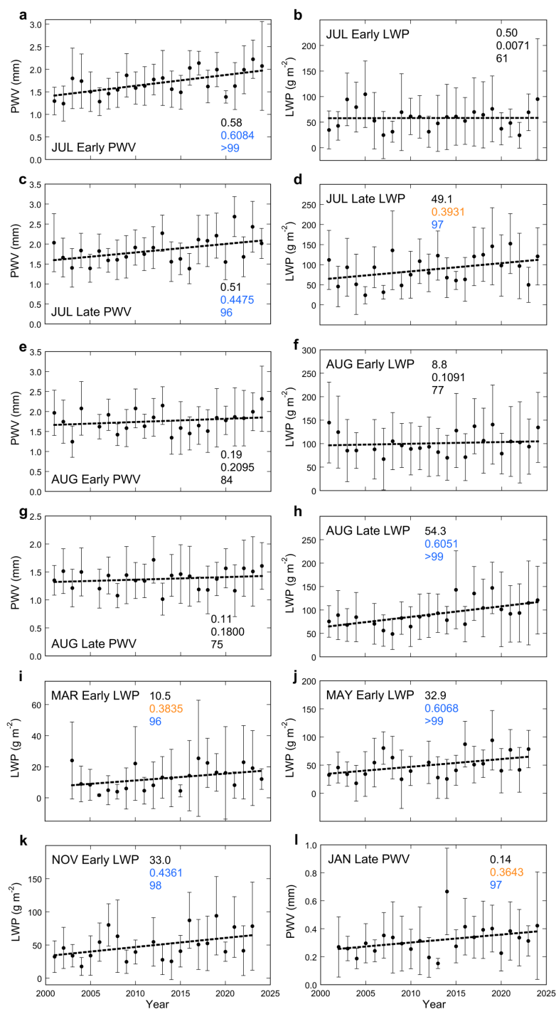
240 Figure 4. Time series of the semi-monthly interval-average microwave radiometer-derived precipitable water vapor (PWV) and cloud liquid water path (LWP) for the four intervals in July and August (panels a-h), and for four other intervals that show some degree of statistical significance in the trend from 2001-2024 (panels i-l). Symbols and numbers on each panel are as in Figure 2.
