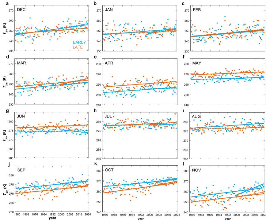
165 Figure 1. Trends in the semi-monthly interval-averaged 2 m near-surface air temperature at the NSA site from ERA5 data, organized by month (panels a-l) and semi-monthly intervals (light blue for the first two weeks, orange for the second). For each interval two linear trend lines are shown, one for the full time series (1959-2024) and one for the period overlapping the NSA data (1999-2024). Trends that are statistically significant with two-tailed confidence are shown as solid lines, while trends with less statistical significance are shown as dotted lines.
