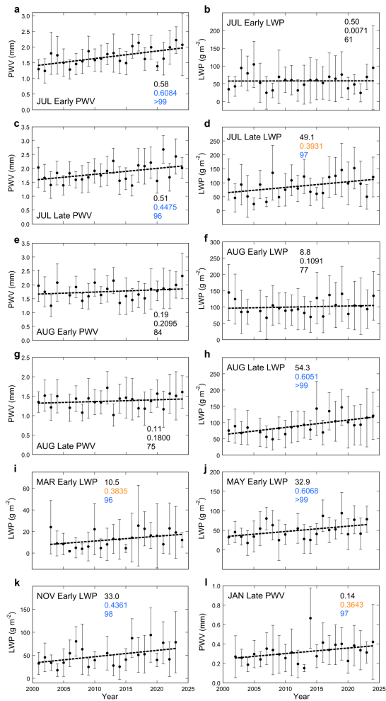
260 Figure 4. Time series of the semi-monthly interval-average microwave radiometer-derived precipitable water vapor (PWV) and cloud liquid water path (LWP) for the four intervals in July and August (panels a-h), and for four other intervals that show some degree of statistical significance in the trend from 2001-2024 (panels i-l). Symbols and numbers on each panel are as in Figure 2.
